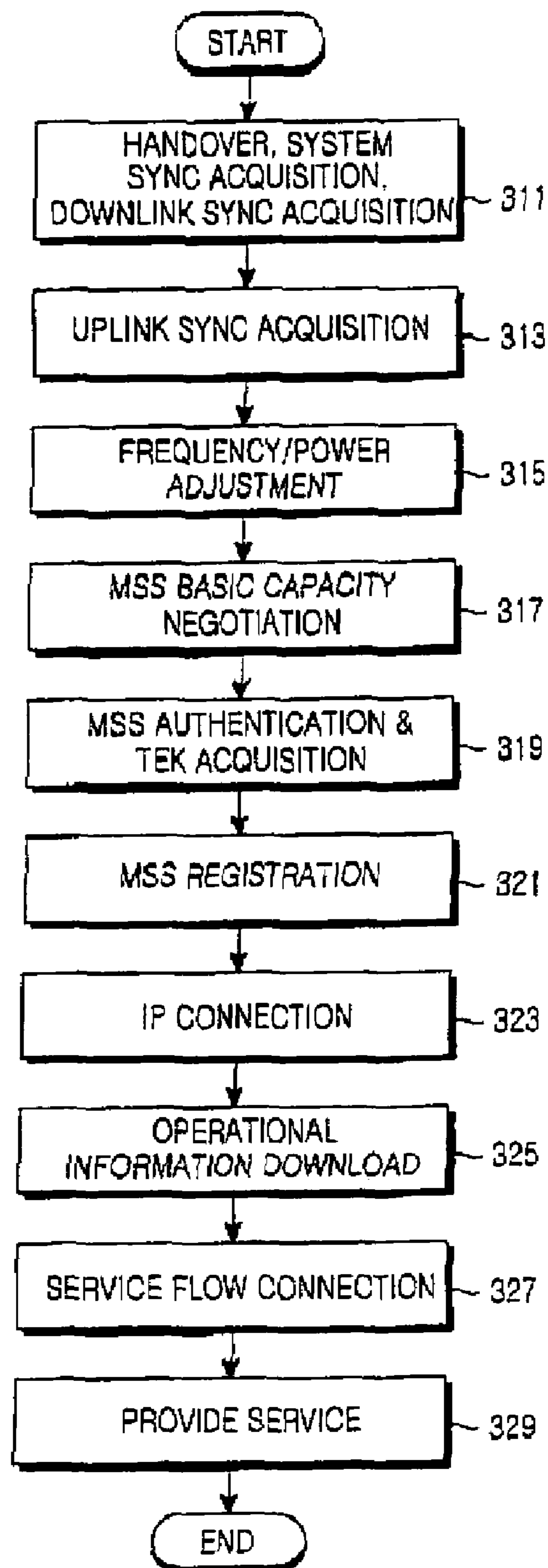
FIG. 3 (PRIOR ART)
