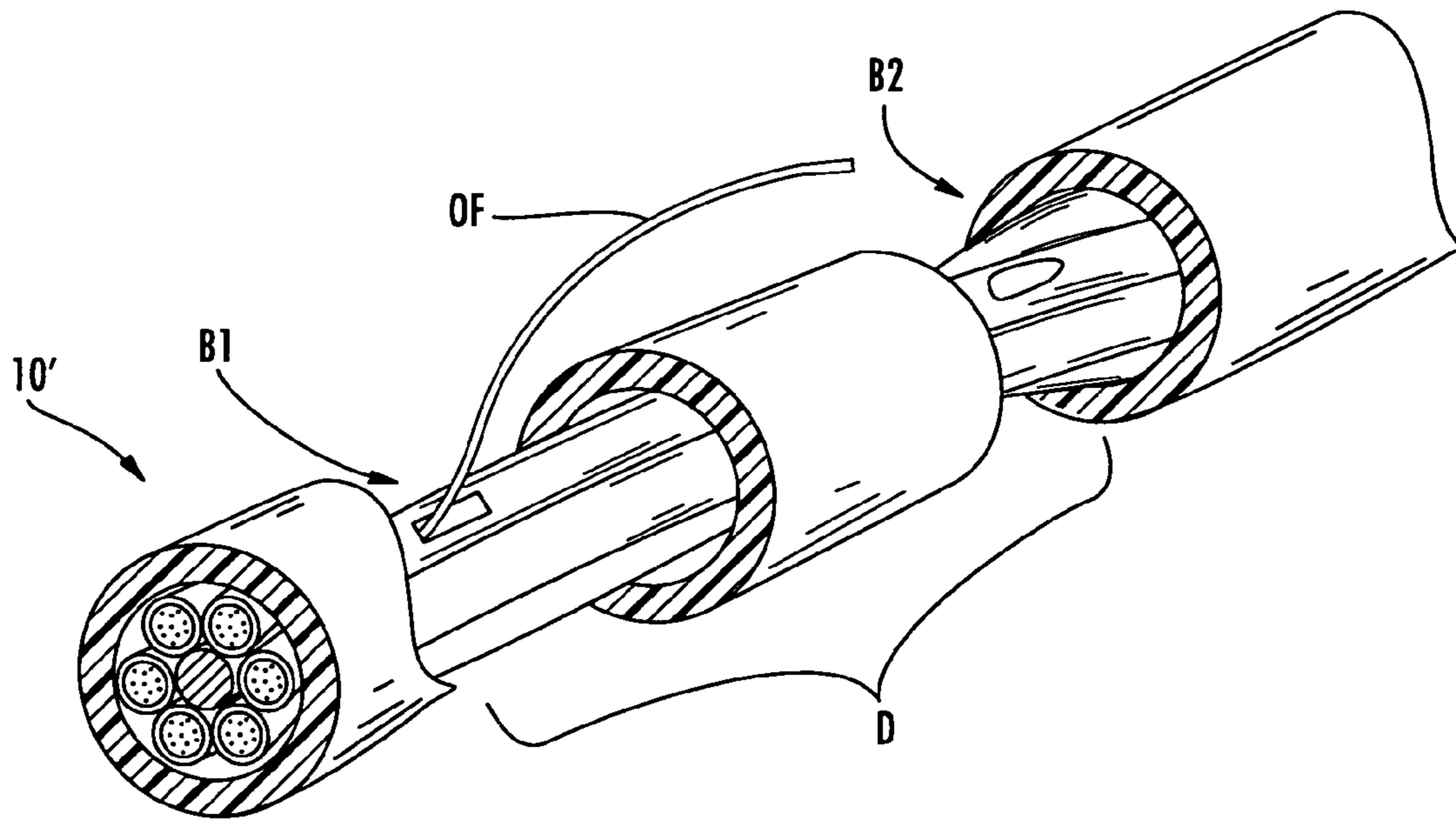
FIG. 2 (PRIOR ART)
