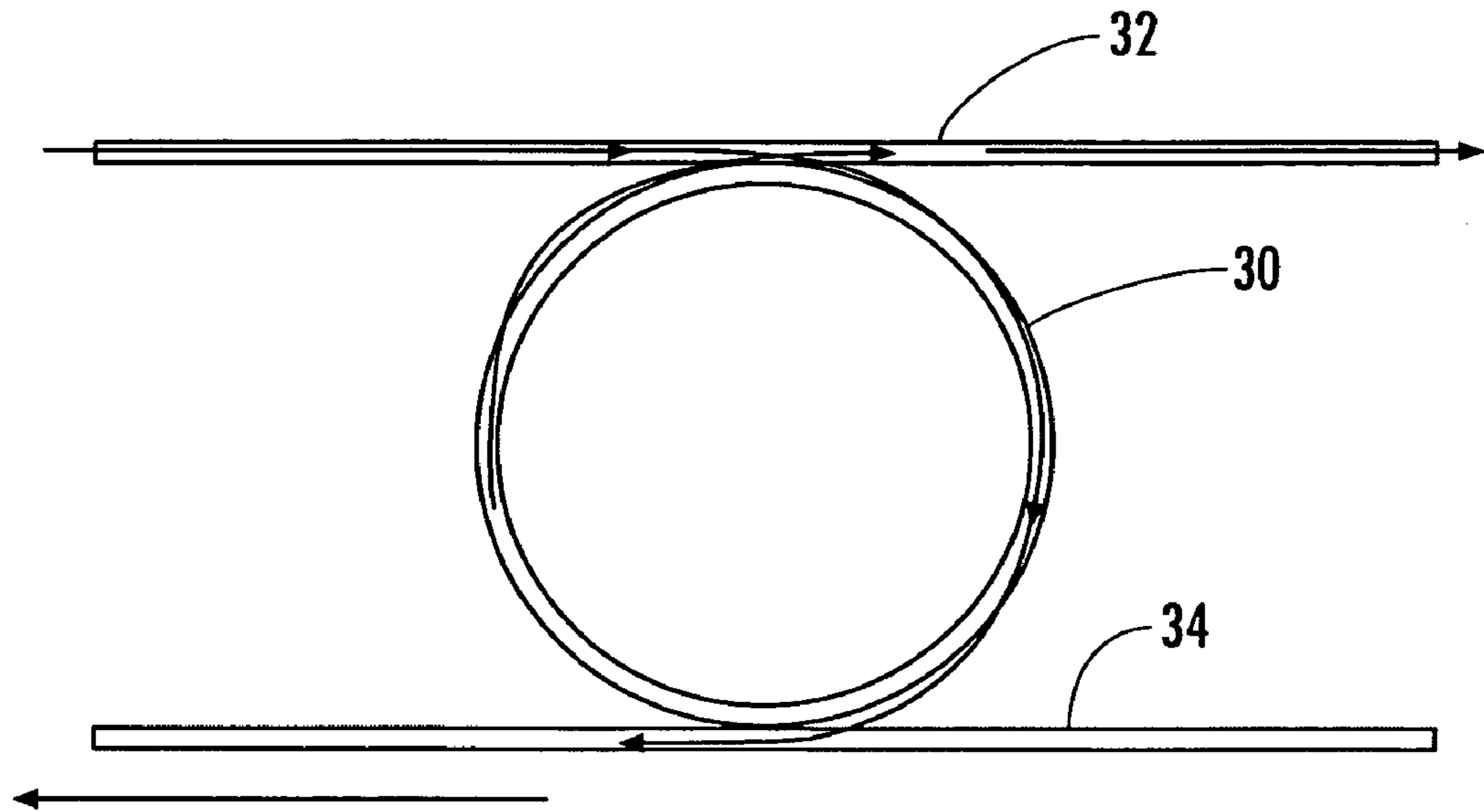
FOUR-PORT RESONANT STRUCTURE
