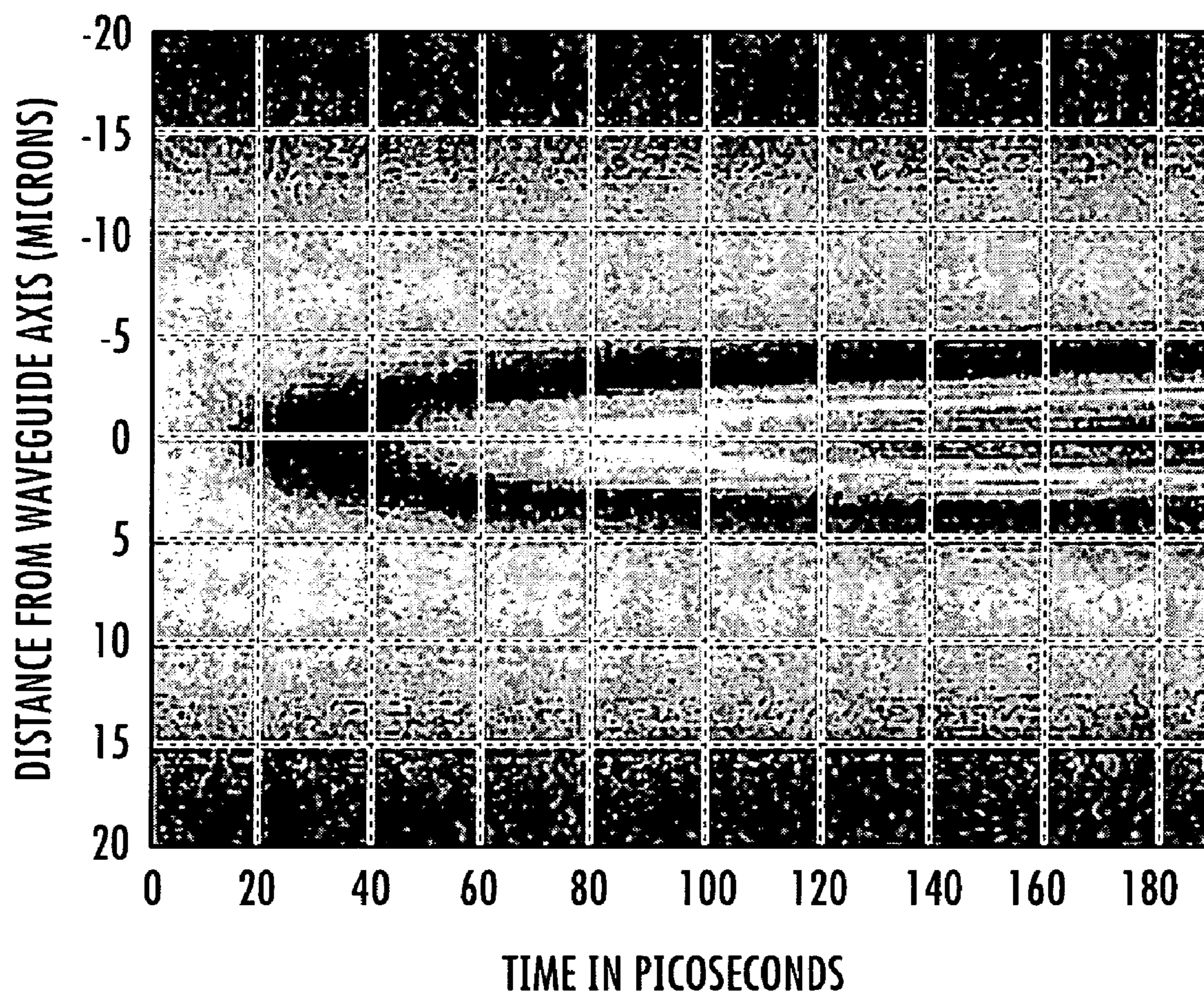
TRANSIENT FIELD PATTERNS IN SOURCE GUIDE
