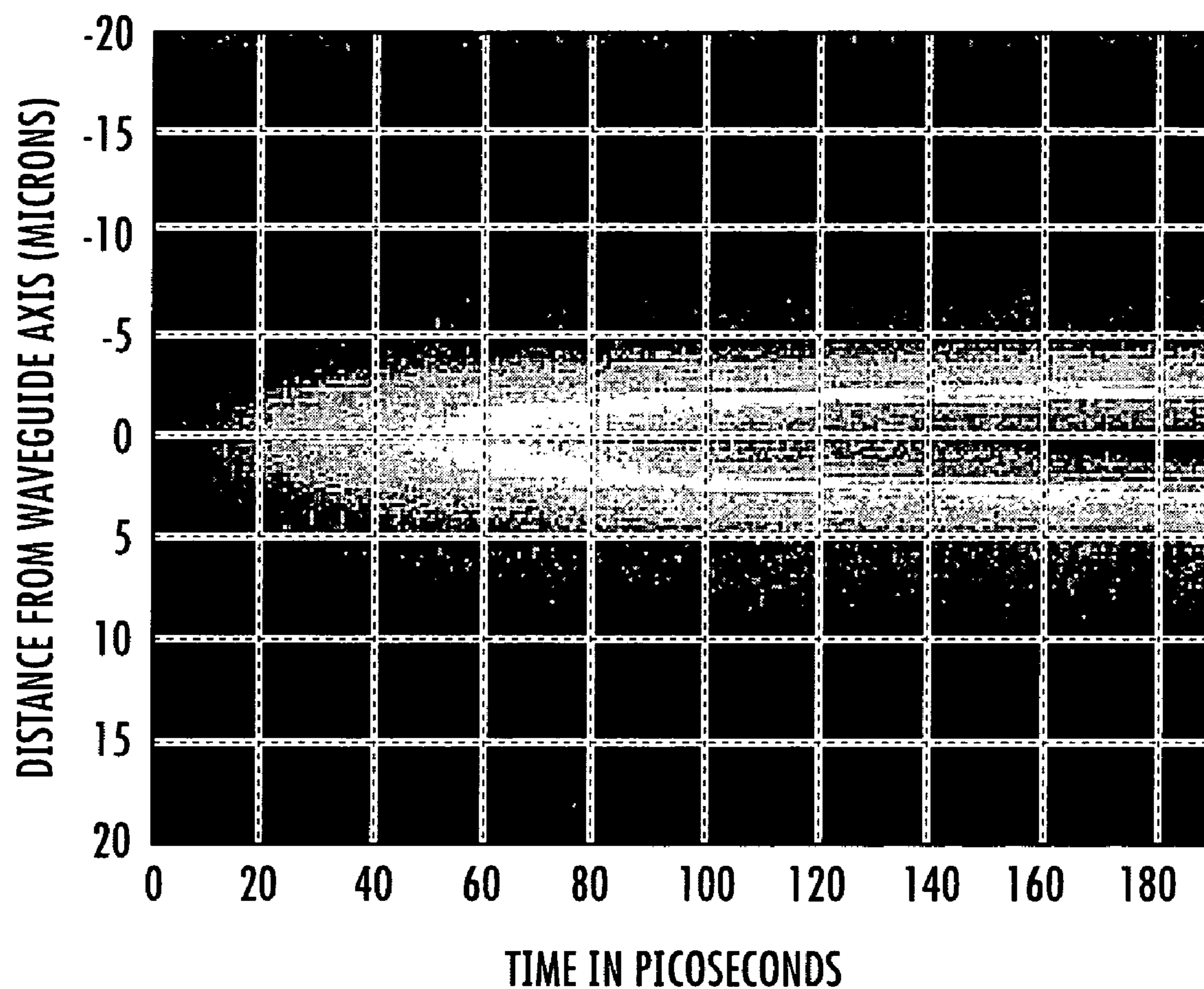
TRANSIENT FIELD PATTERNS IN RESONATOR GUIDE
