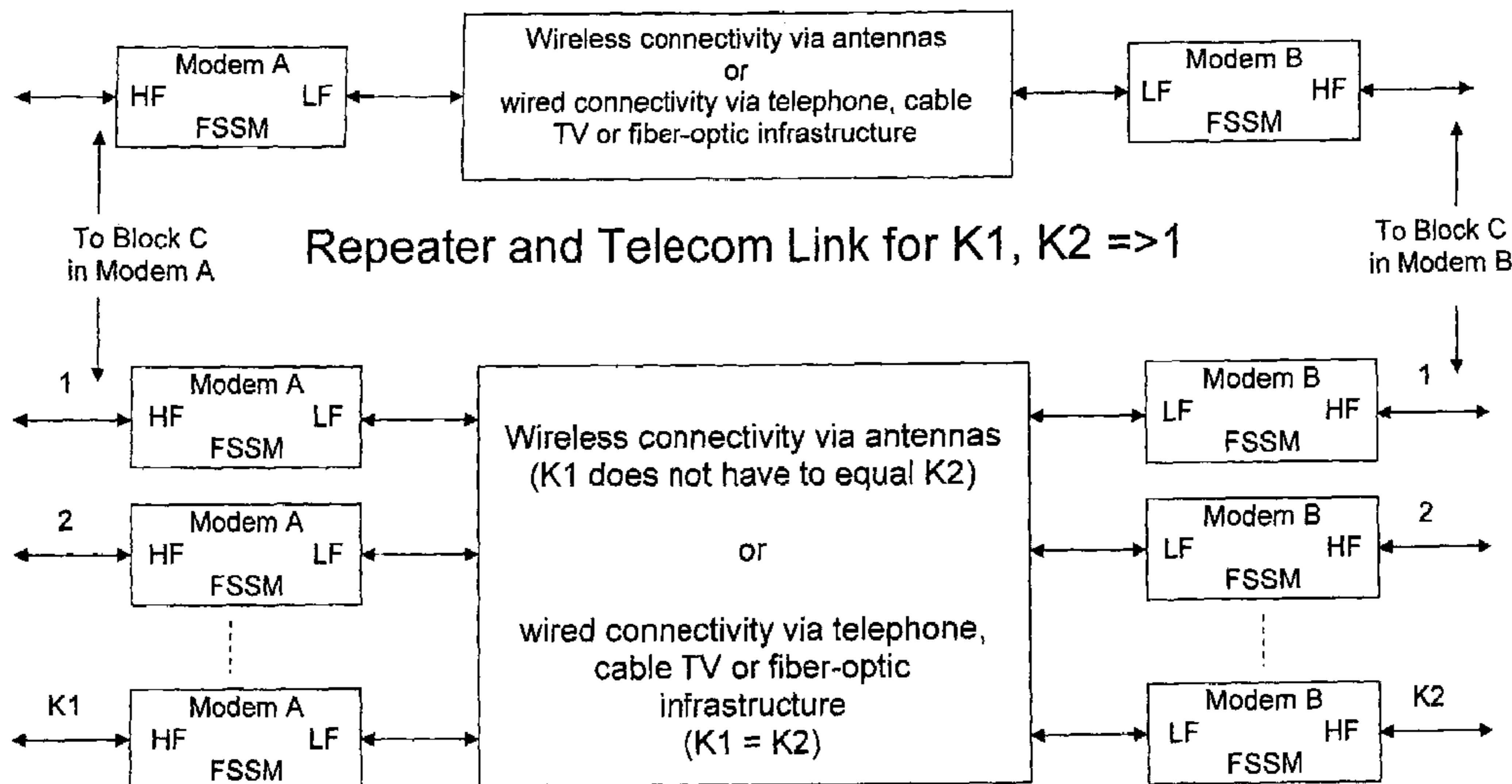
Repeater and Telecom Link (Block D of Fig. 1) for K=1
