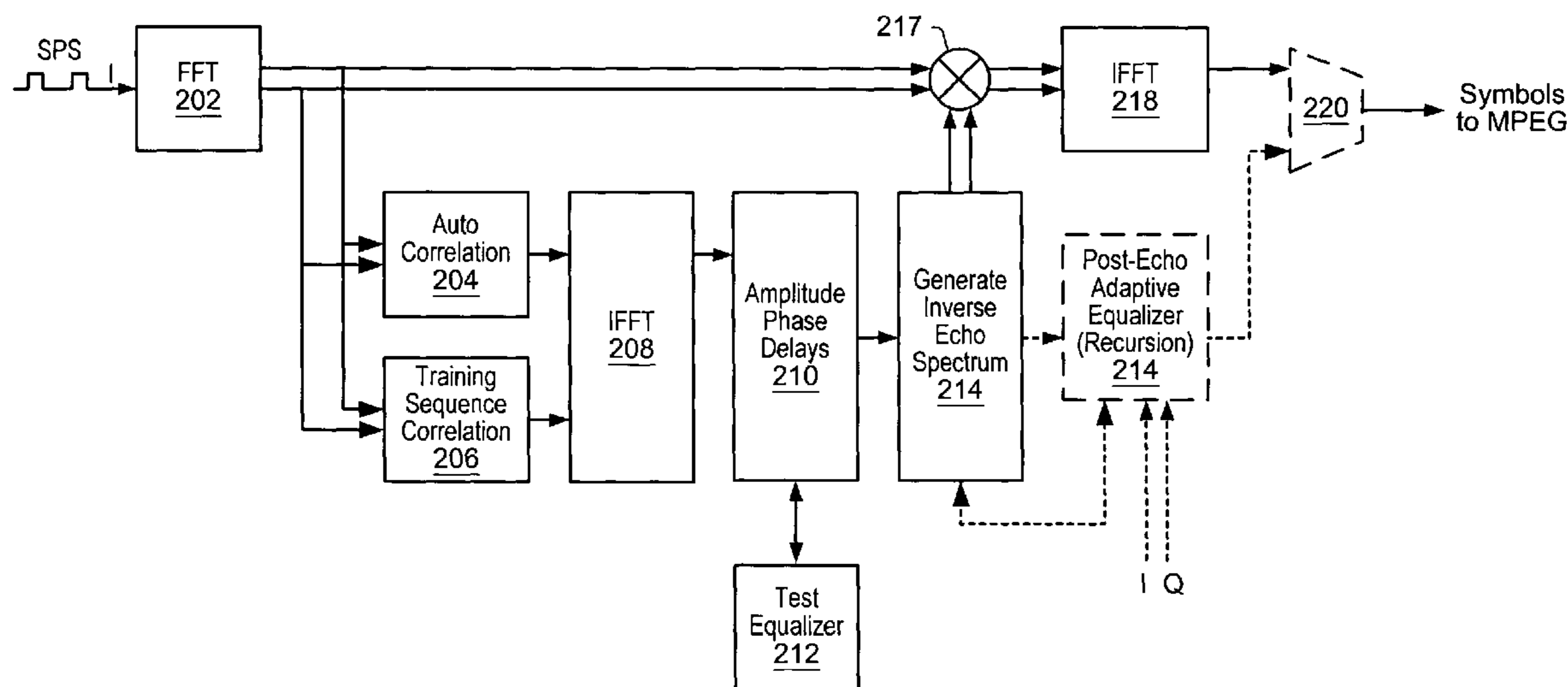
Overview of frequency Domain Equalization Algorithm
