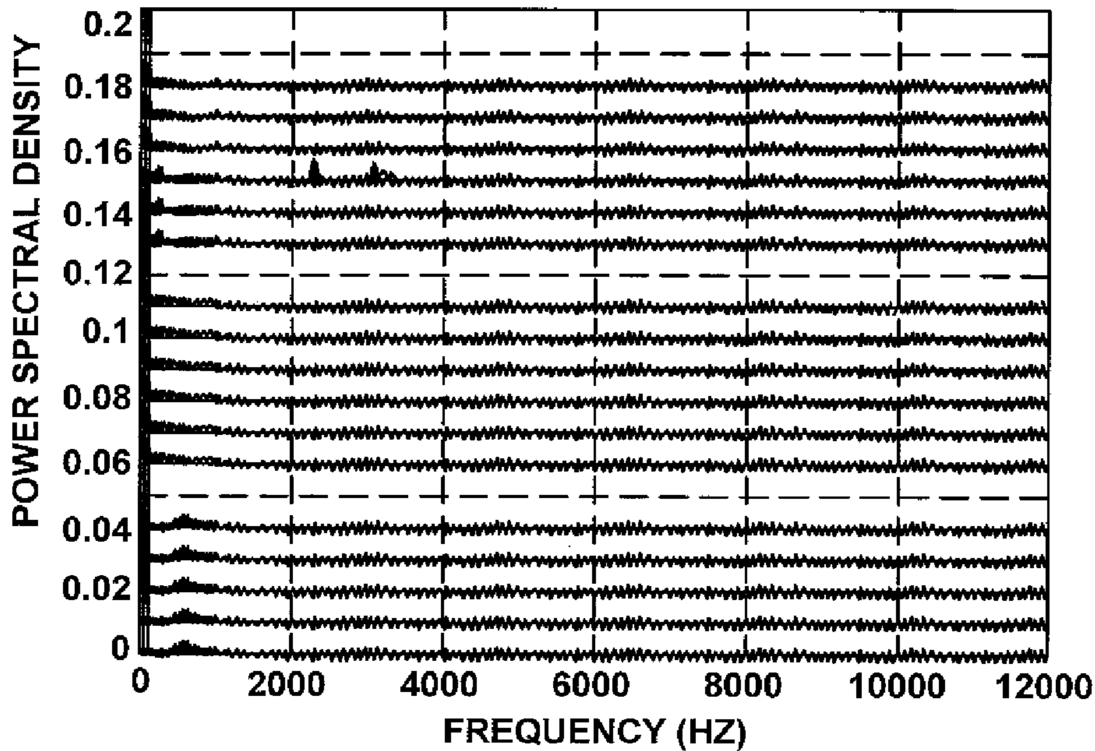
FFT (HELIUM IN SPINDLE AIR BEARING & HELIUM IN ACTUATOR BEARING)
