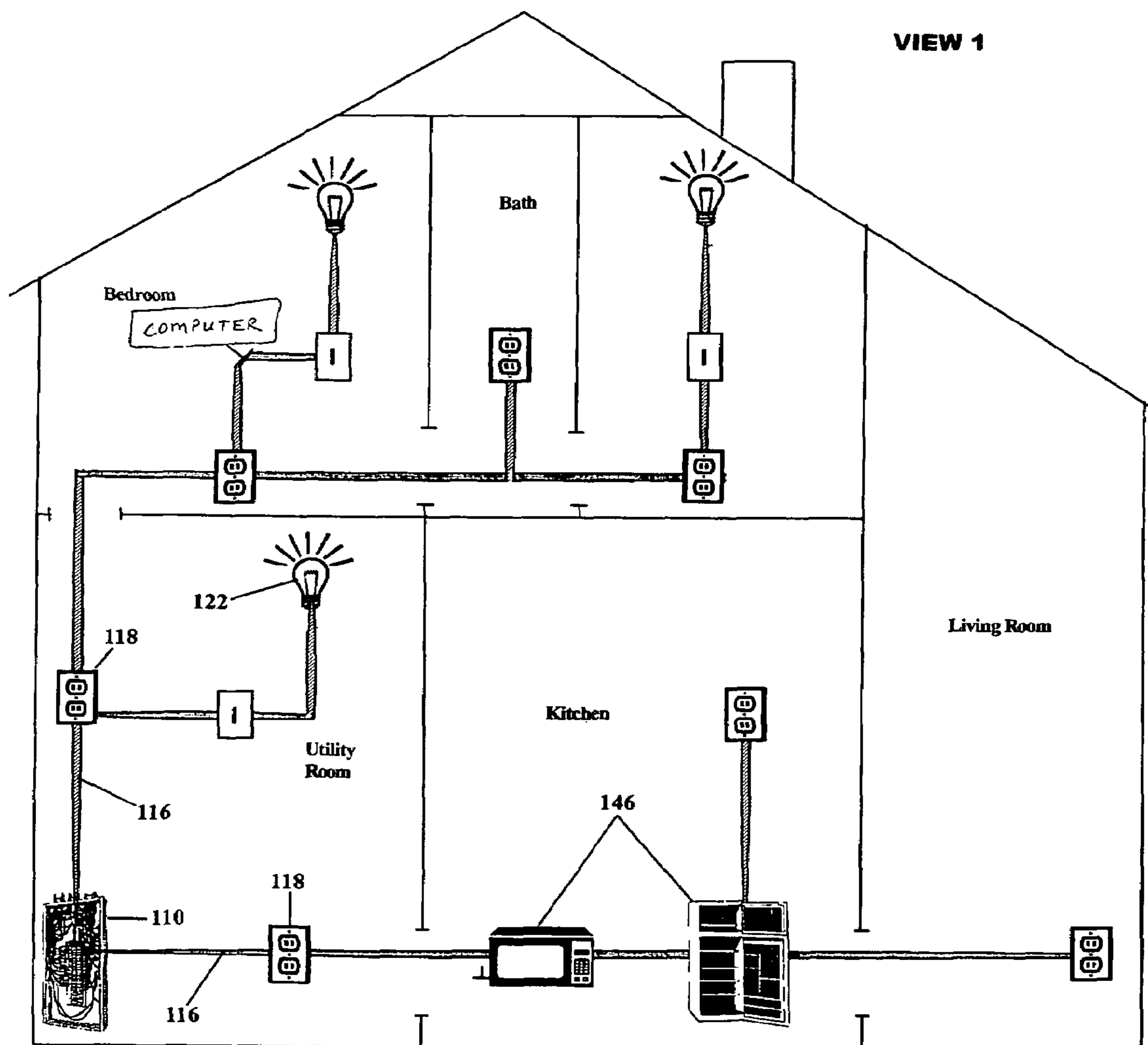
ELECTRICAL PANEL ARC FAULT AND GROUND FAULT CIRCUIT PROTECTION
