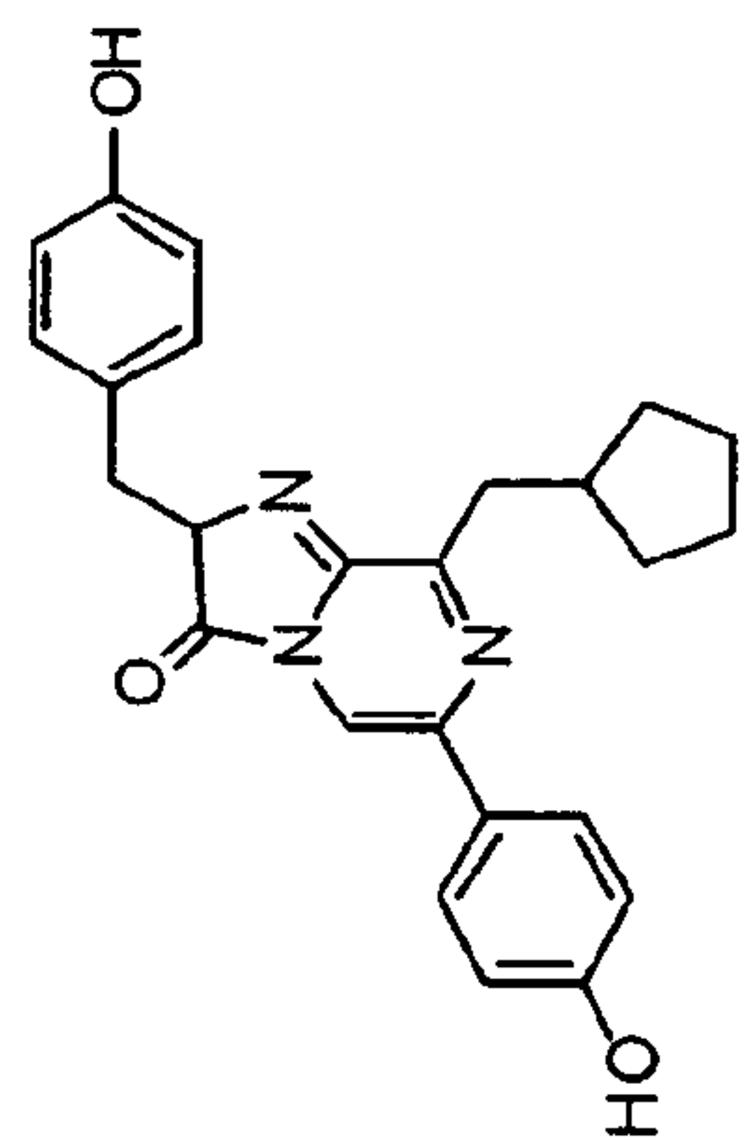
Fig. 16 Coelenterazine Analogs
