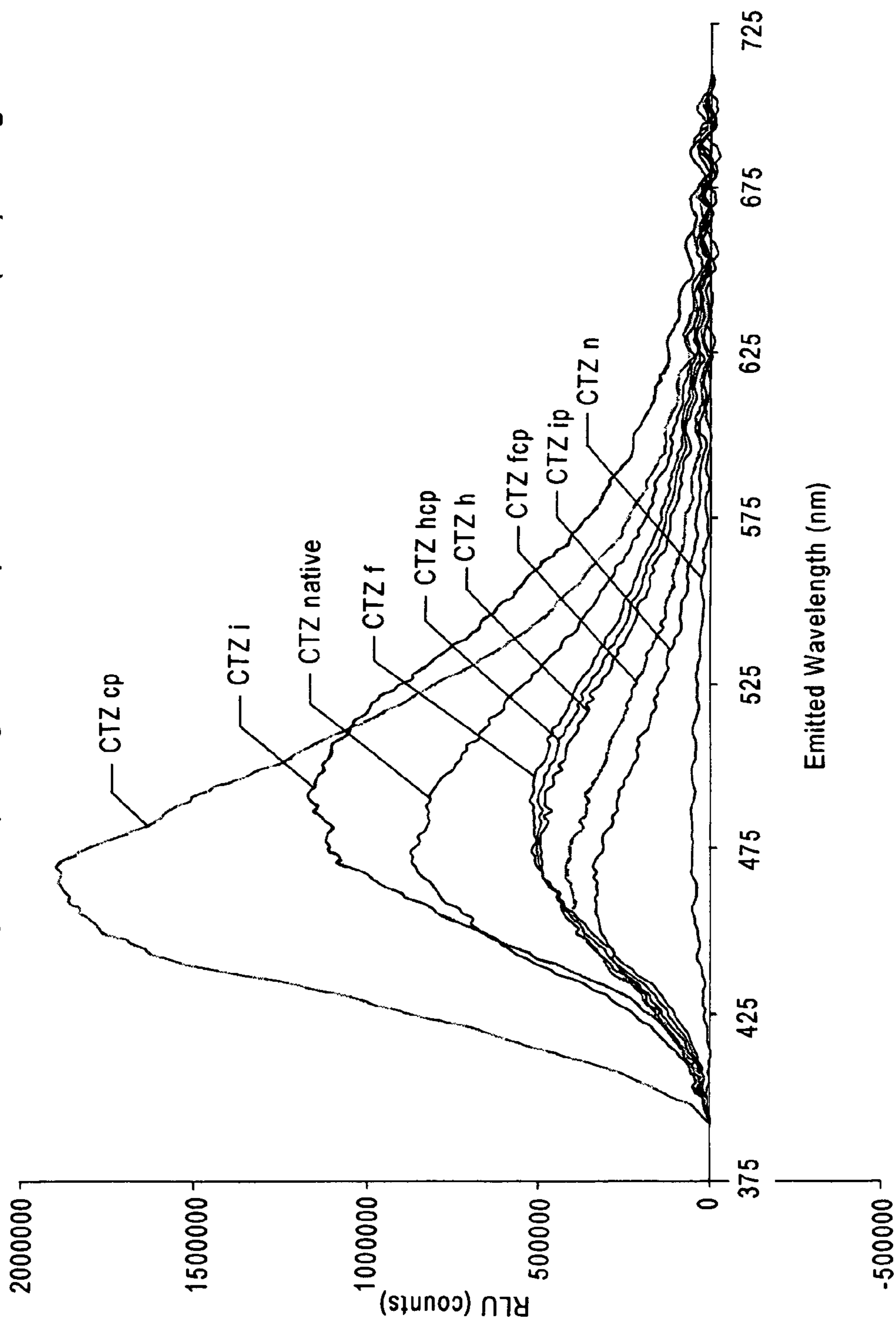
Fig. 4 Crude Aequorin 5 (Average of 2 Trials) With Coelenterazine (CTZ) Analogues
