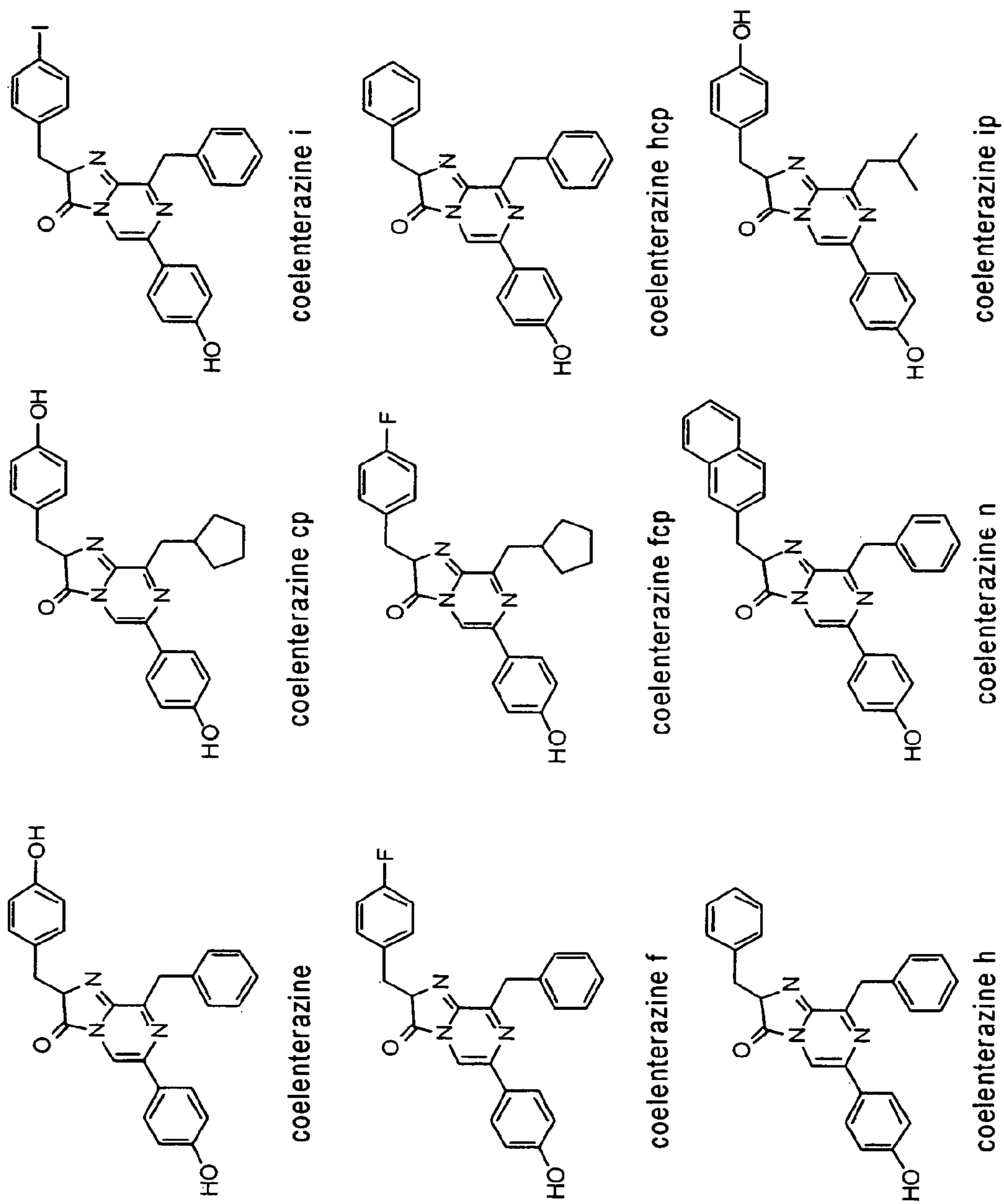
Fig. 16 Coelenterazine Analogs
