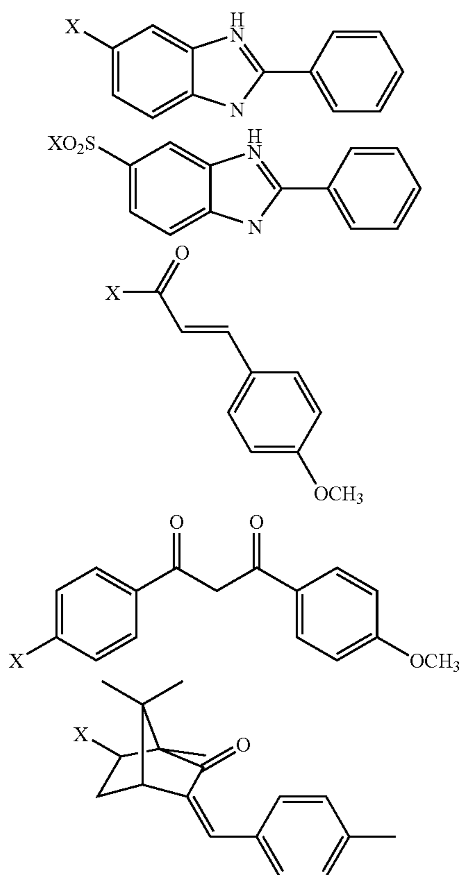
Scheme 1: Examples of Suitable Precursors for Introducing Radicals R^1 , R^2 , R^3 , R^4 and R^5
