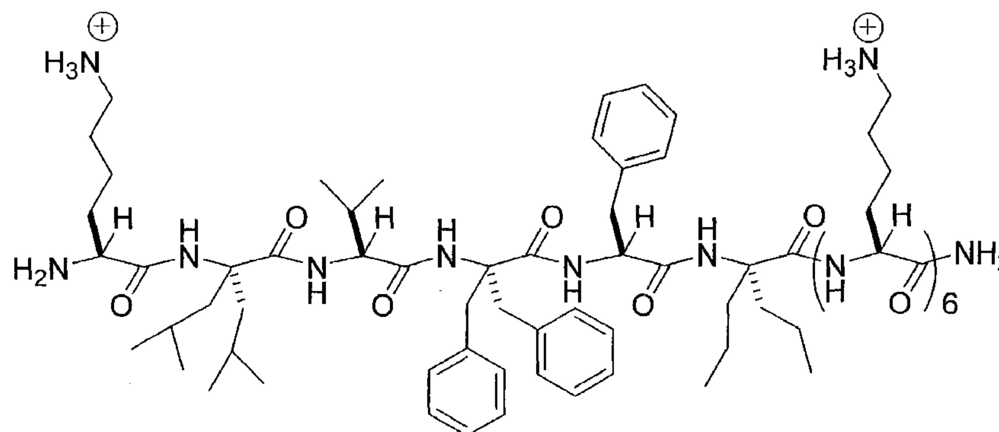
H-Lys-Dibg-Val-Dbzg-Phe-Dpg-(Lys) 6 -NH 2
