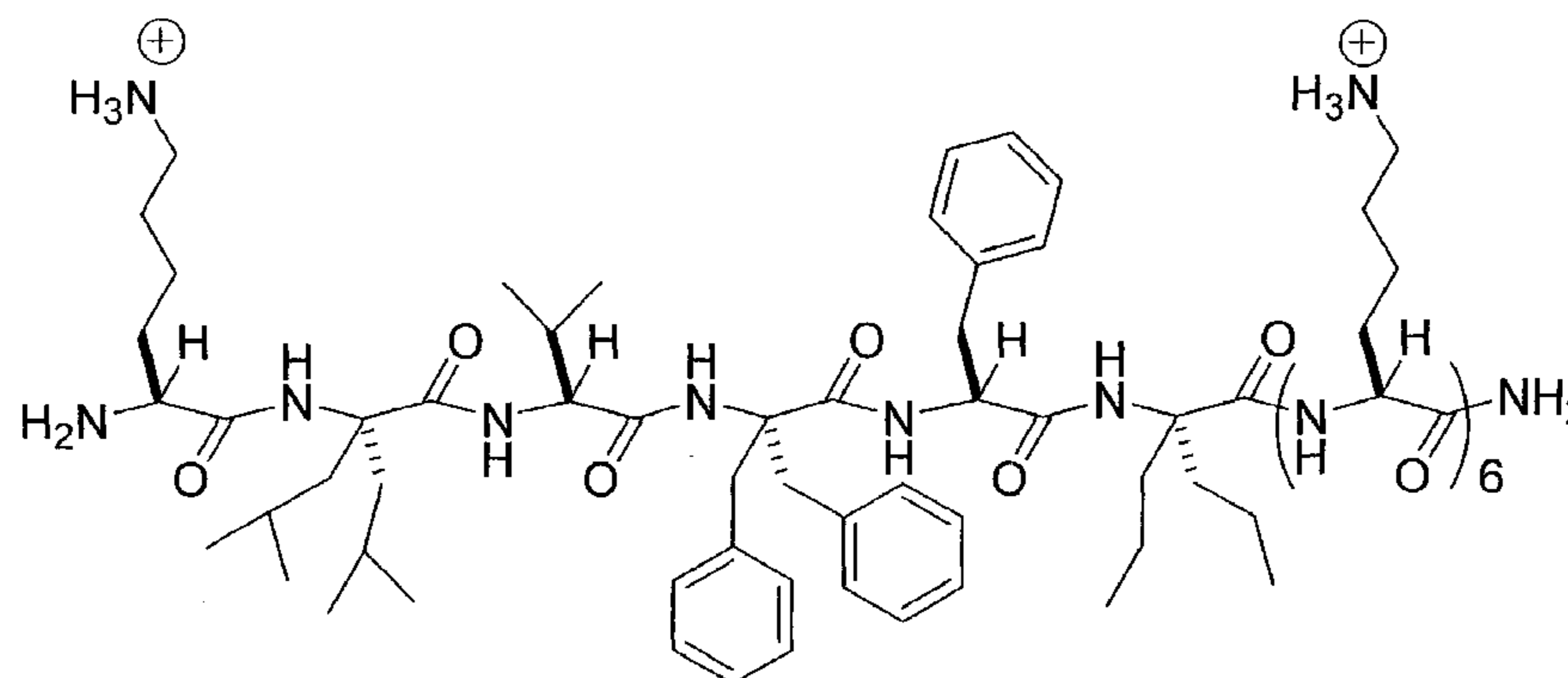
H-Lys-Dibg-Val-Dbzg-Phe-Dpg-(Lys) 6 -NH 2
