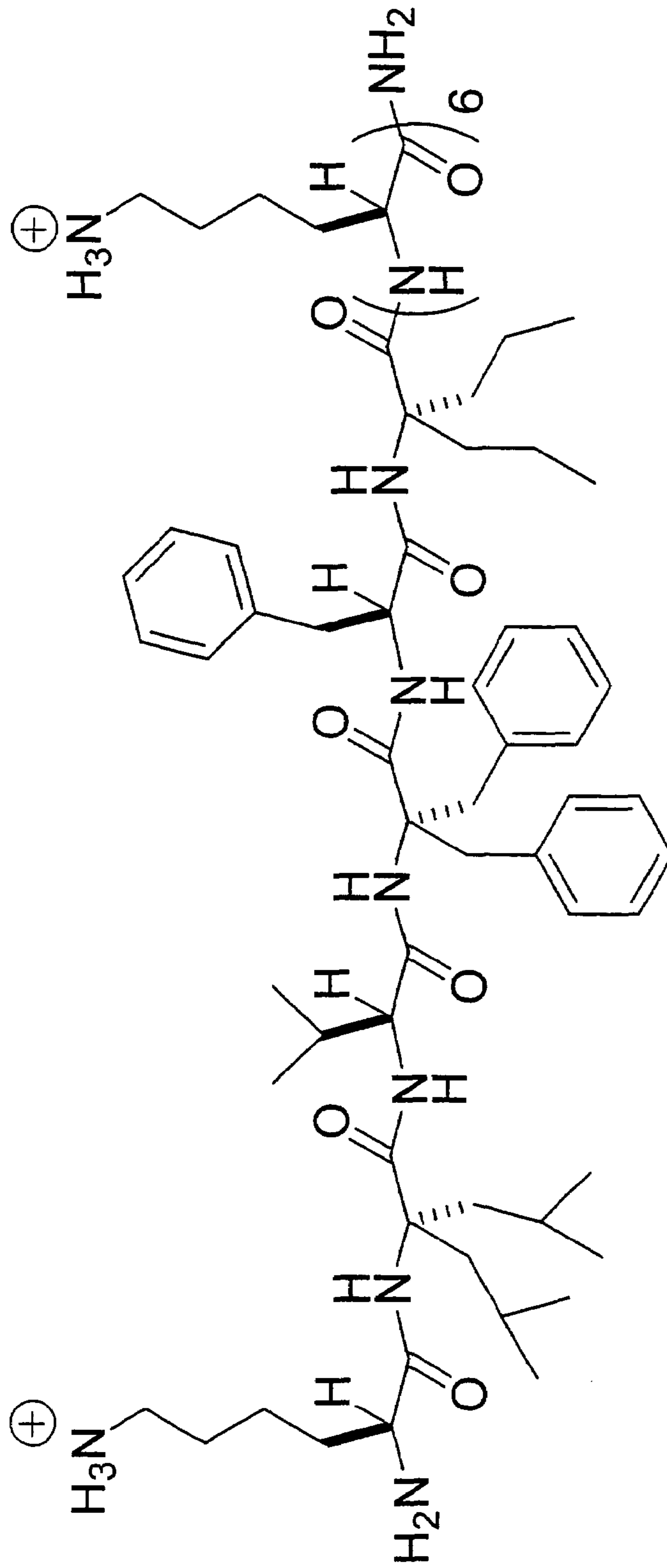
H-Lys-Dibg-Val-Dbzg-Phe-Dpg-(Lys) 6 -NH 2
