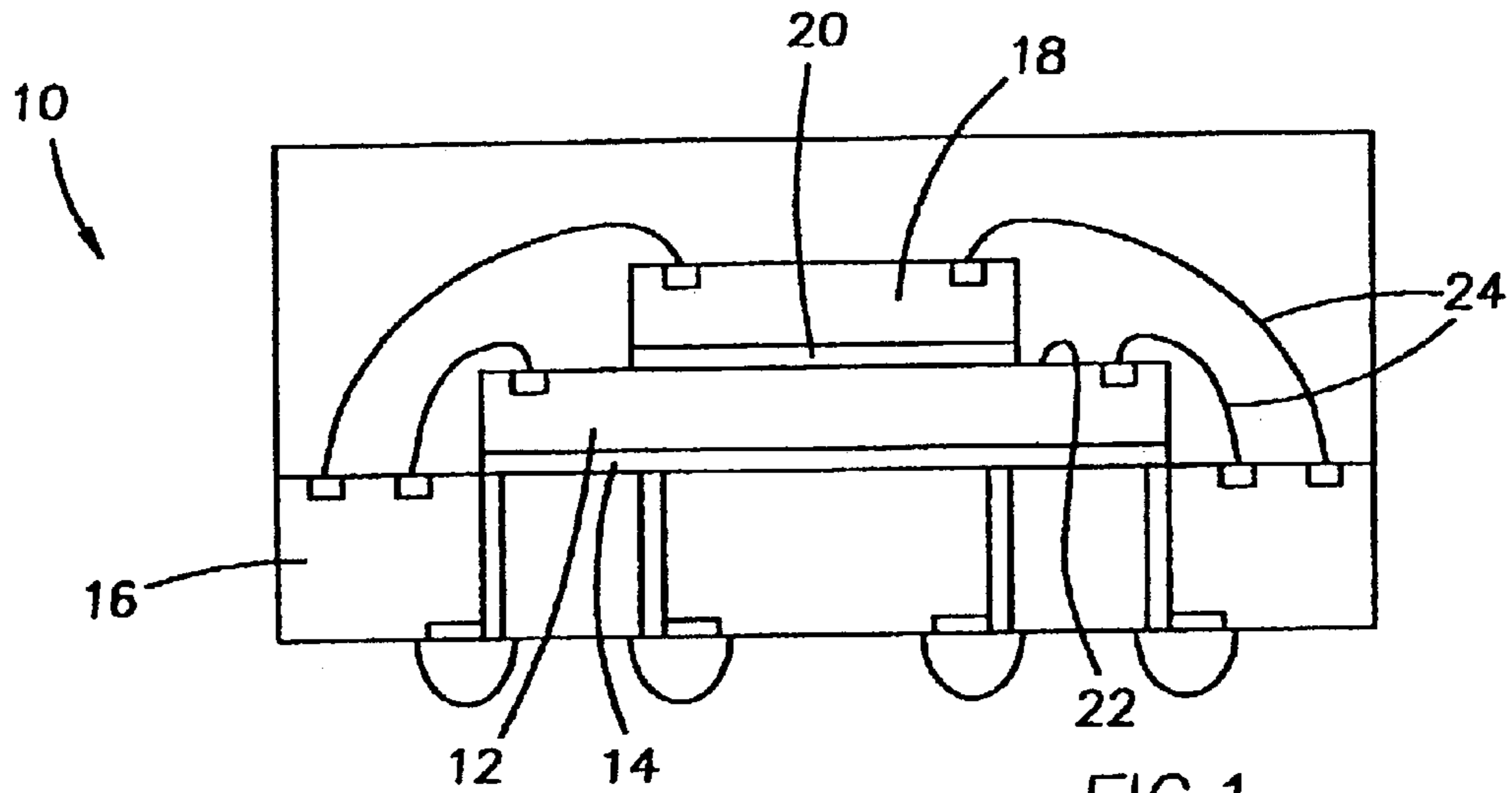
FIG. 1 PRIOR ART
