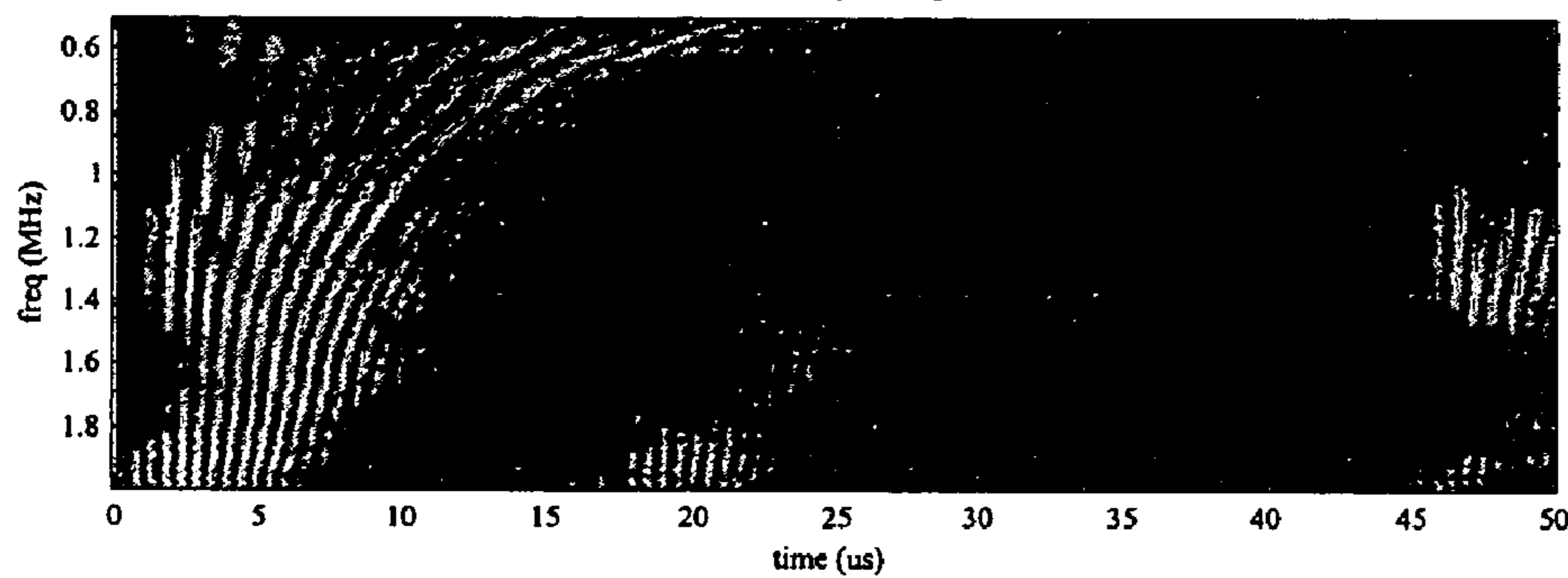
Norm A-line through gel and glass bead
