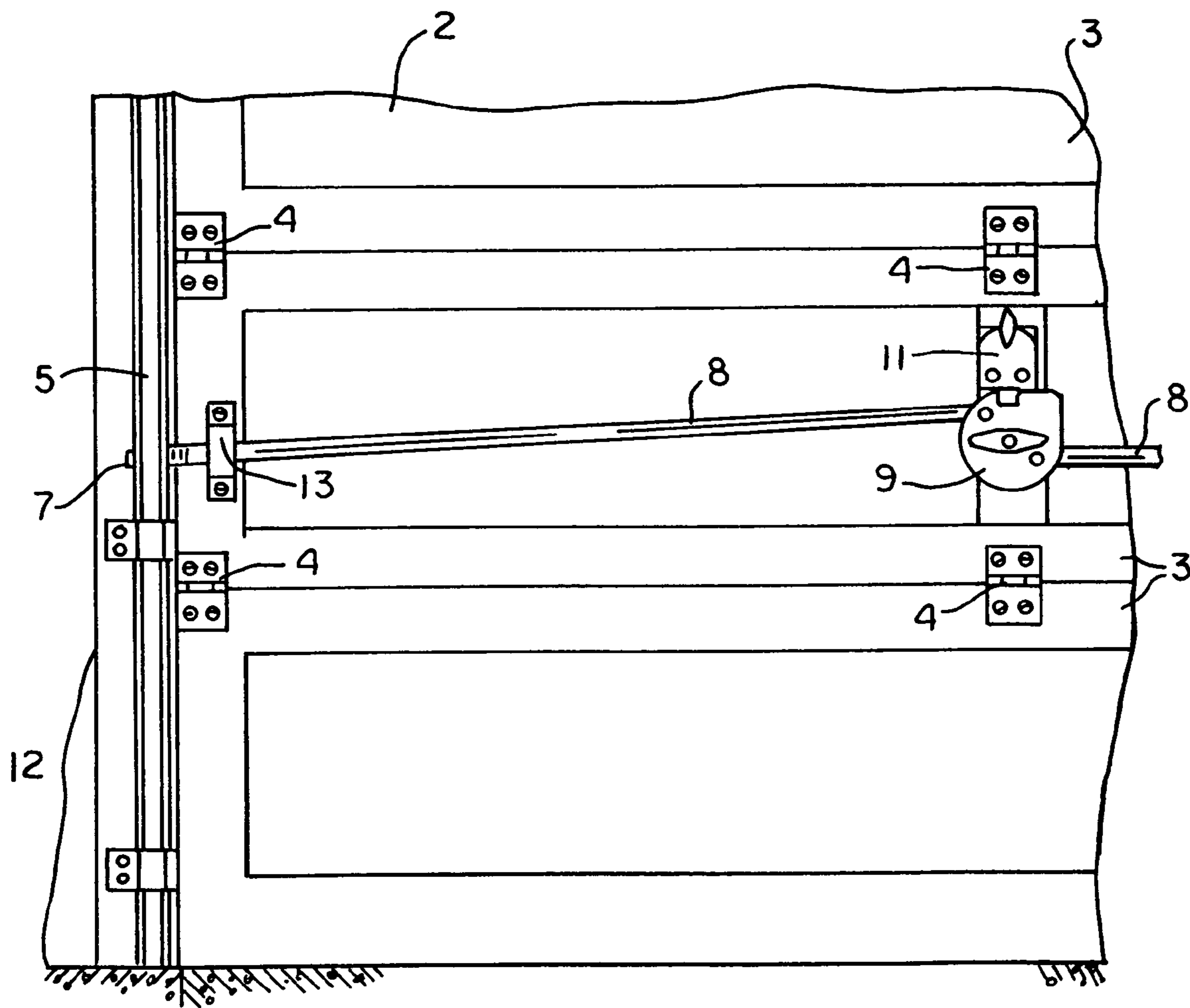
FIG. 1 PRIOR ART
