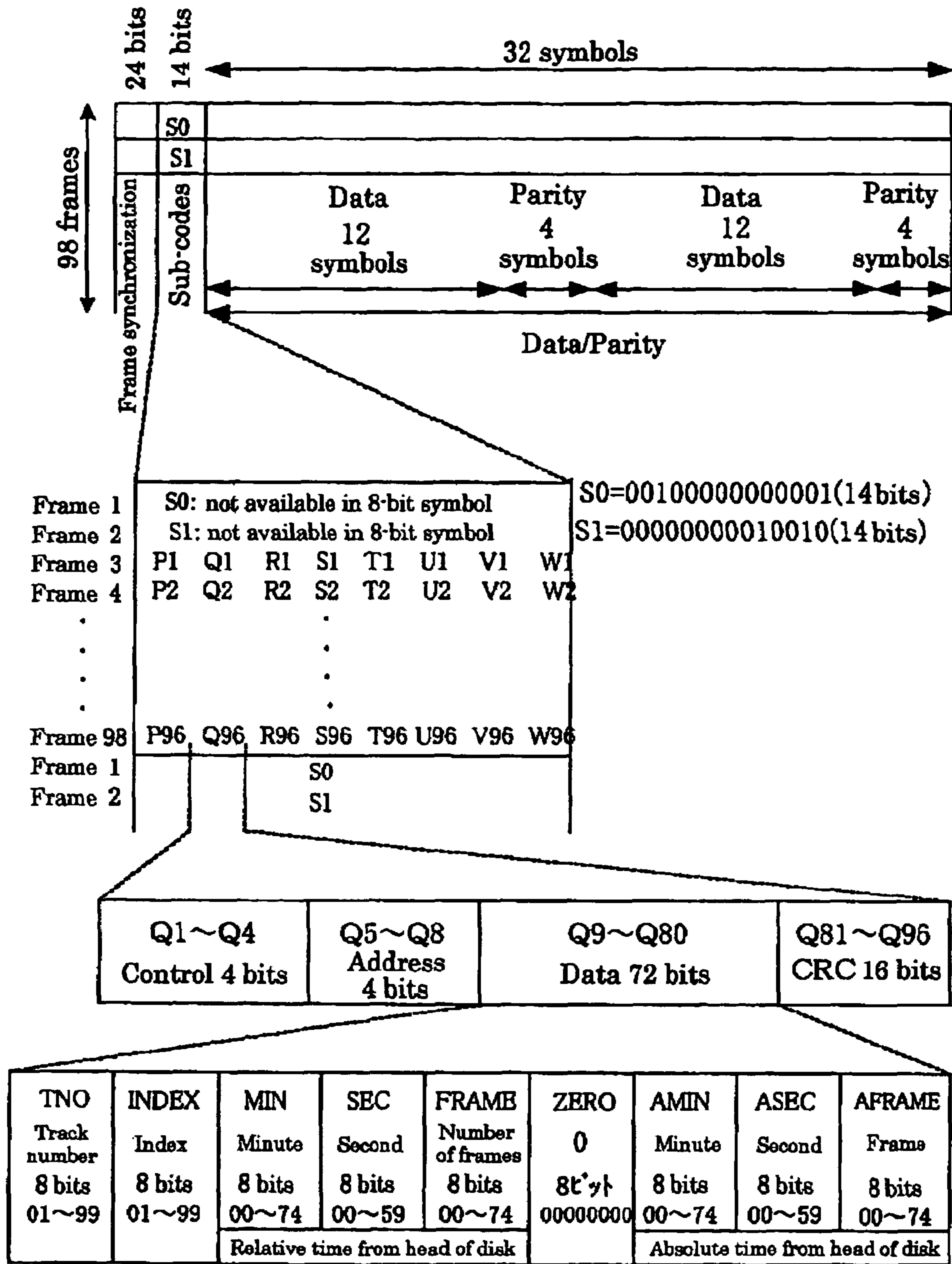
FIG. 1 (BACKGROUND ART)
