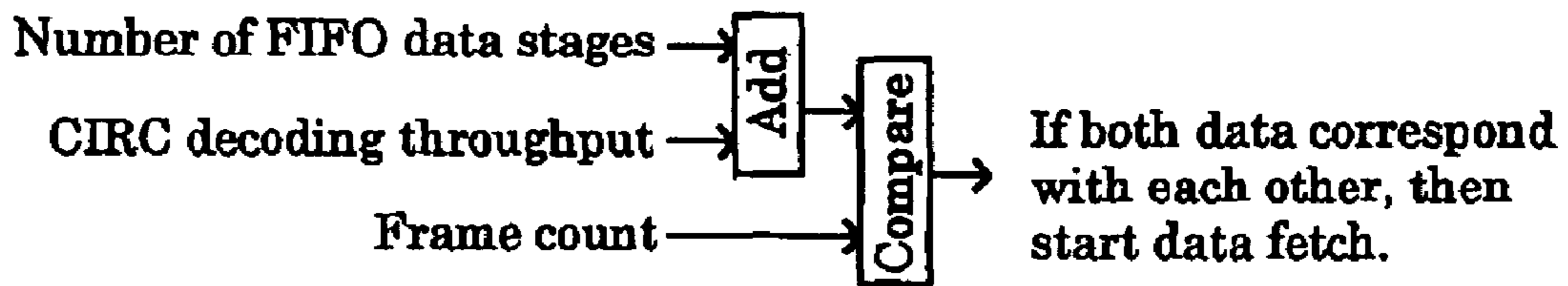
FIG. 3C (BACKGROUND ART)
