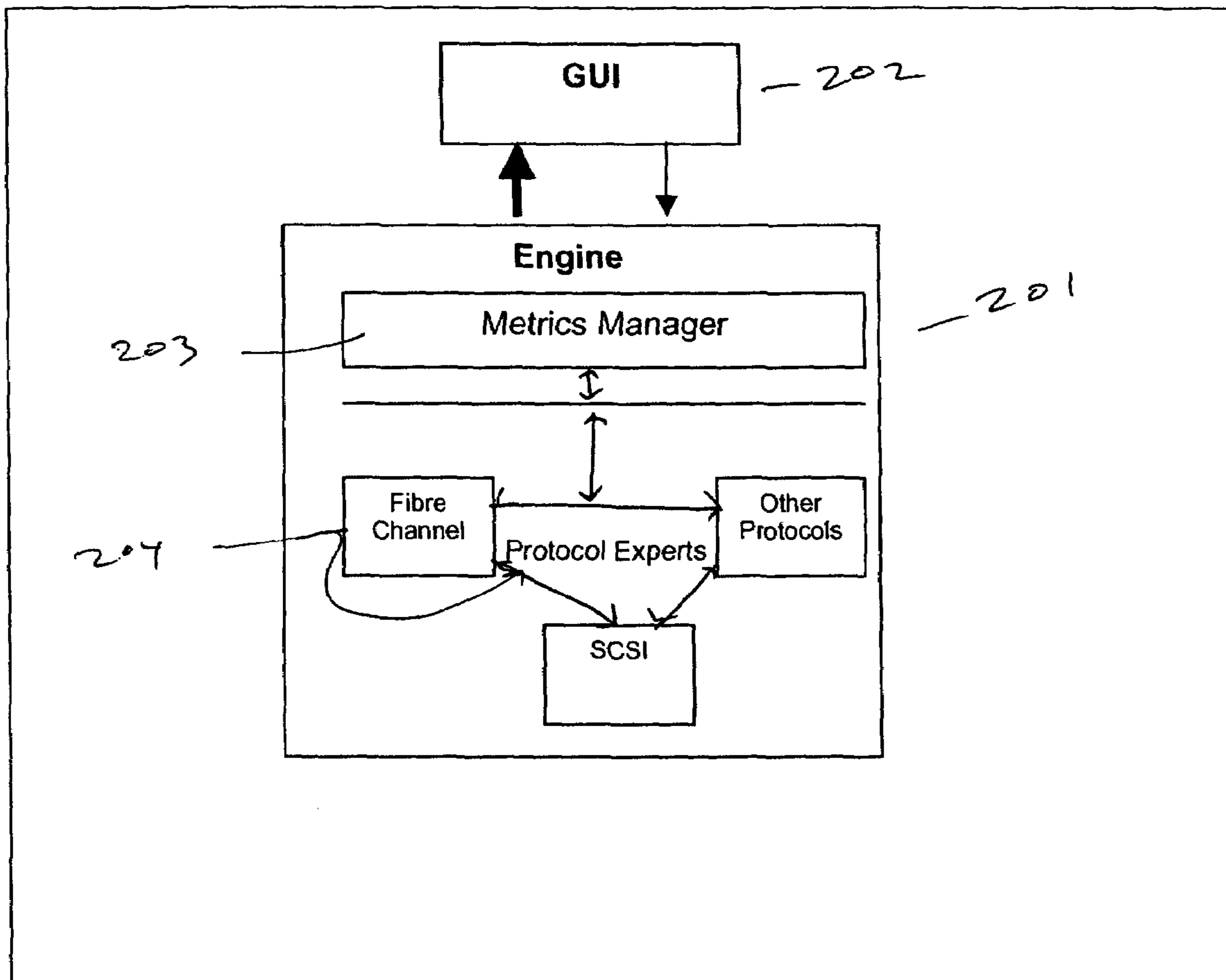
Figure 2. SANMetrics Architecture
