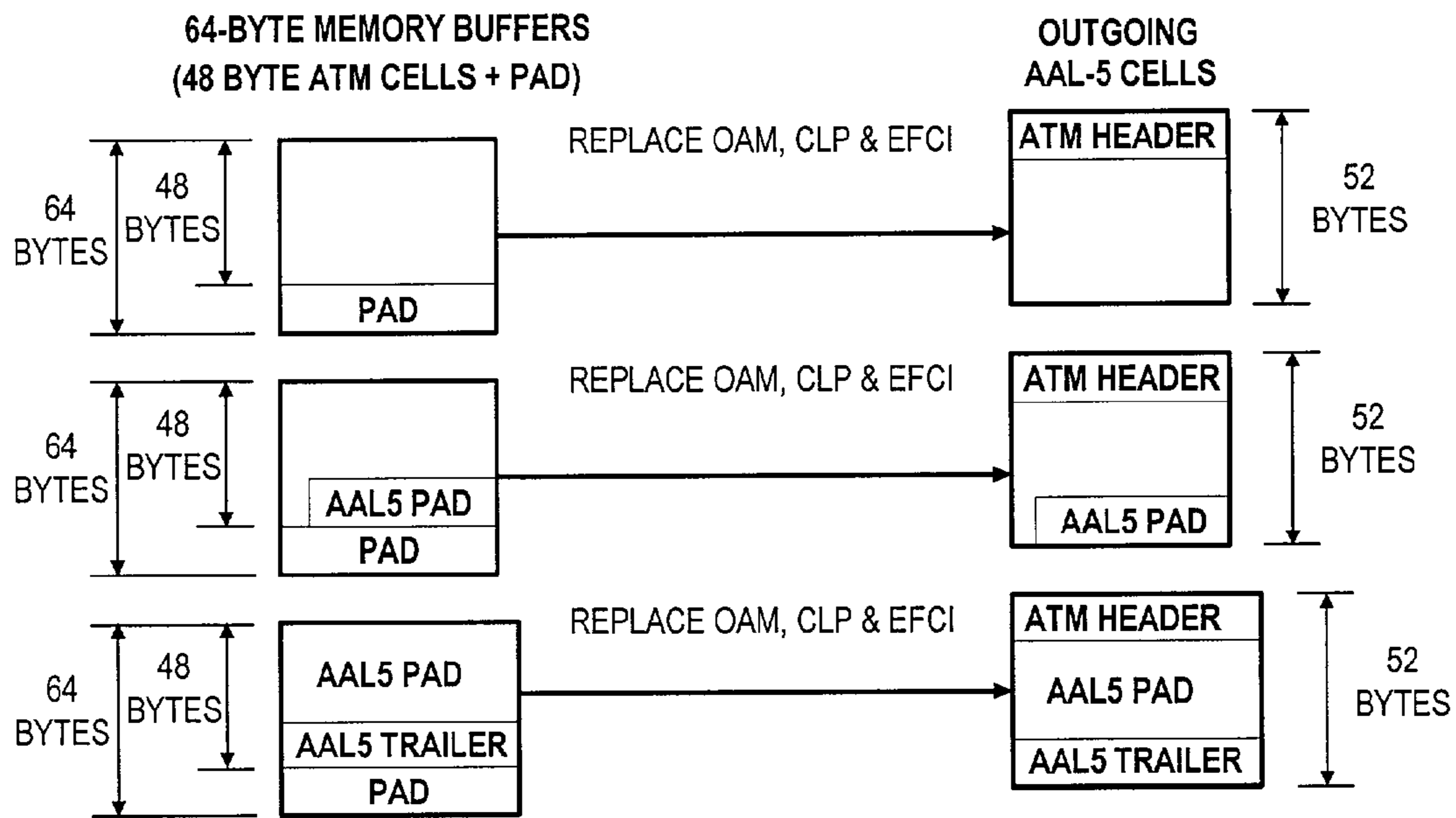
REASSEMBLY TYPE 7 (INGRESS APPLICATION TYPES 10 AND 13)
