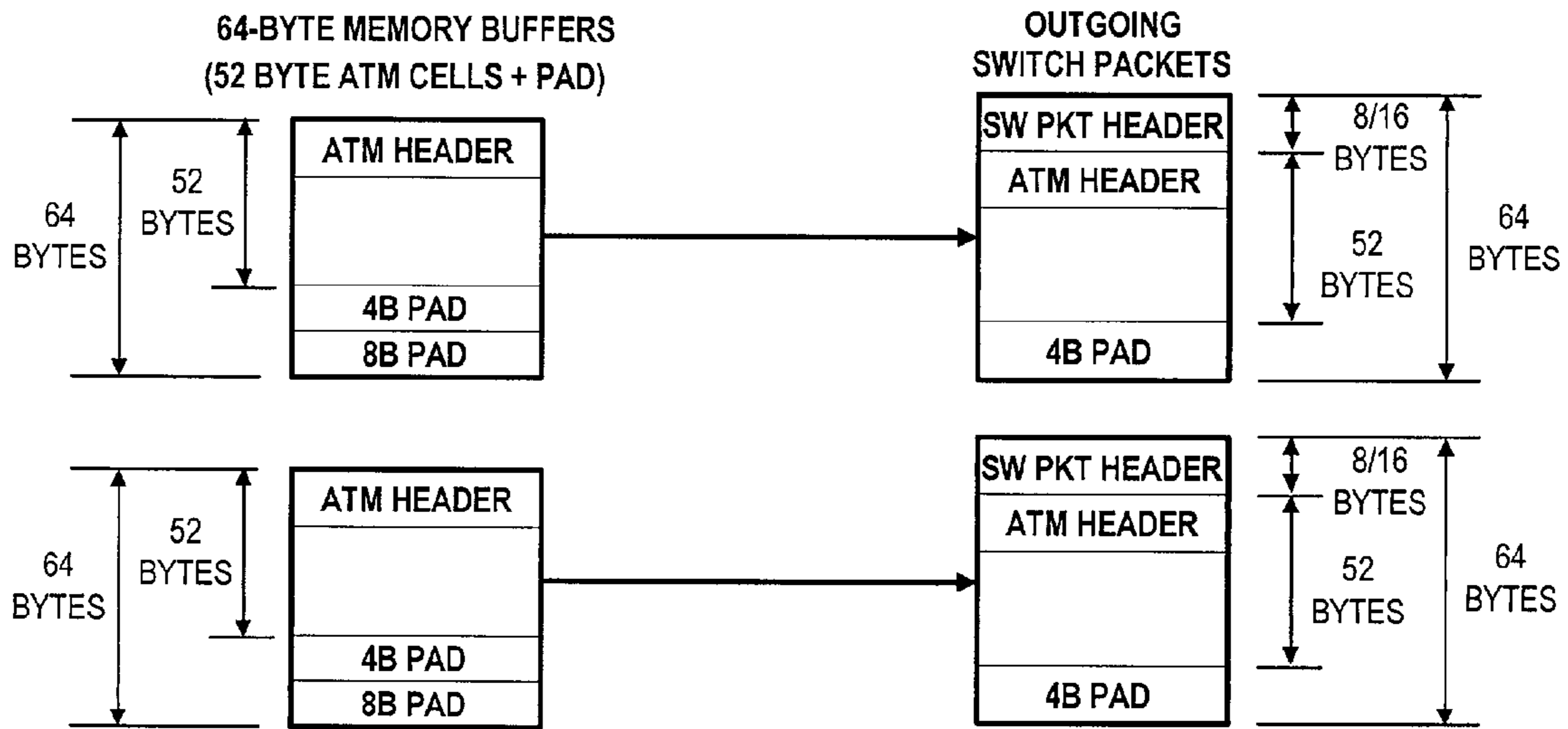
REASSEMBLY TYPE 2 (INGRESS APPLICATION TYPE 4) FIG. 60D
