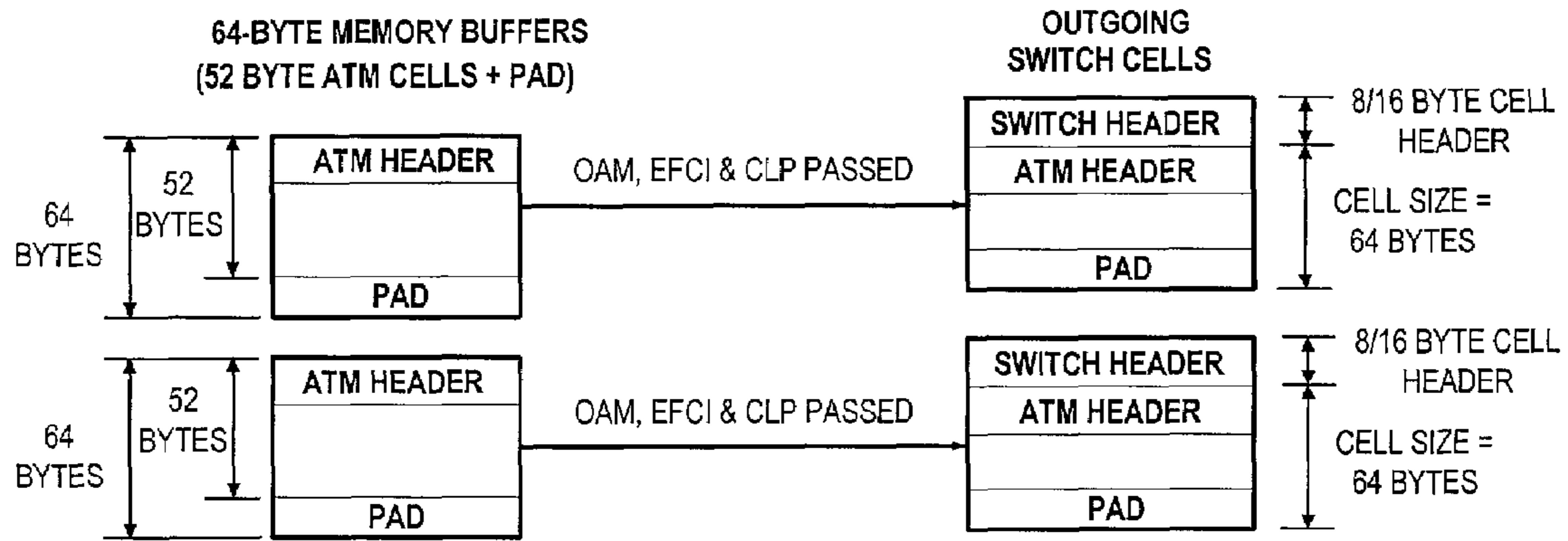
REASSEMBLY TYPE 1 (INGRESS APPLICATION TYPE 0)
