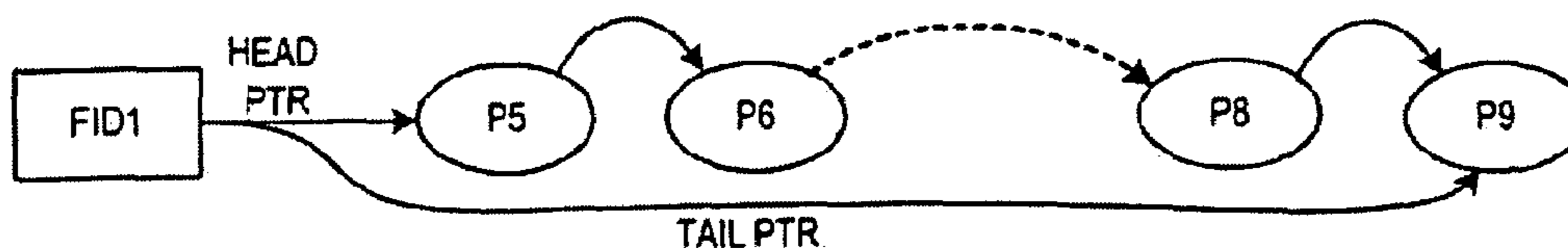
PACKET QUEUE
