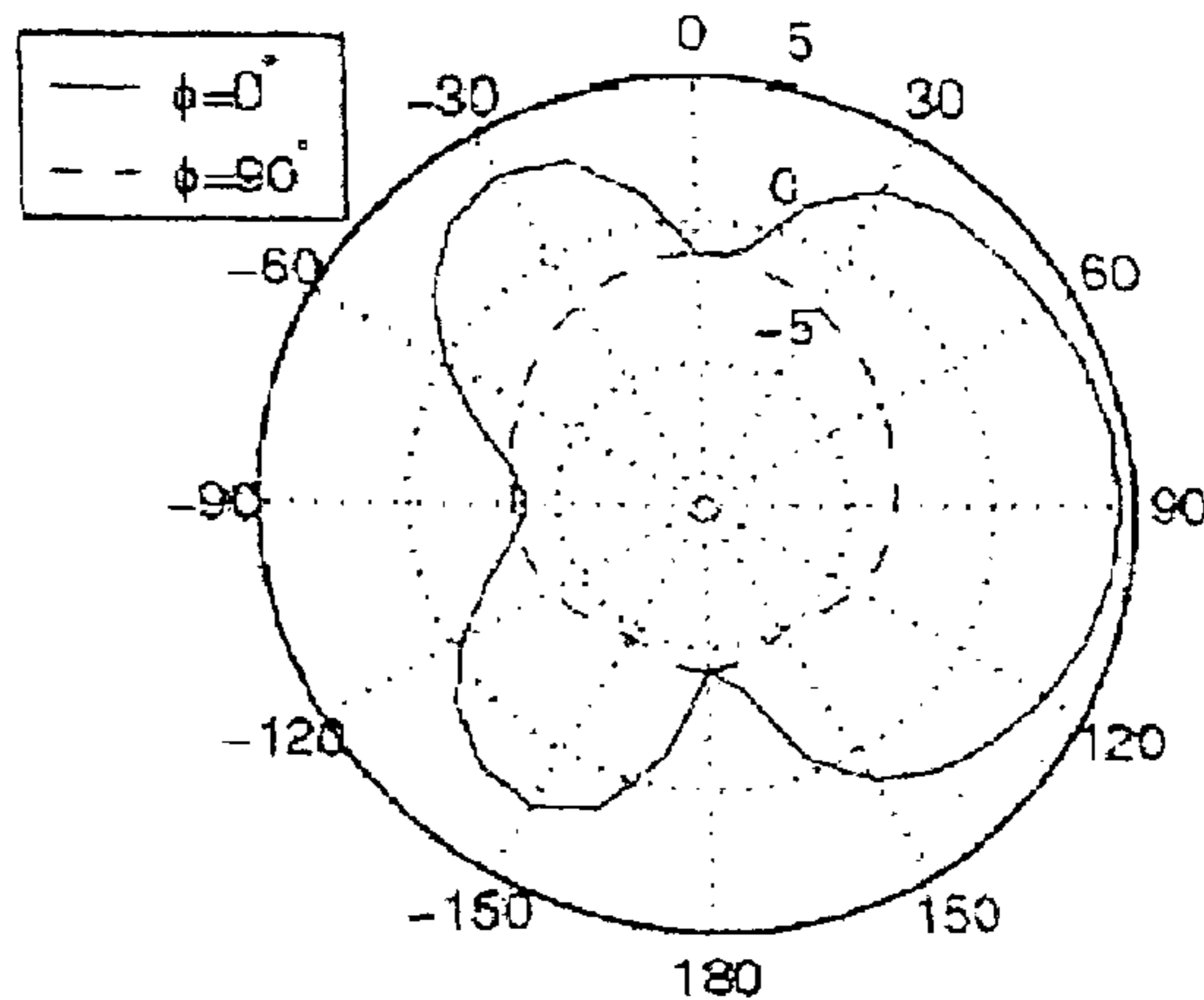
vertical radiation pattern
