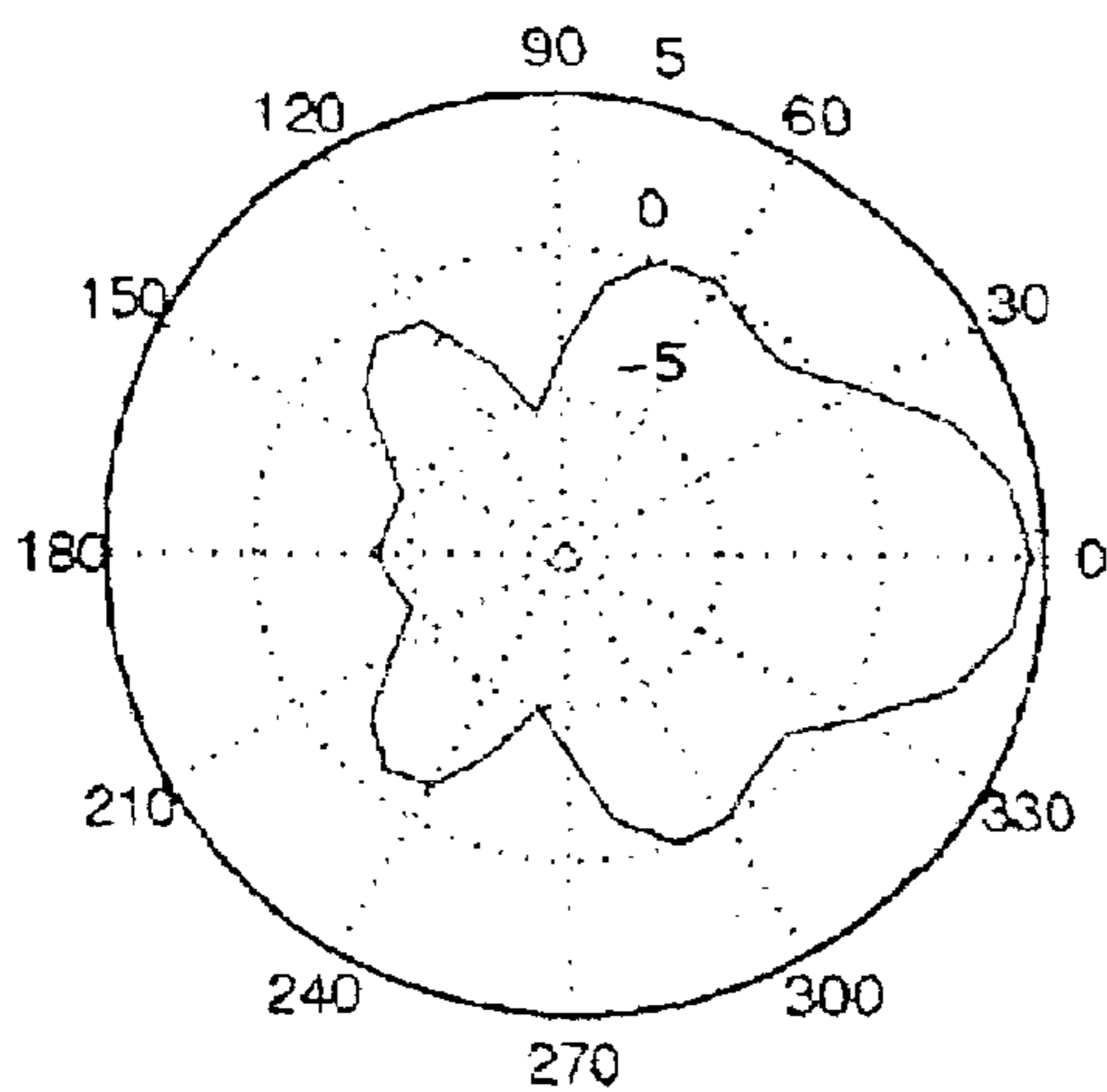
horizontal radiation pattern
