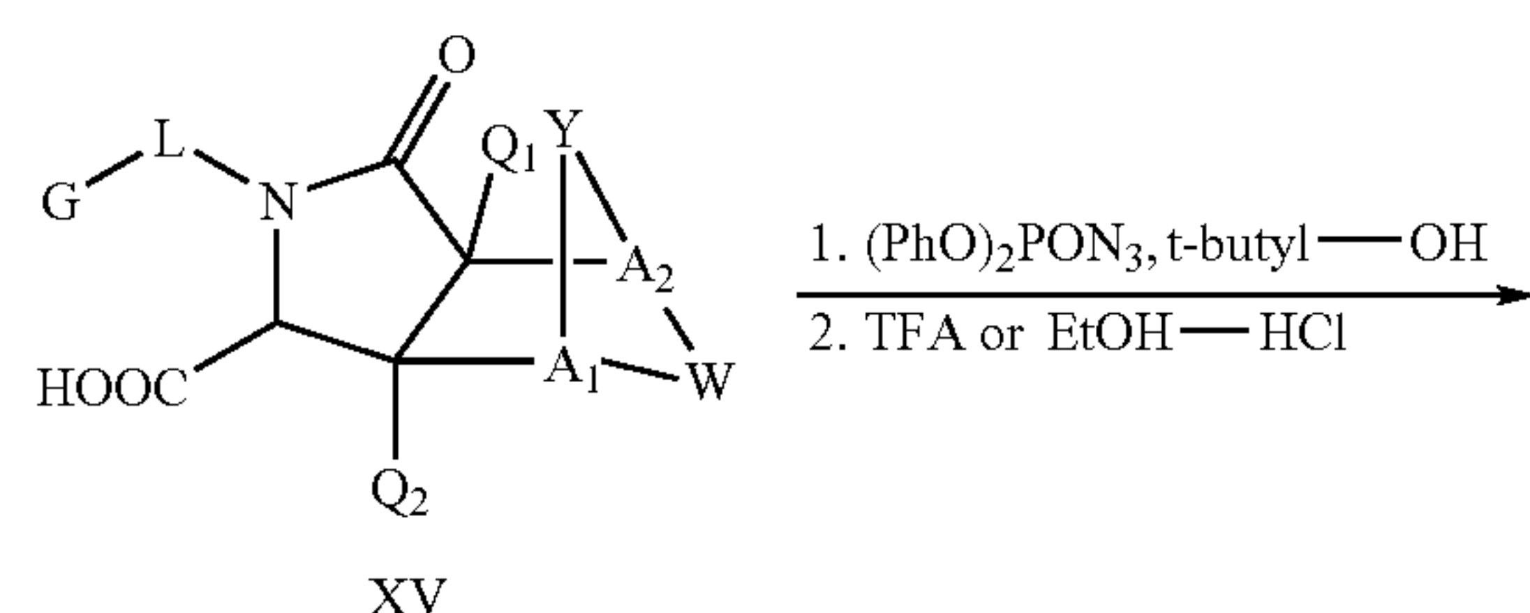
Scheme VIII
