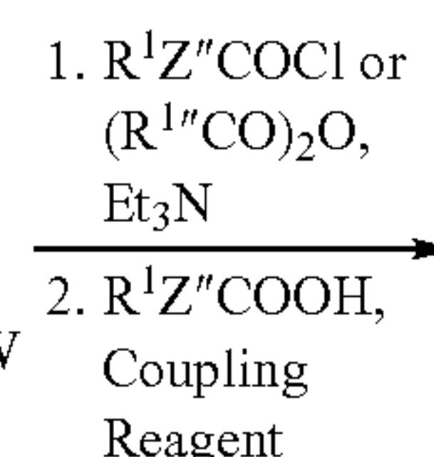
Scheme IX
