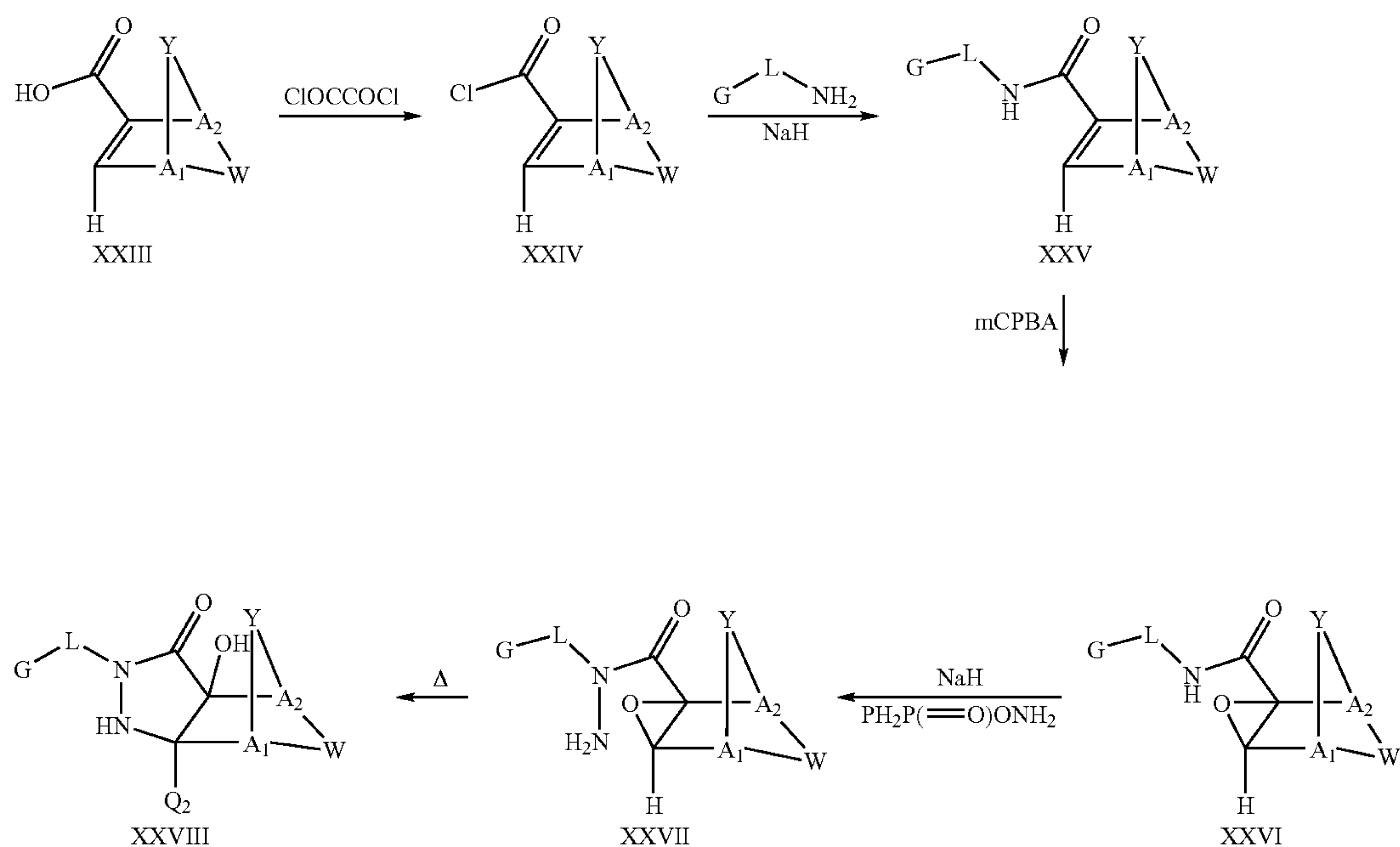
Scheme XII
