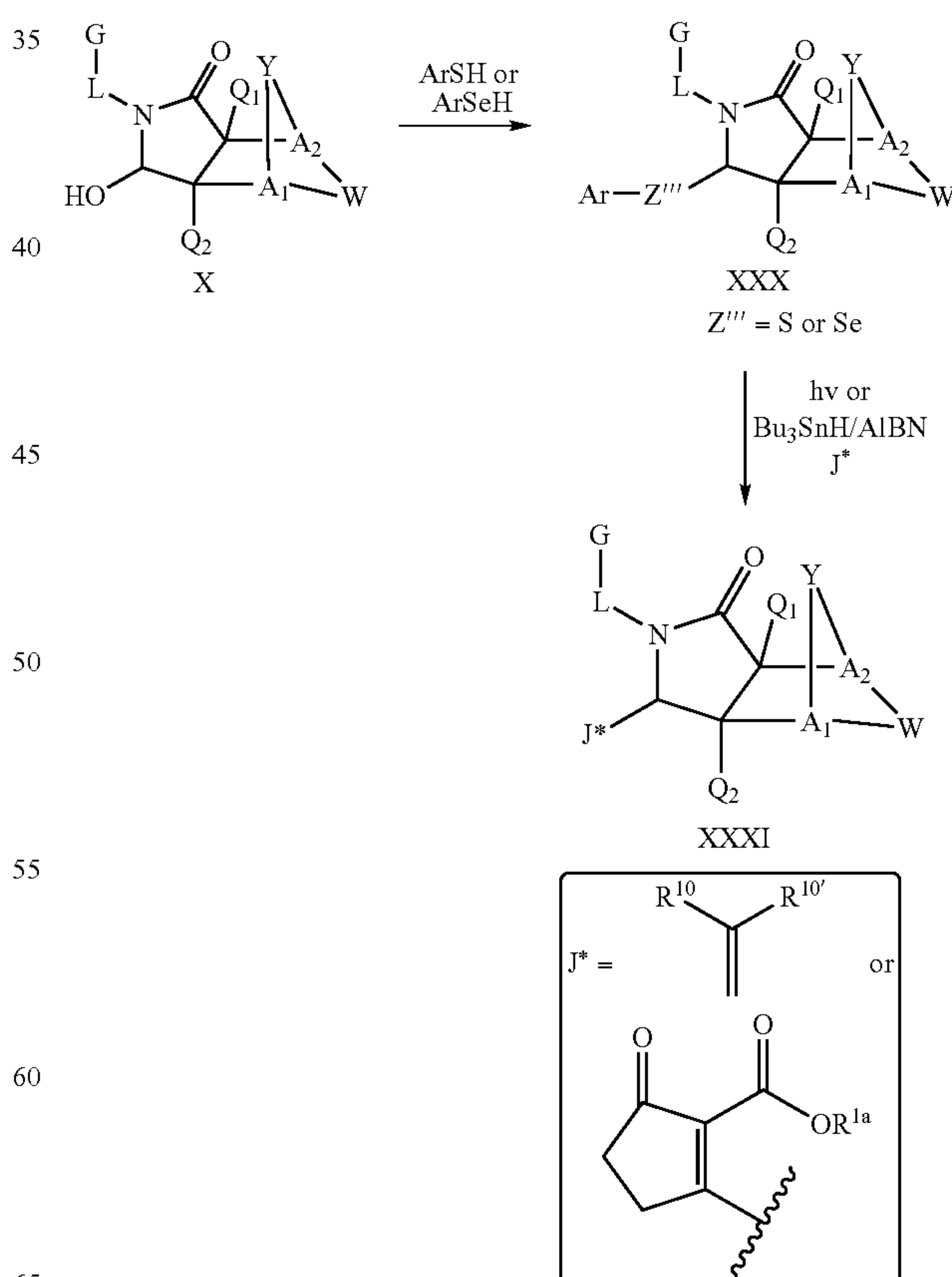
SCHEME XIV
