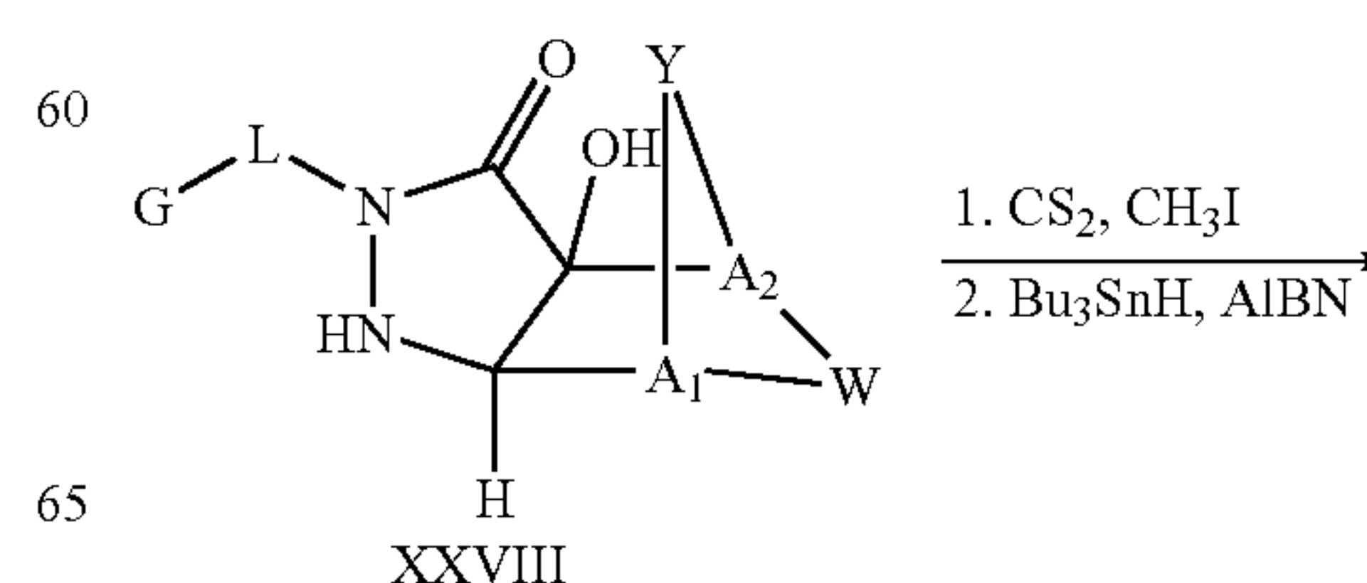
Scheme XXI
