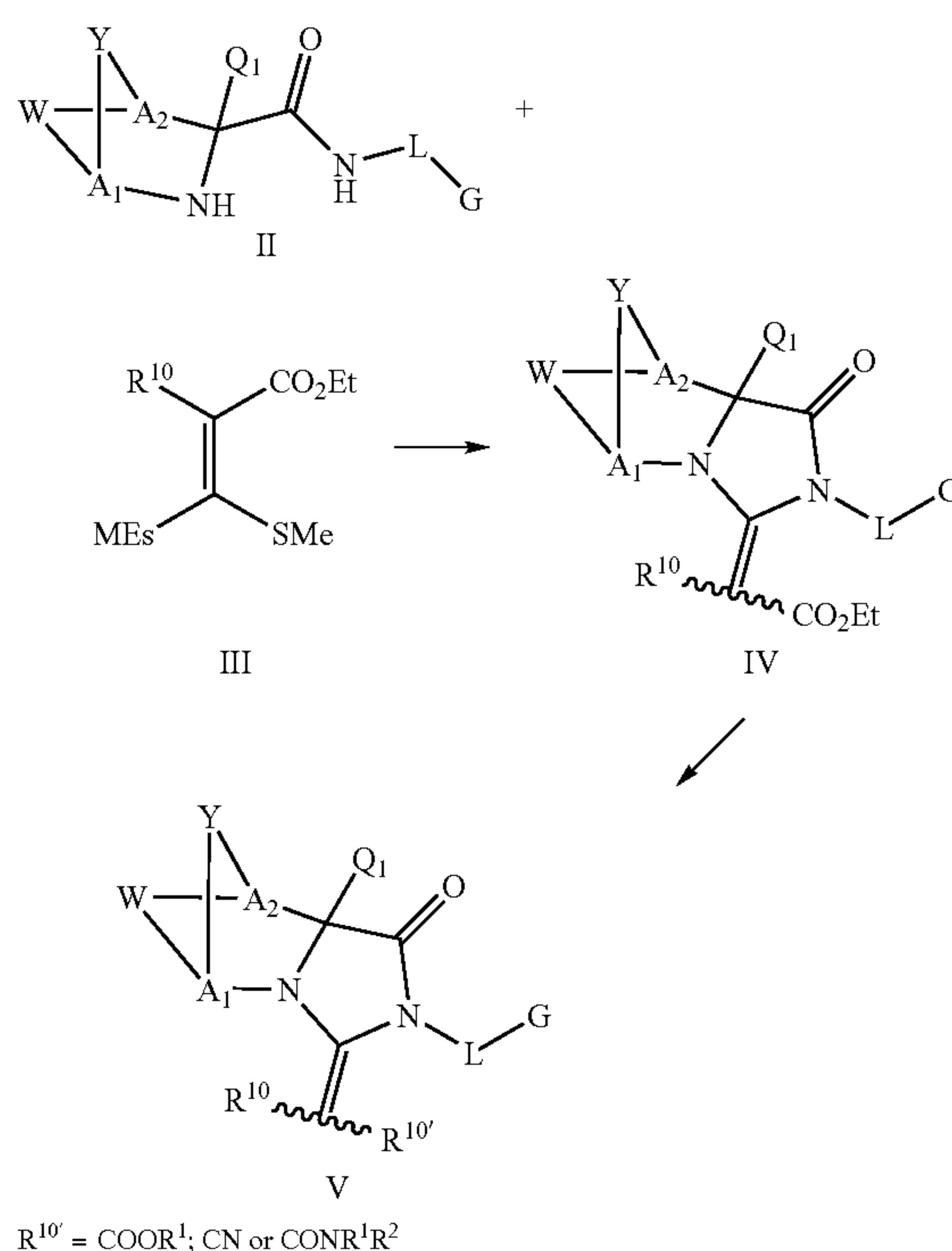
Scheme I
