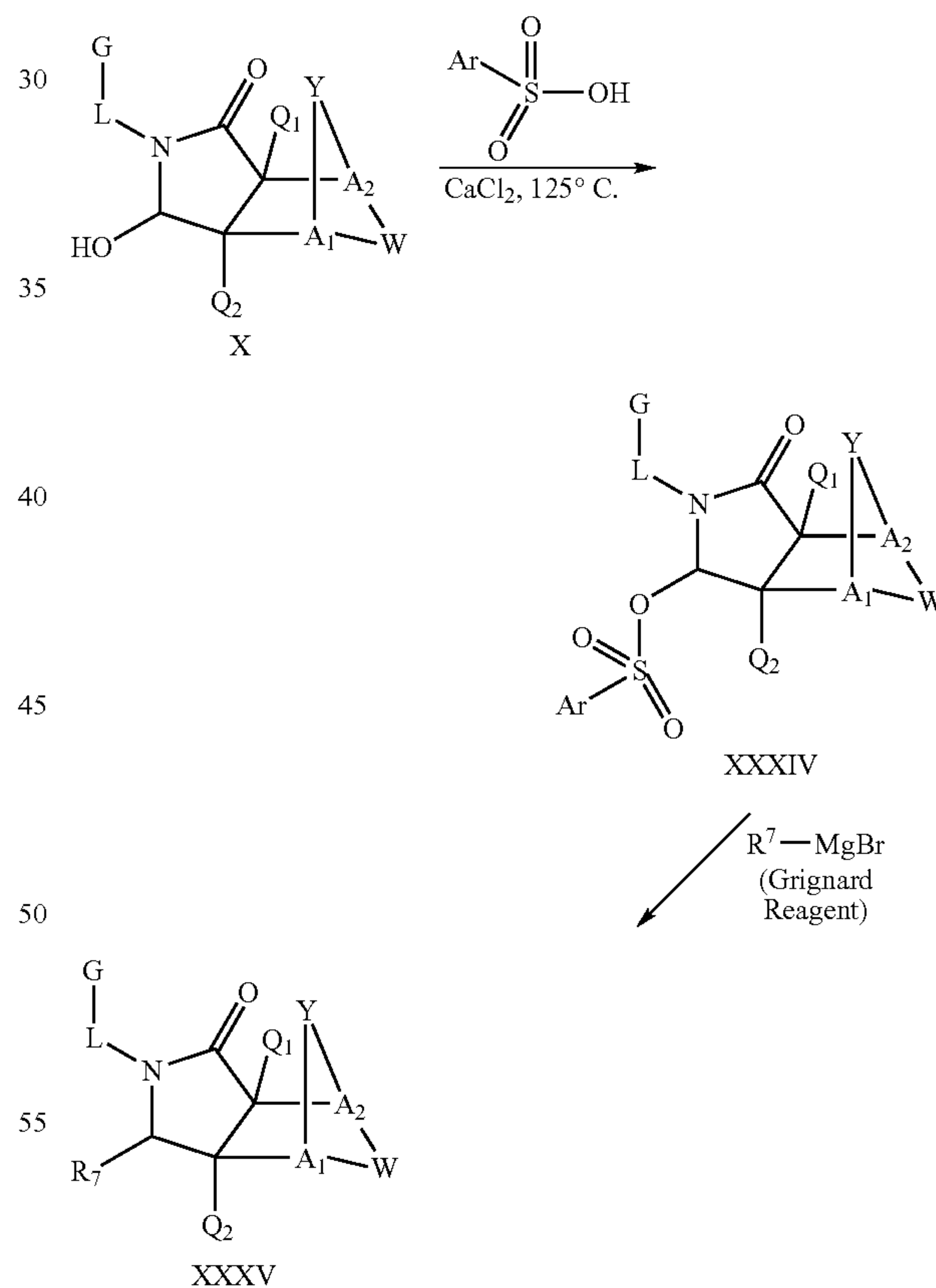
Scheme XVII
