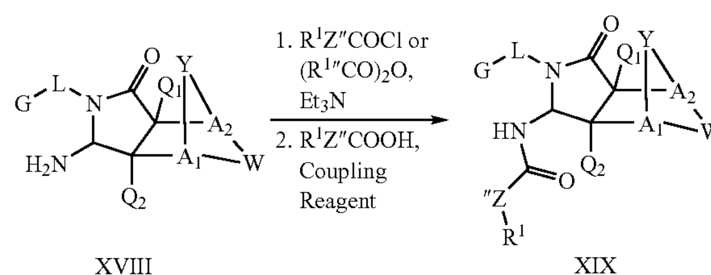
Scheme IX
