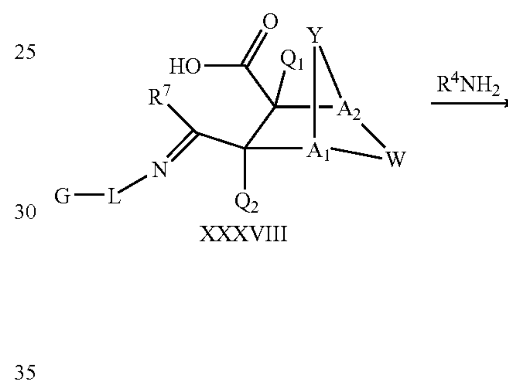
Scheme XX
