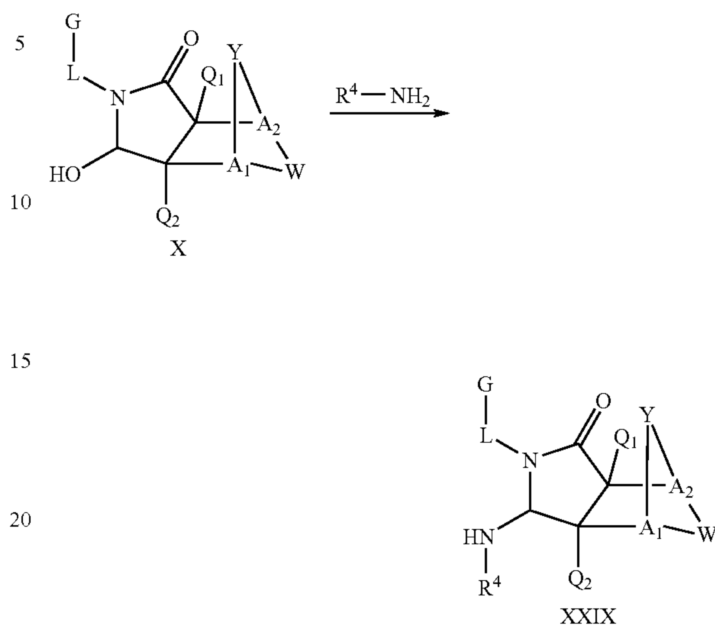
Scheme XIII
