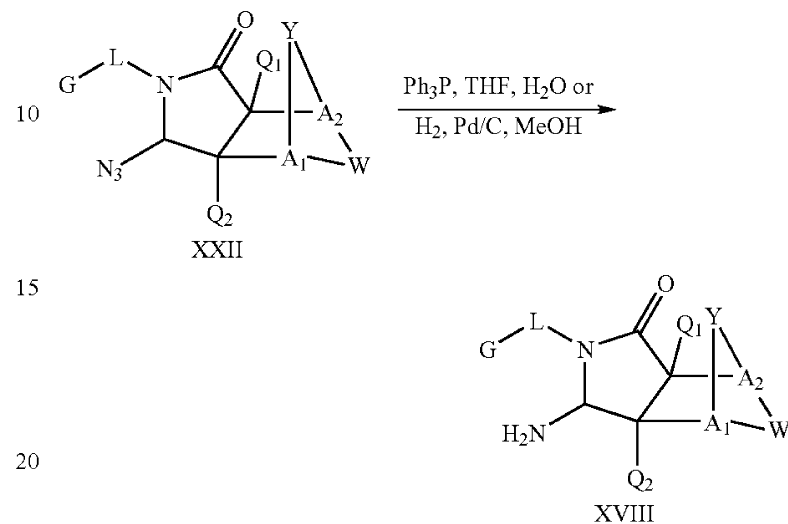
Scheme XI
