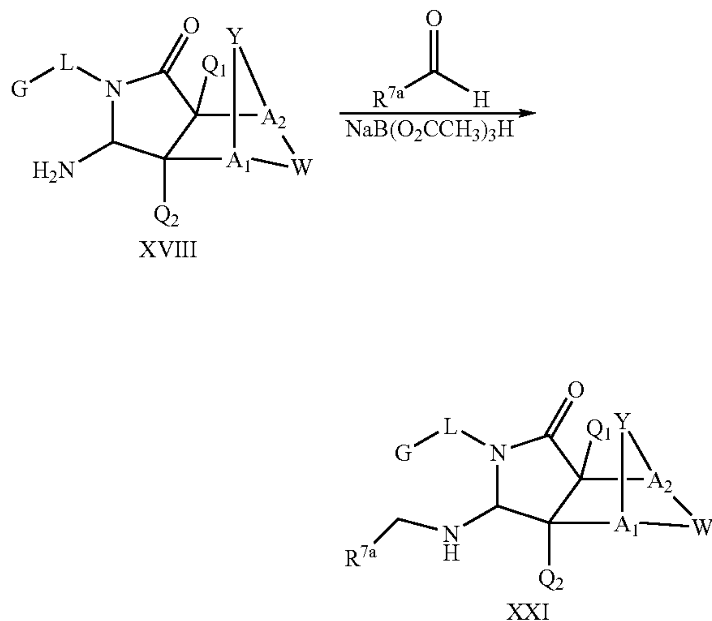
Scheme X
