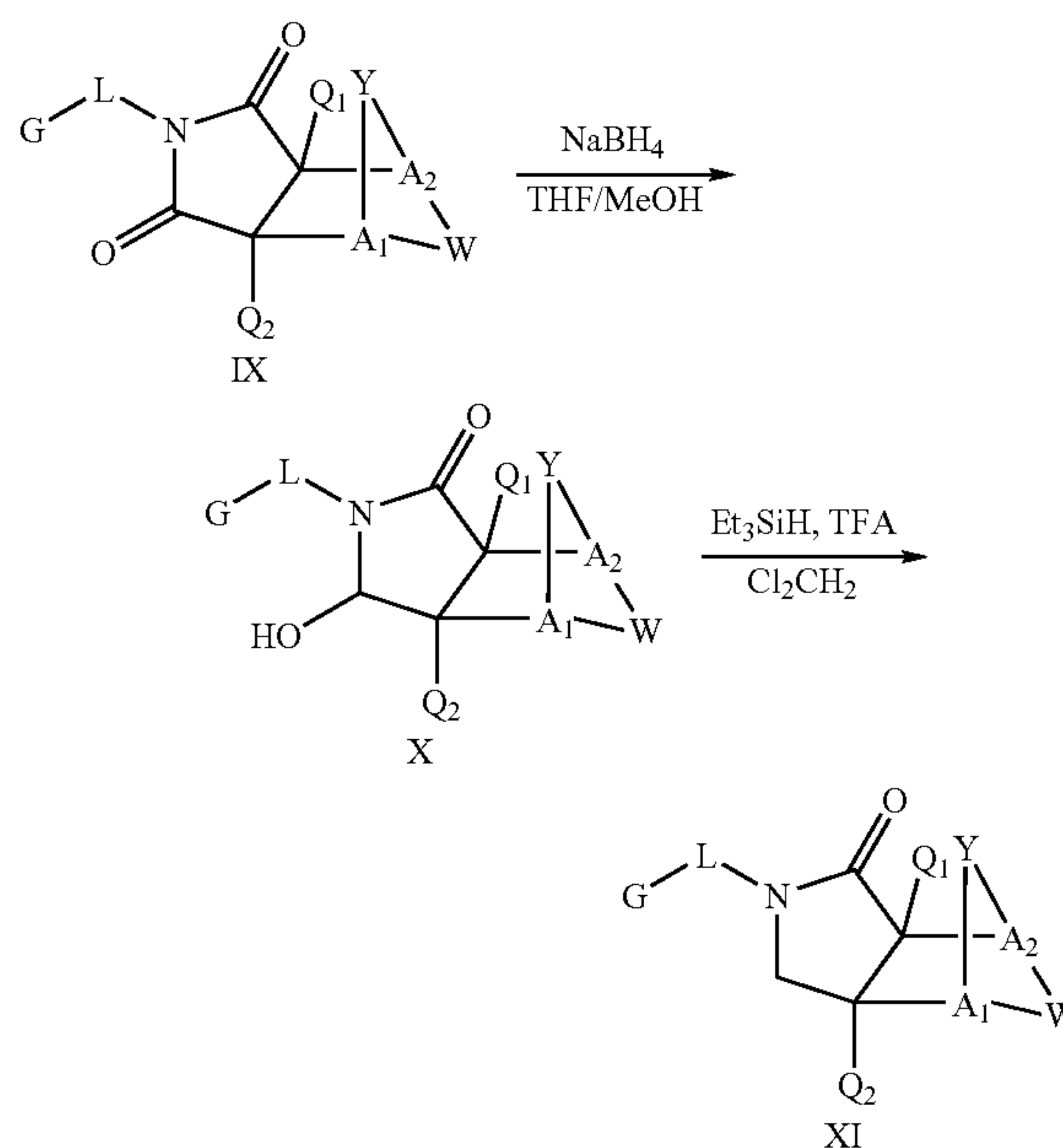
Scheme III
