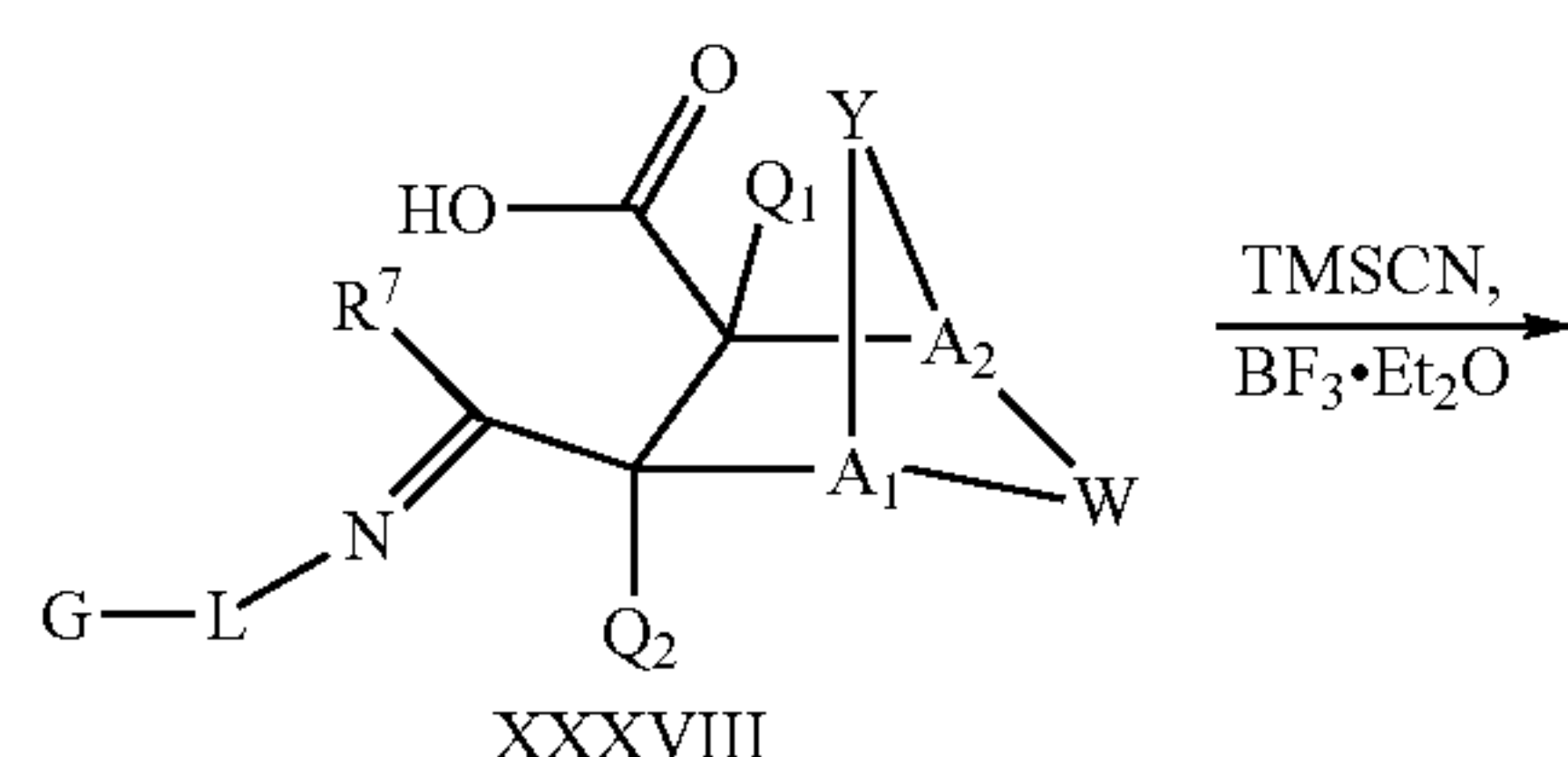
Scheme XIX
