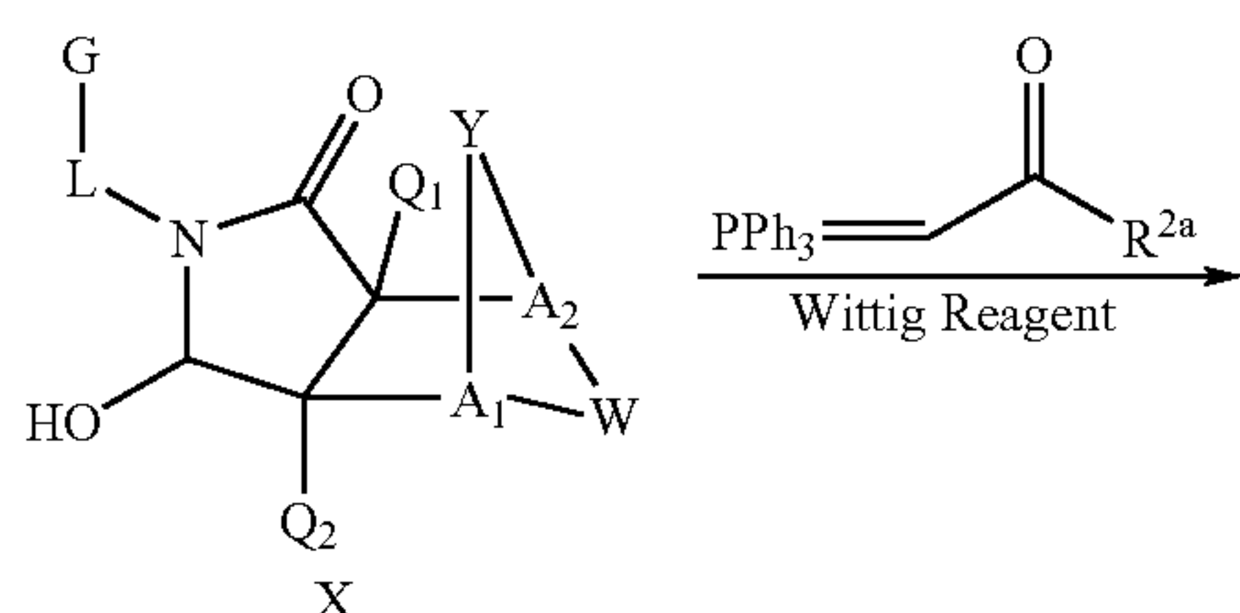
Scheme XVI
