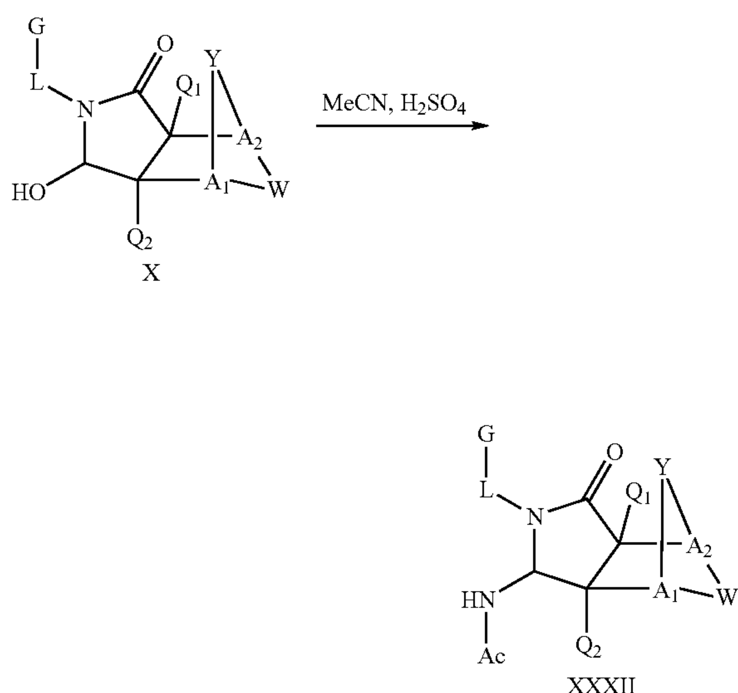
Scheme XV
