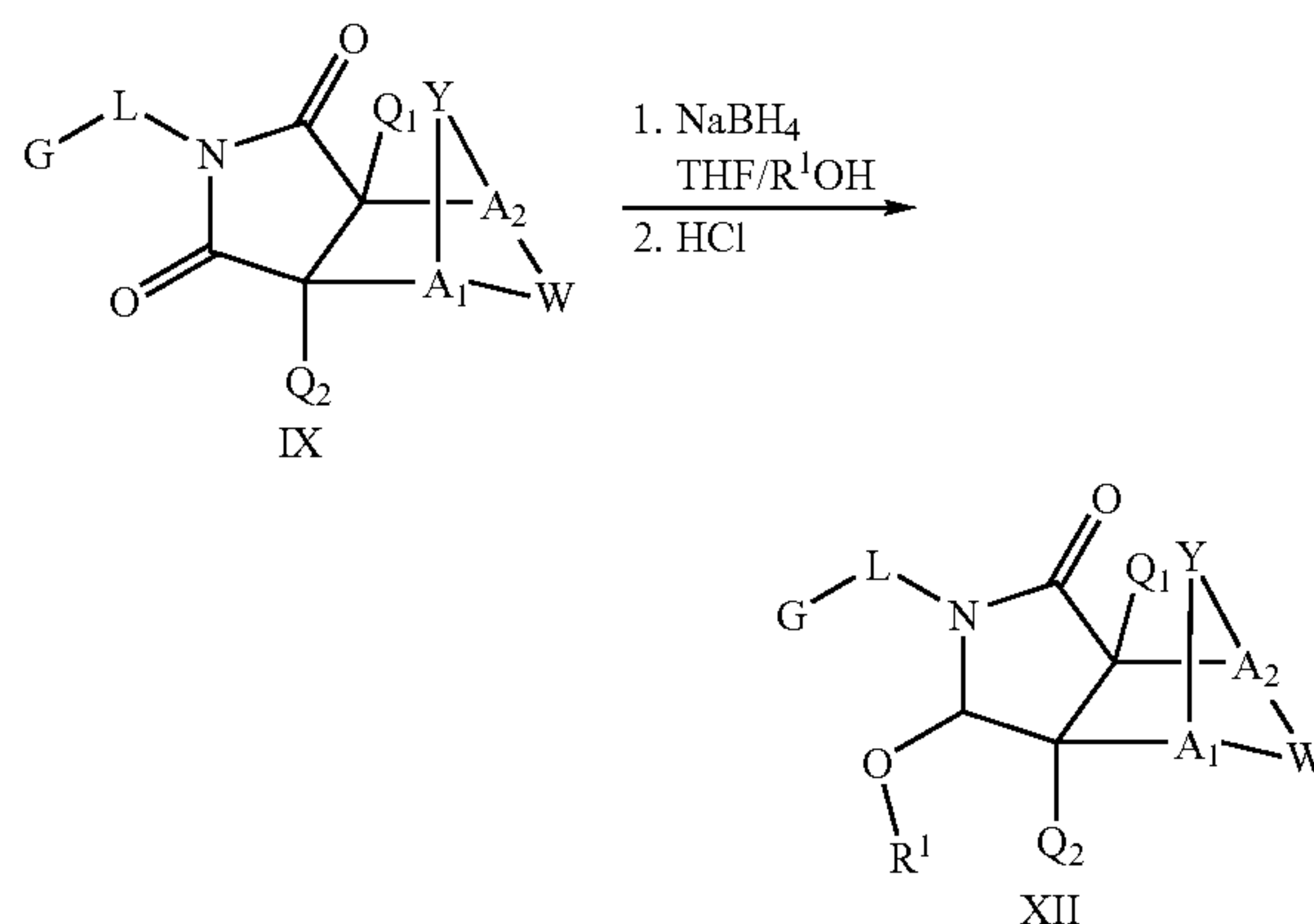
Scheme IV
