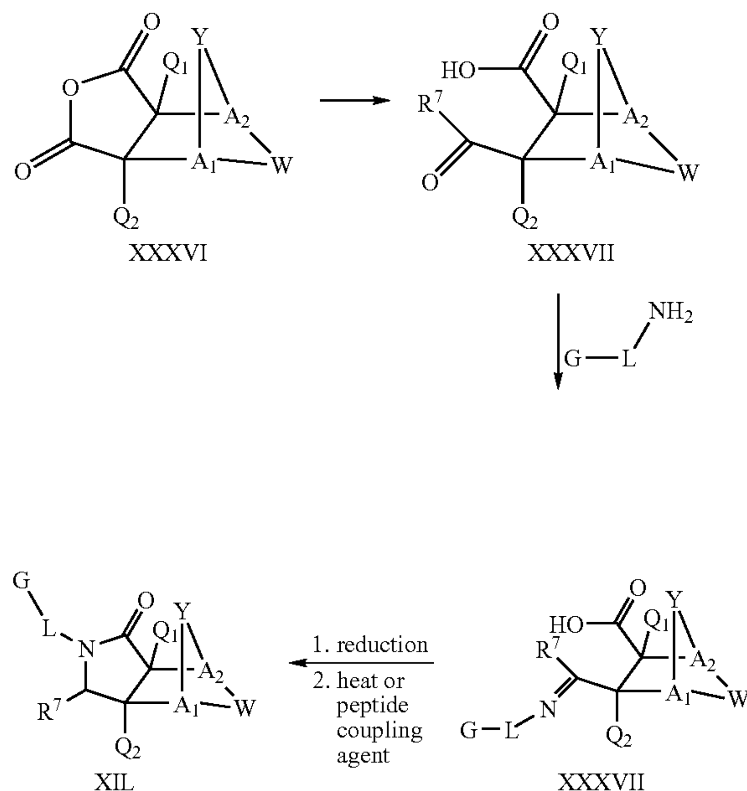
Scheme XVIII
