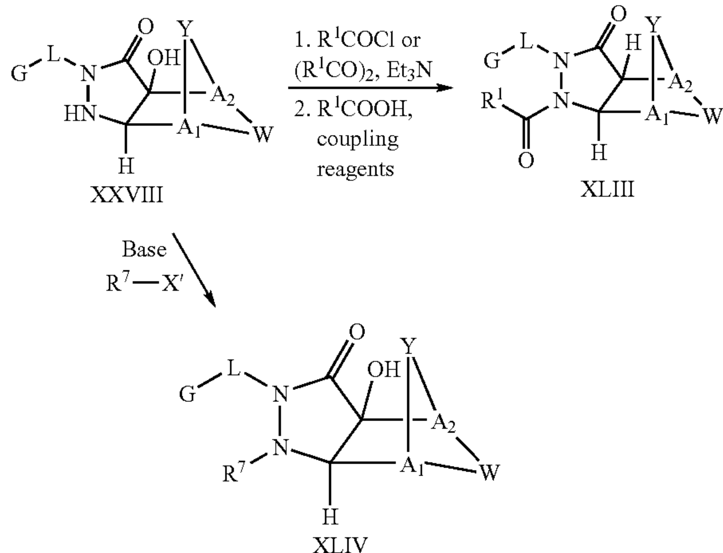
Scheme XXII
