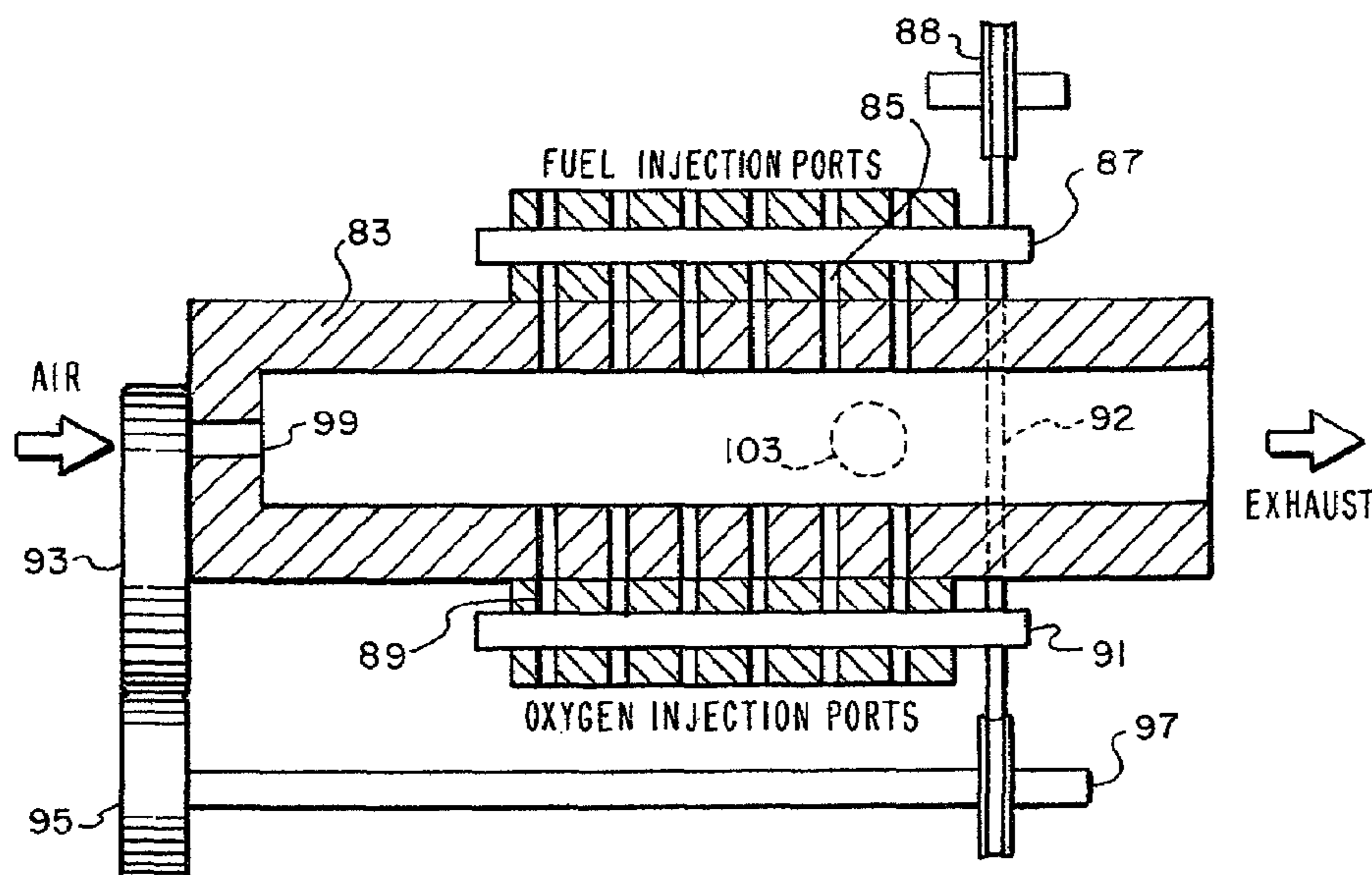
PULSED DETONATION ENGINE
