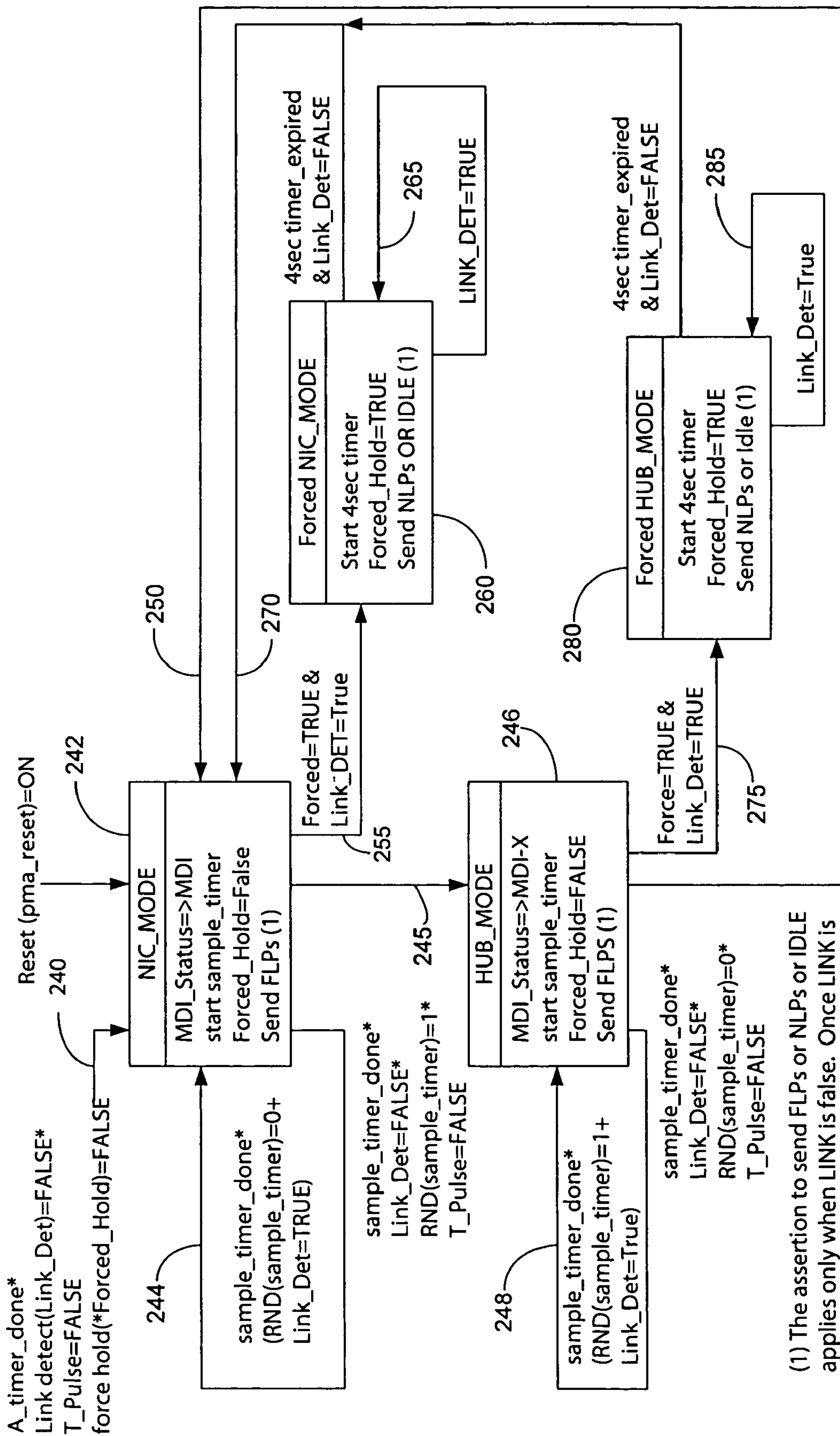
Forced Mode Auto-MDIX State Machine
