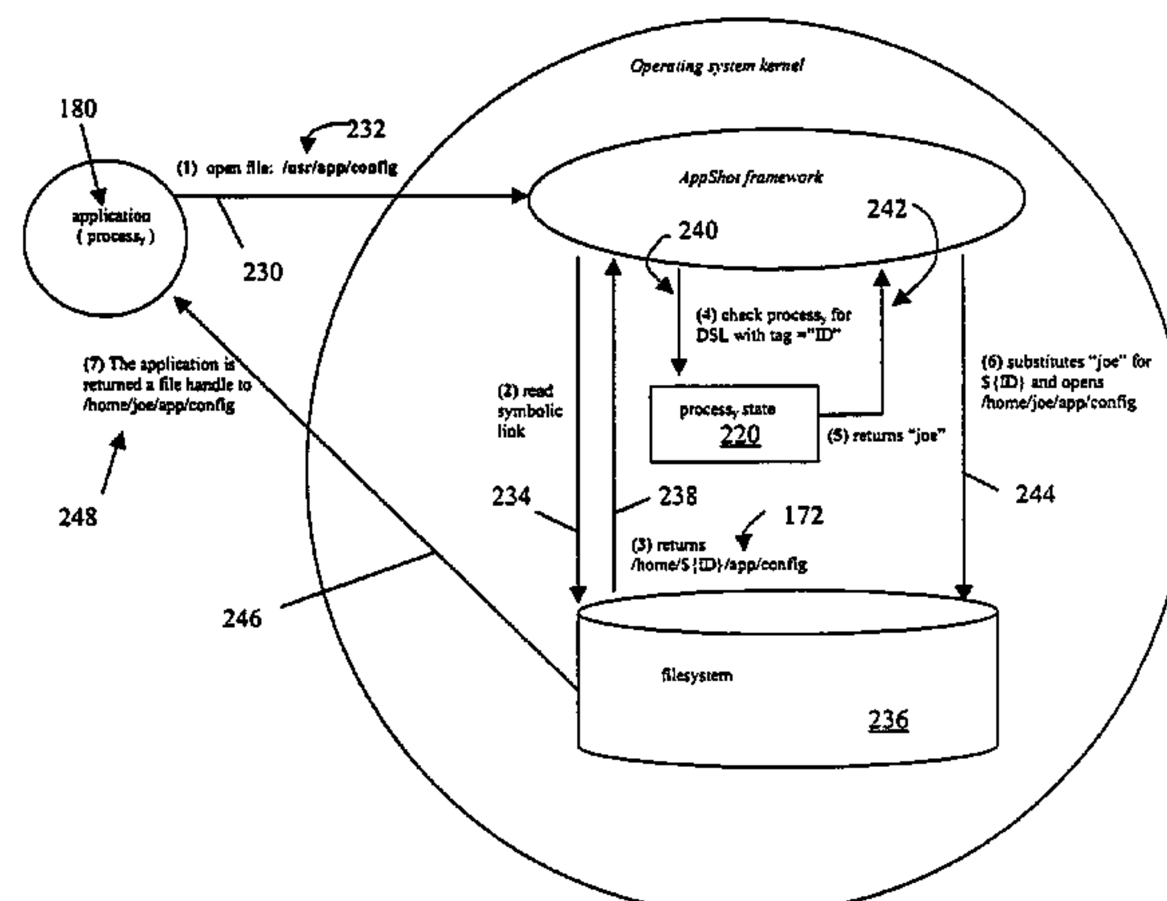
Resolution of a dynamic symbolic link.
