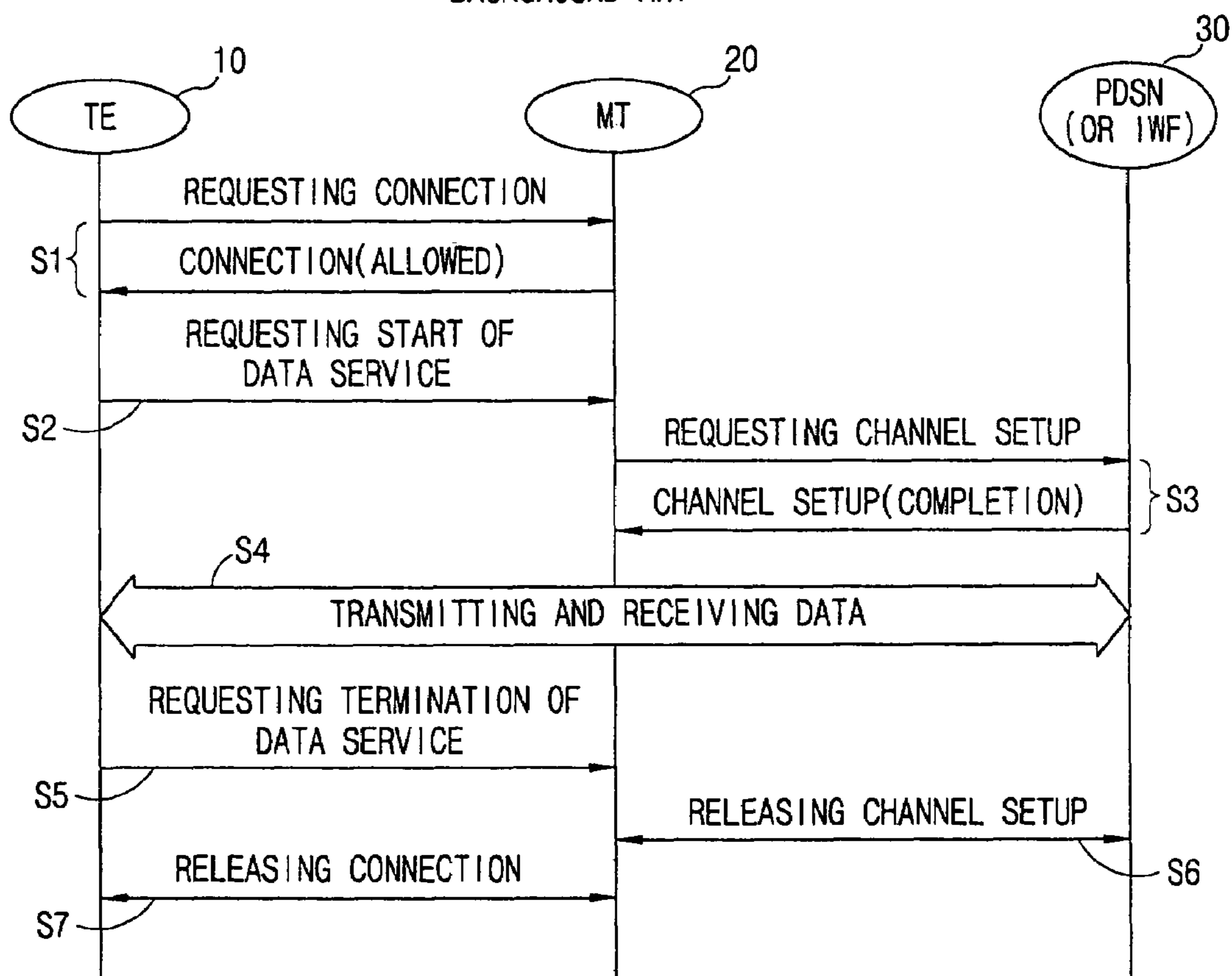
FIG. 2 BACKGROUND ART
