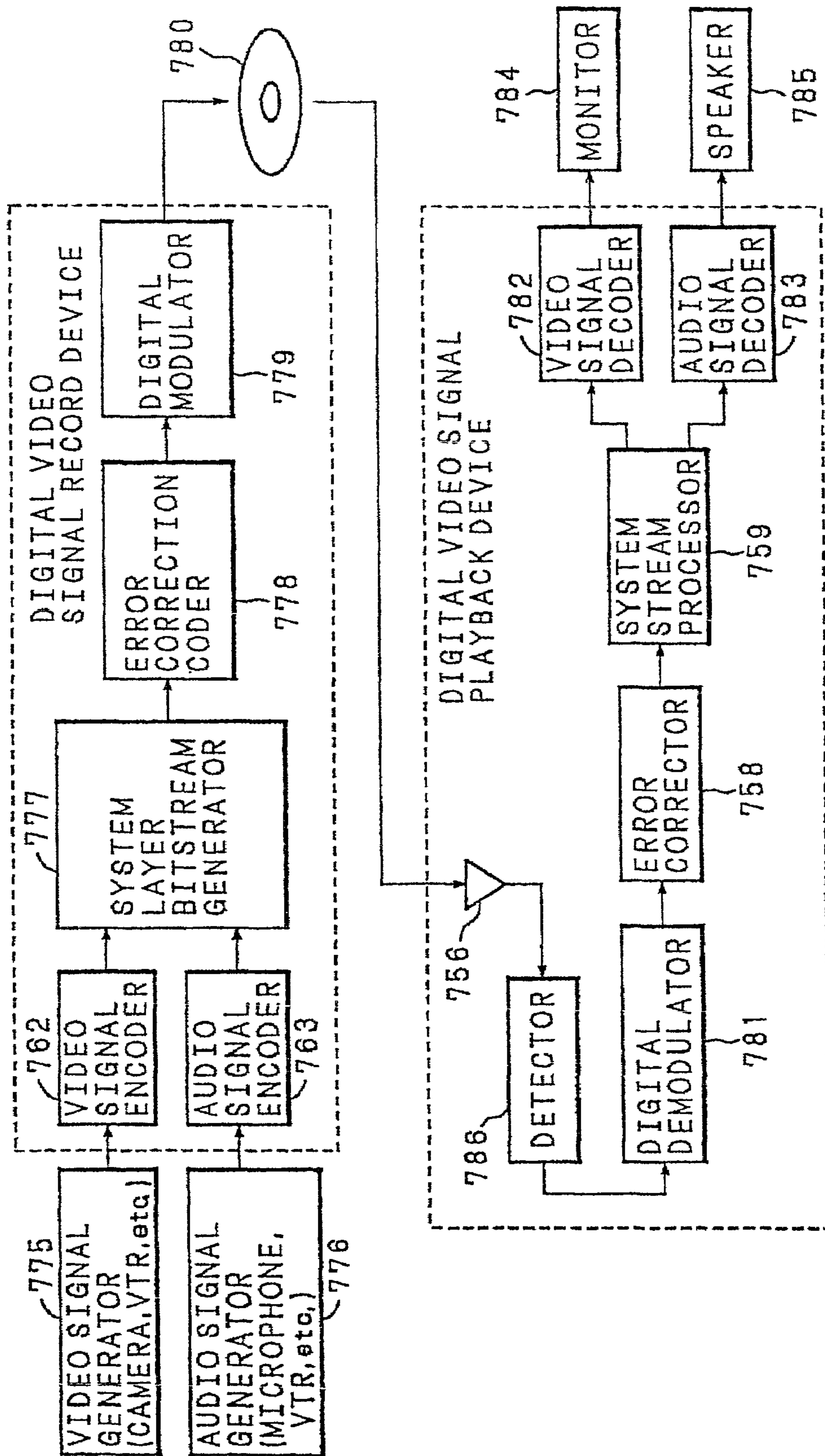
FIG. 10 PRIOR ART
