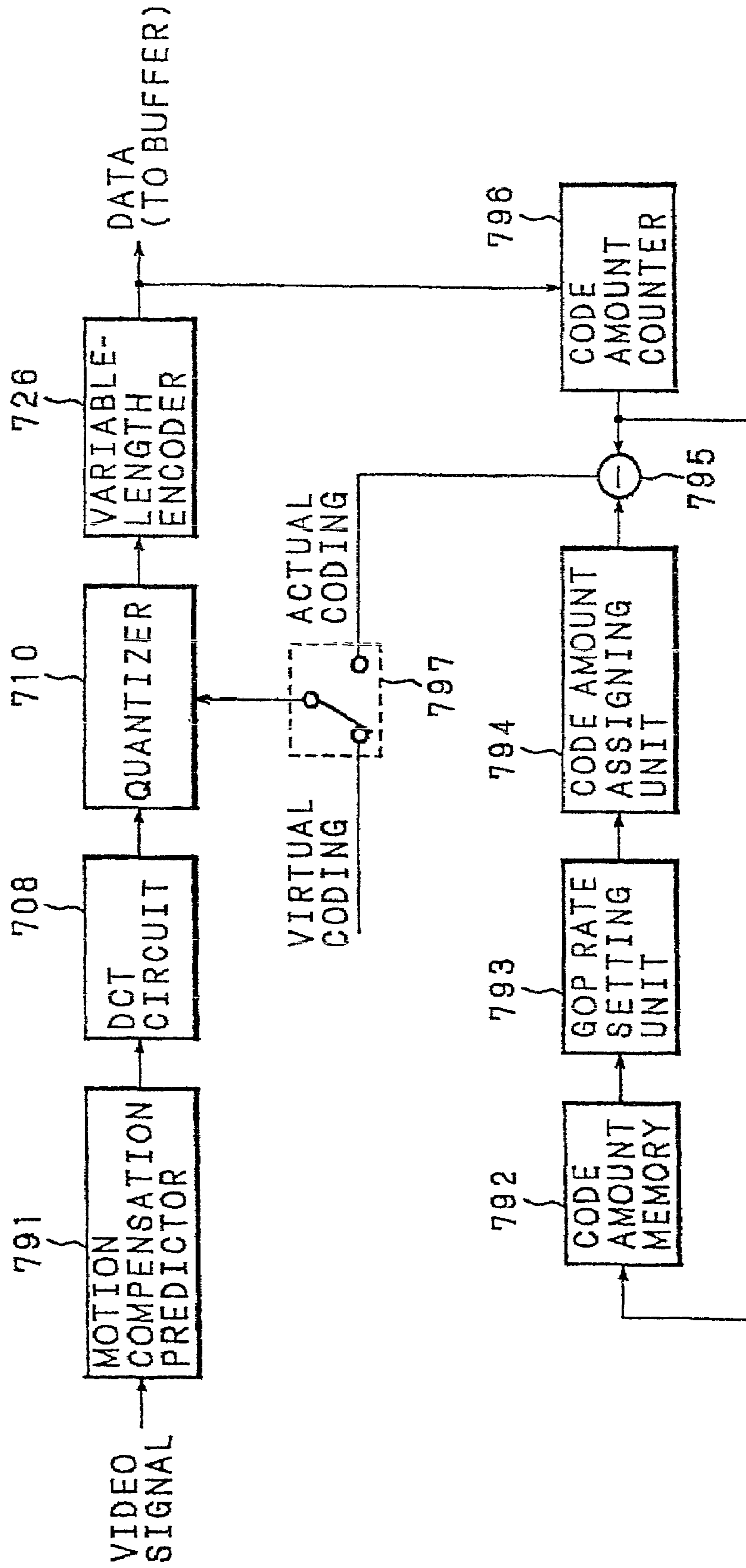
FIG. 14 PRIOR ART
