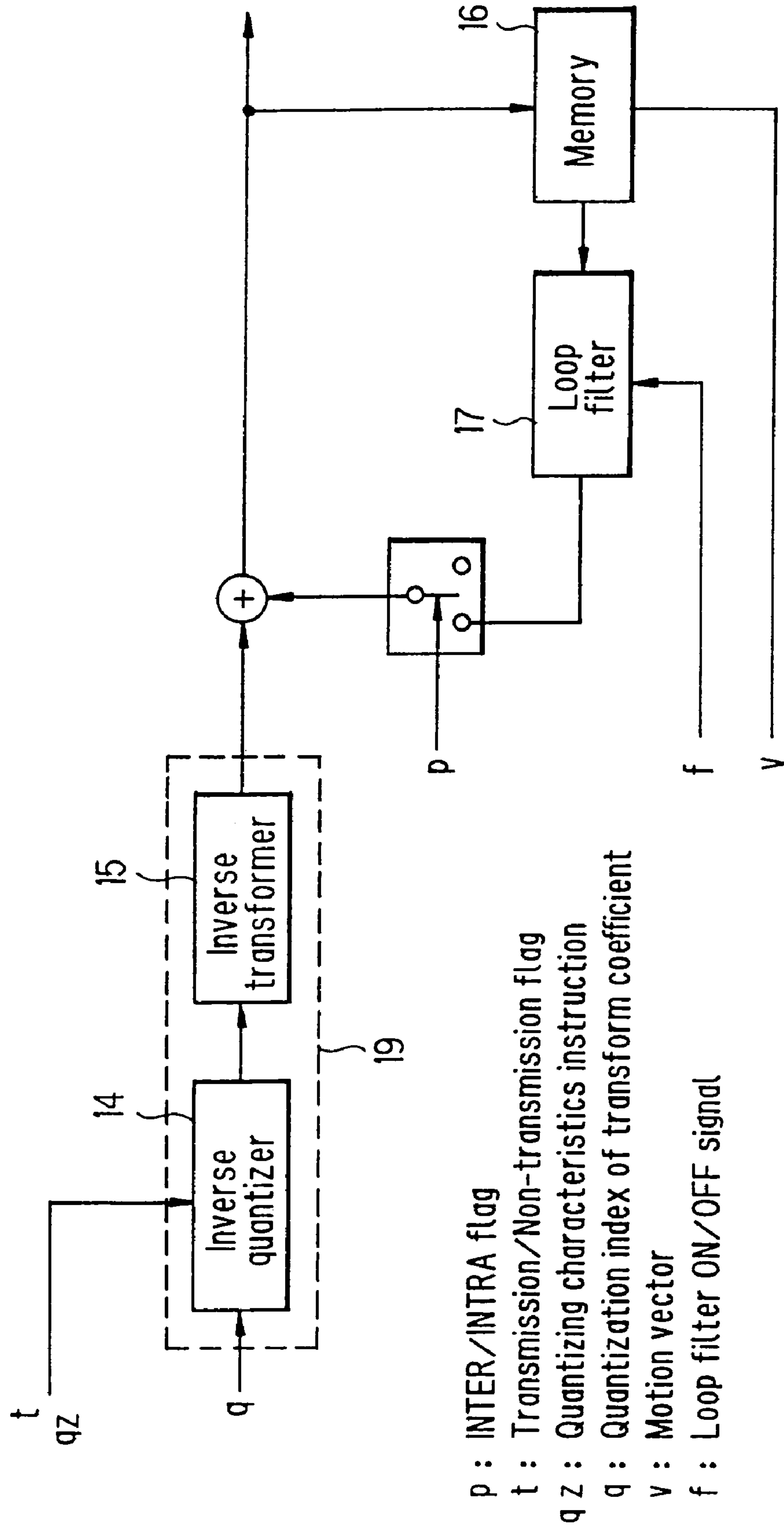
FIG. 3 PRIOR ART
