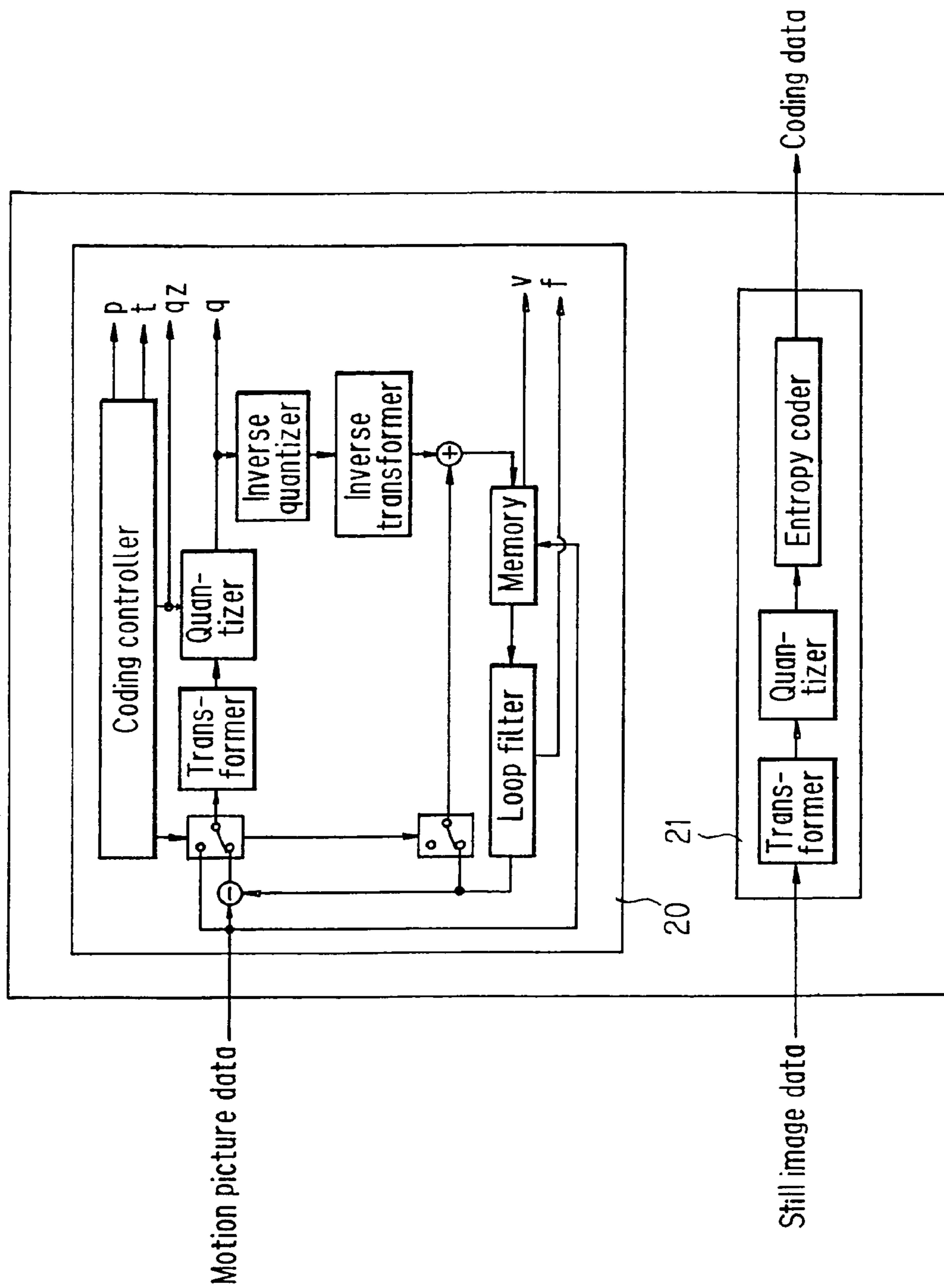
FIG. 4 PRIOR ART
