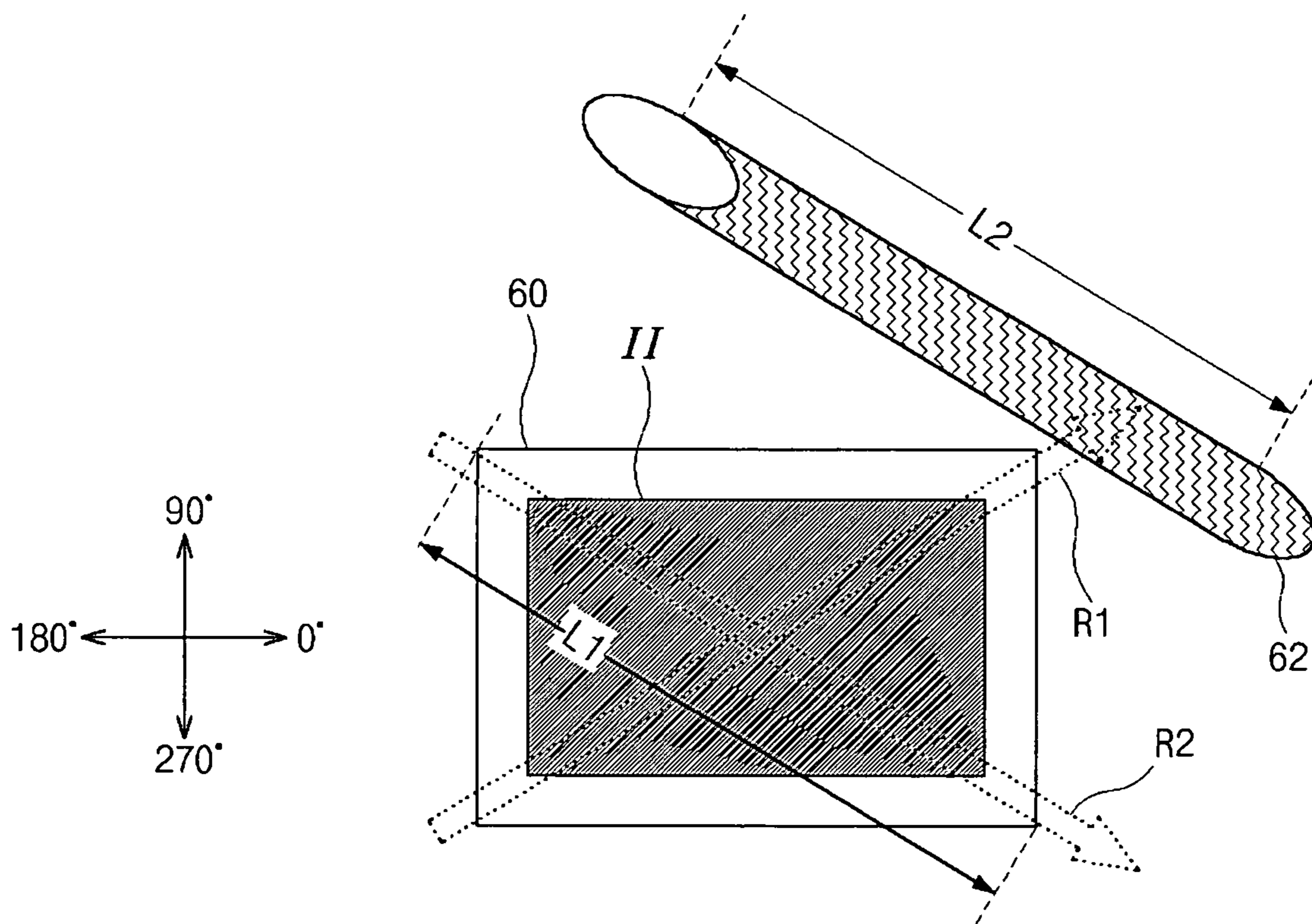
FIG. 2 (RELATED ART)
