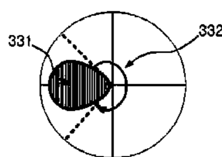
BACK-SUPPRESSED SIGNAL BEAM PATTERN DIAGRAM
