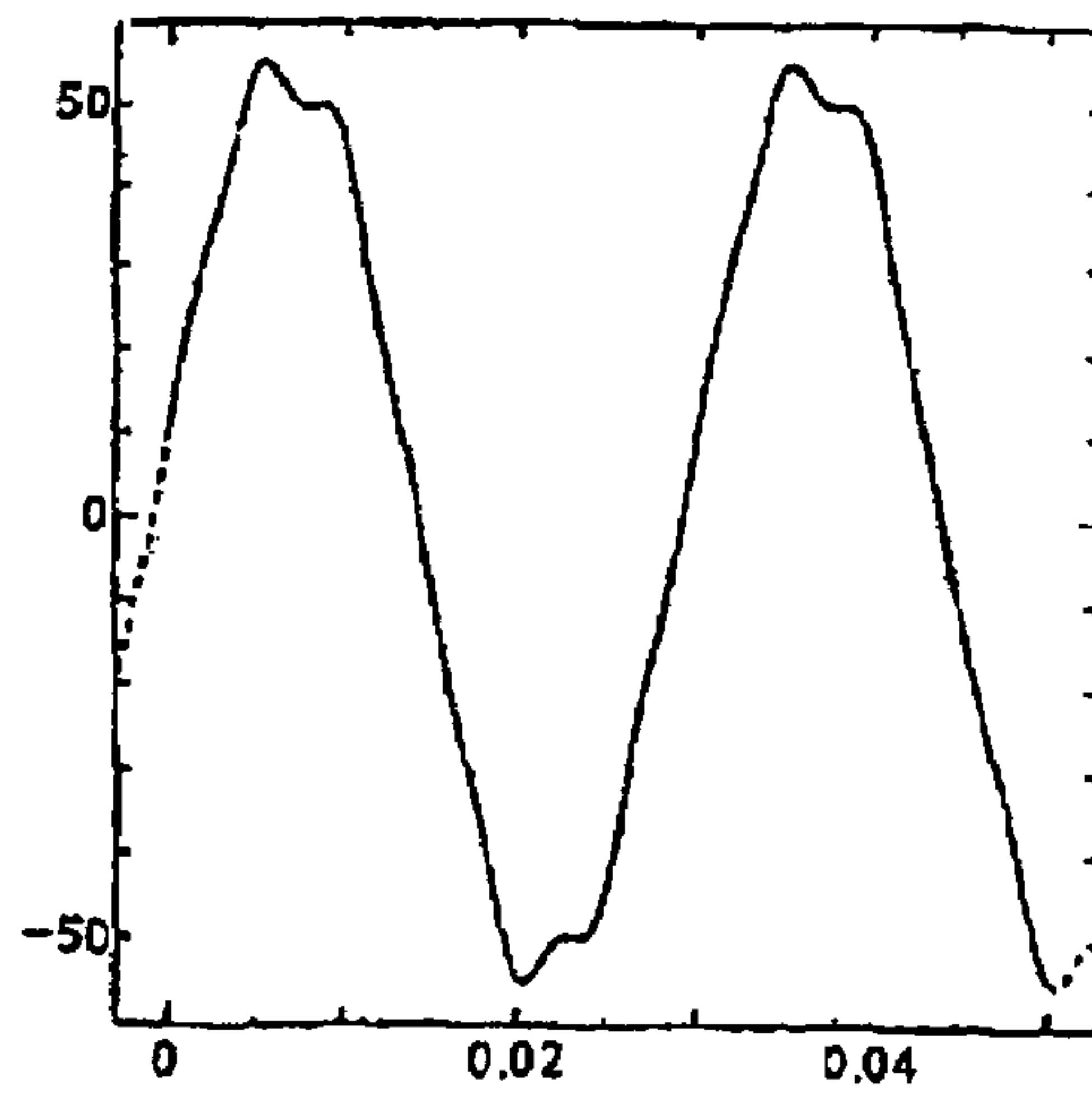
PHASE CURRENT WHEN I_d=10 [A] (C)
