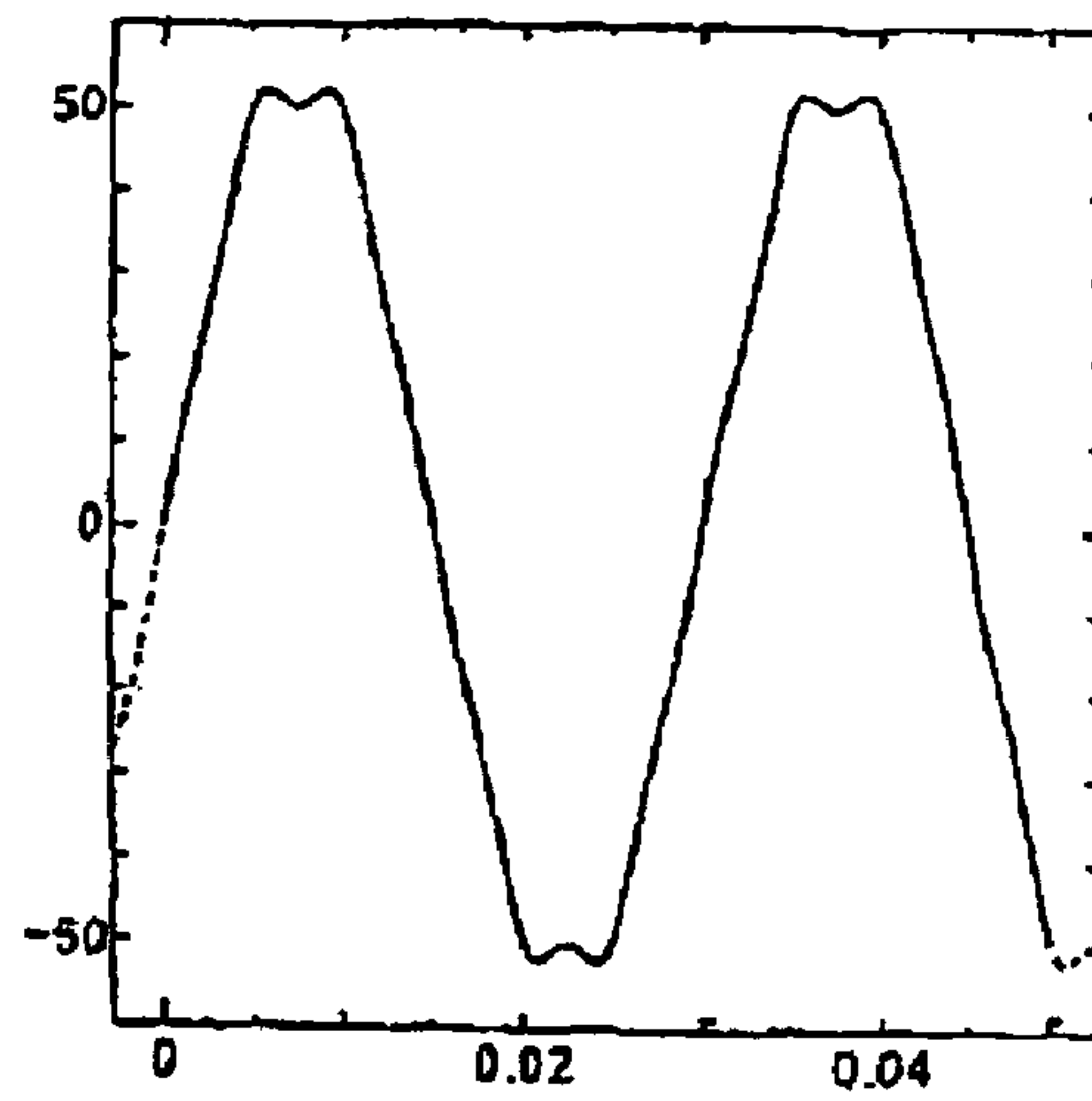
PHASE CURRENT WHEN I_d=0 [A] (B)
