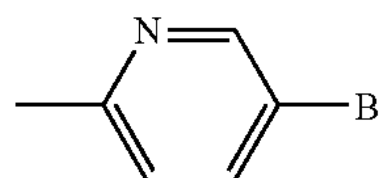
2-pyridyl
