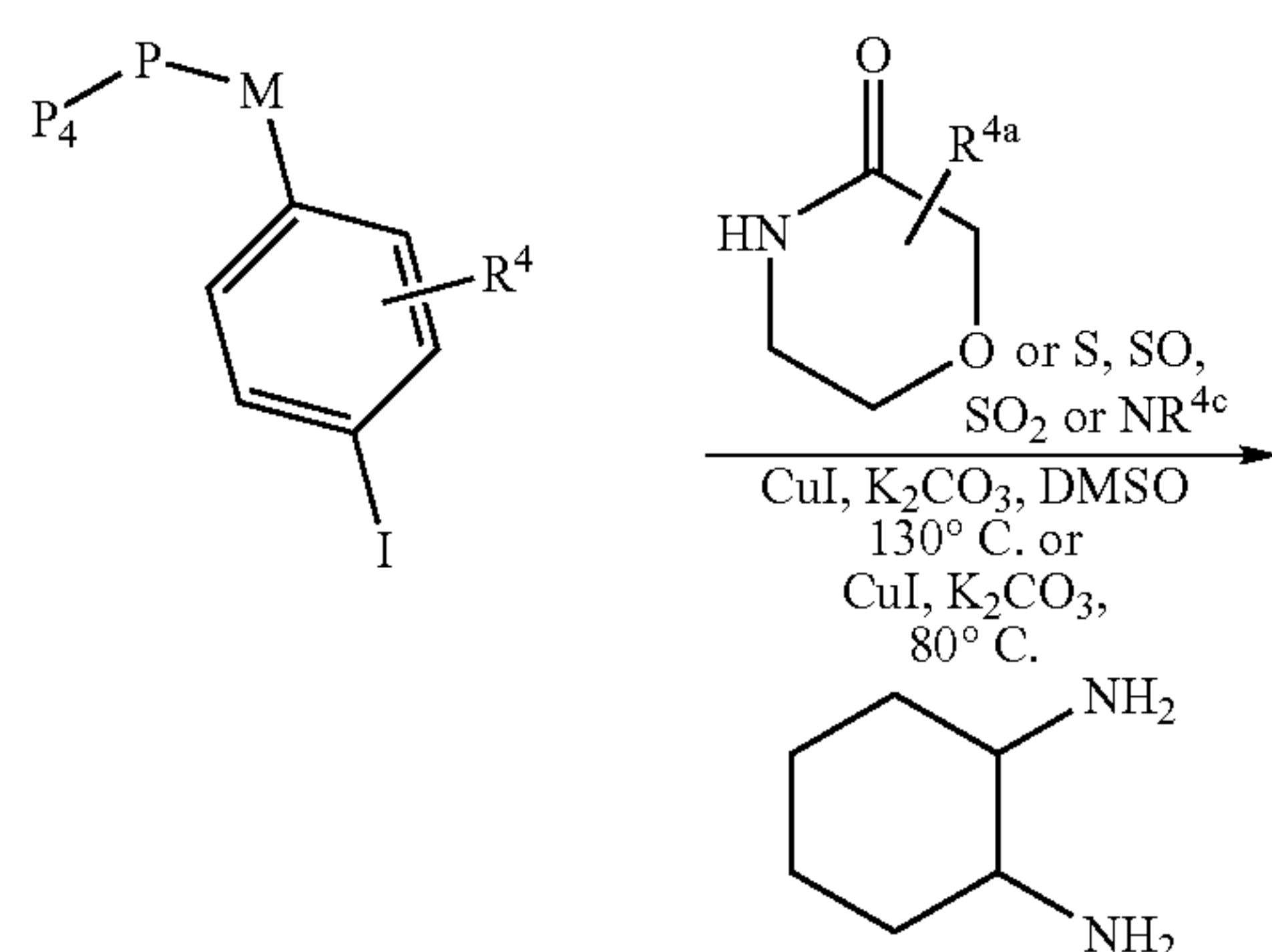
Scheme 11
