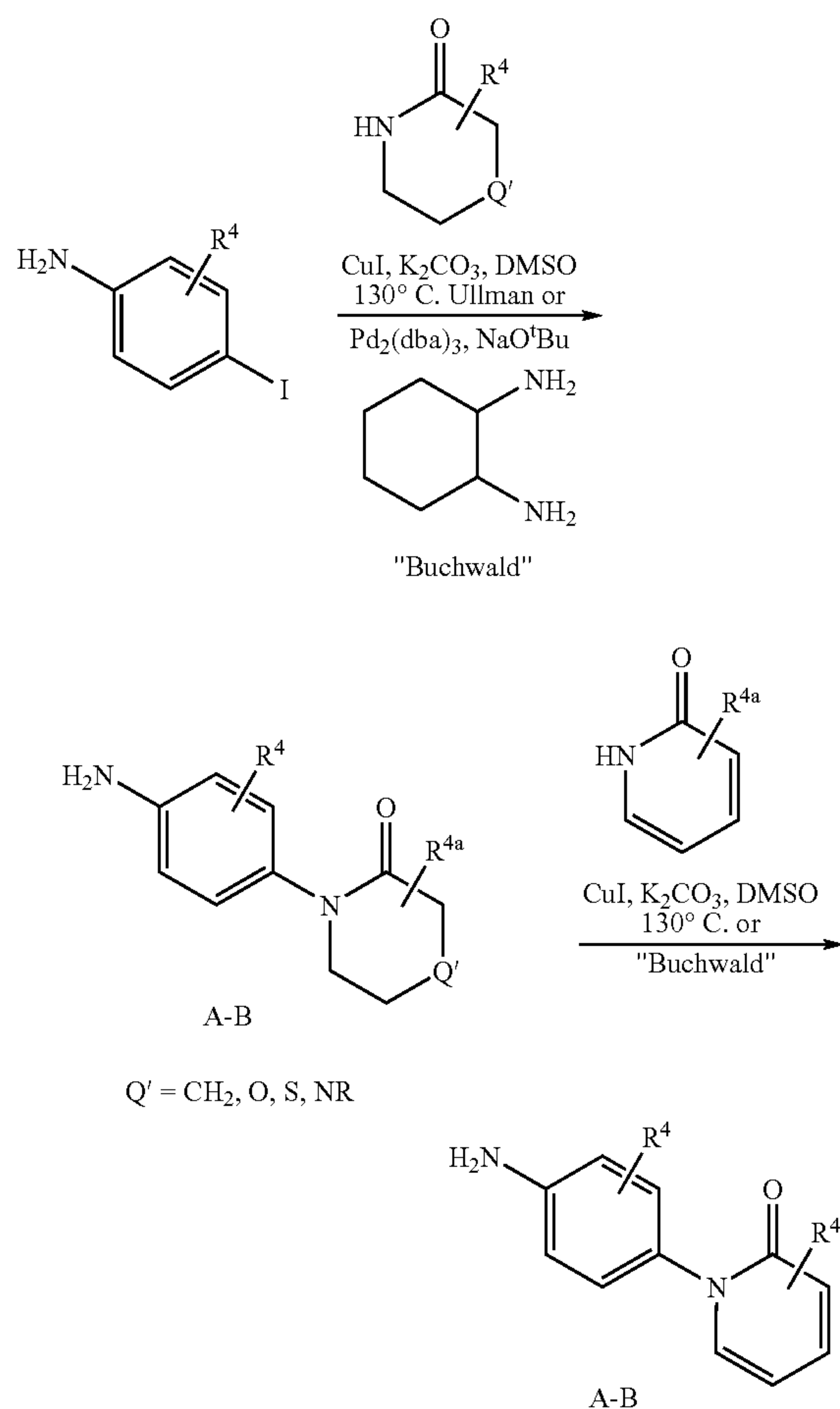
Scheme 2
