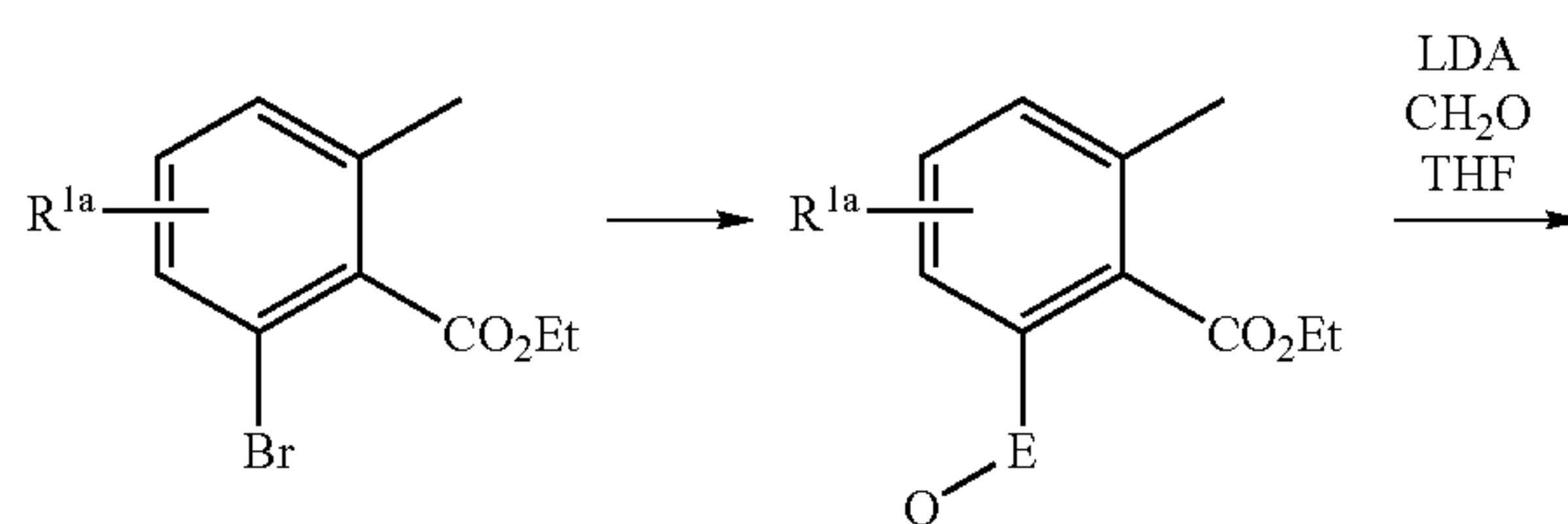
Scheme 24
