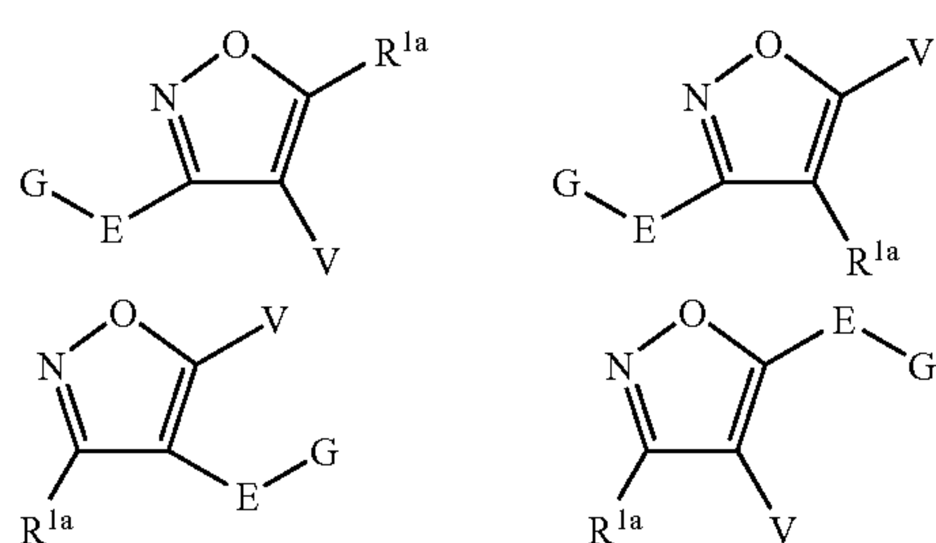
Scheme 17
