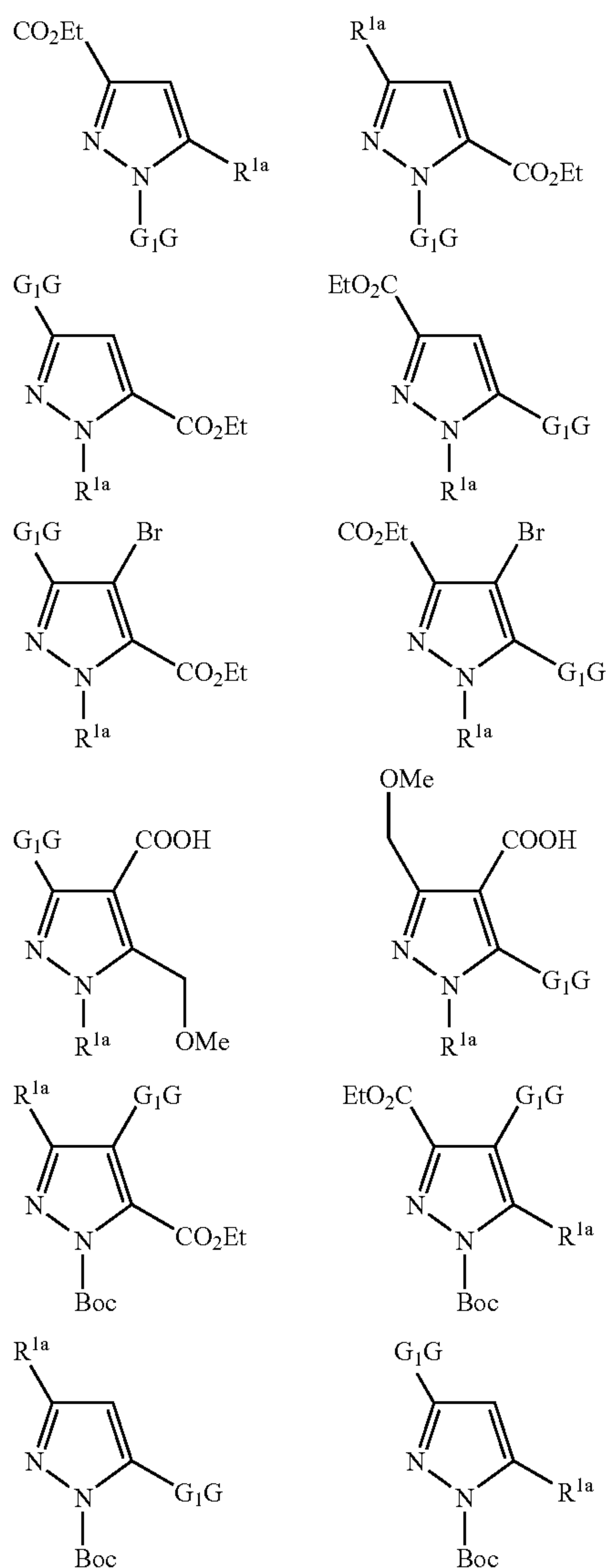
Scheme 16
