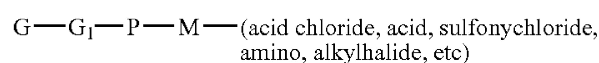
Formula II
