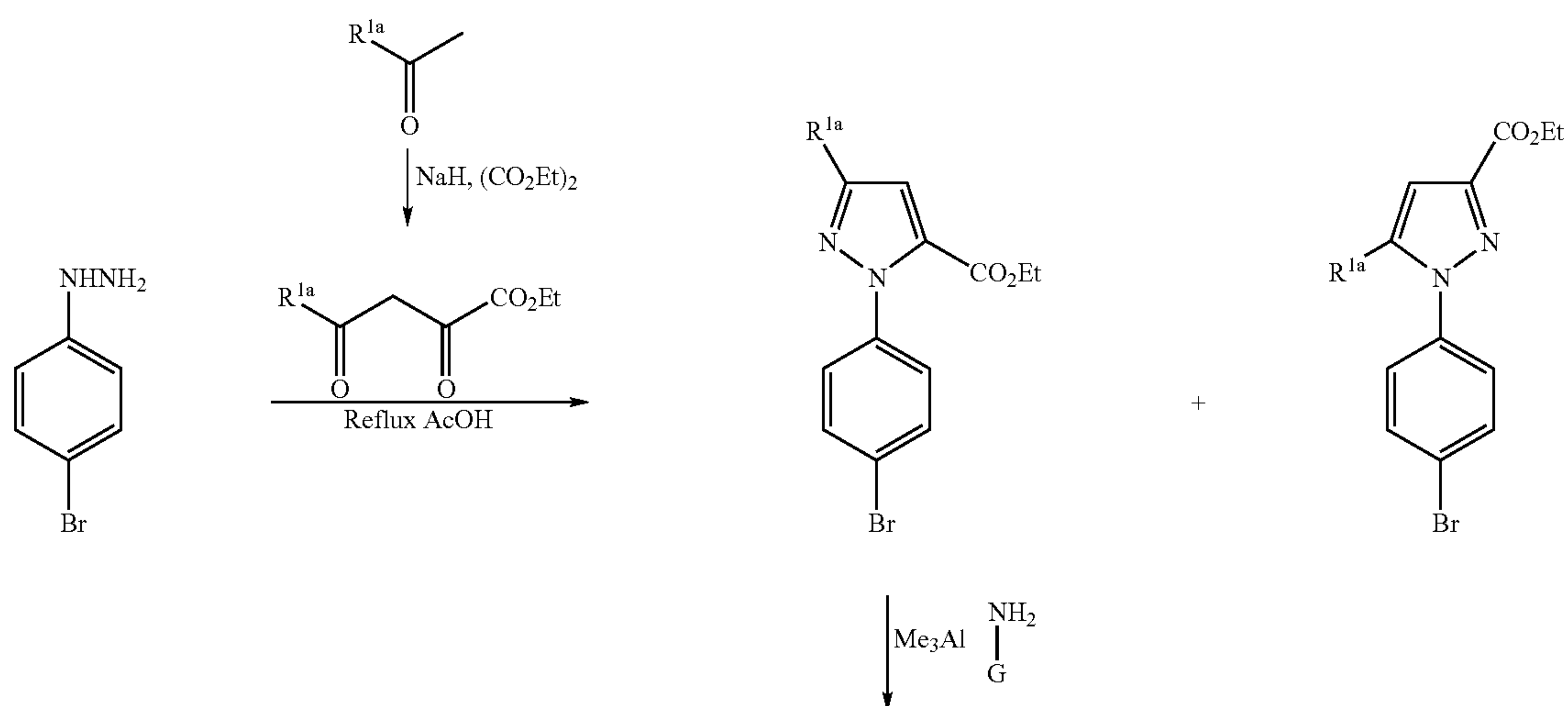
Scheme 22
