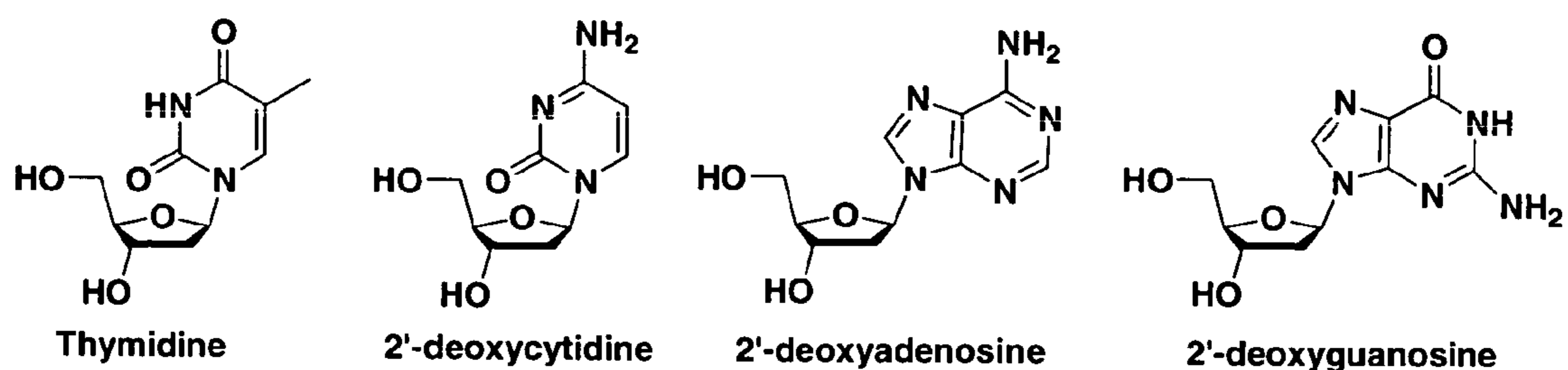
Representative Nucleosides
