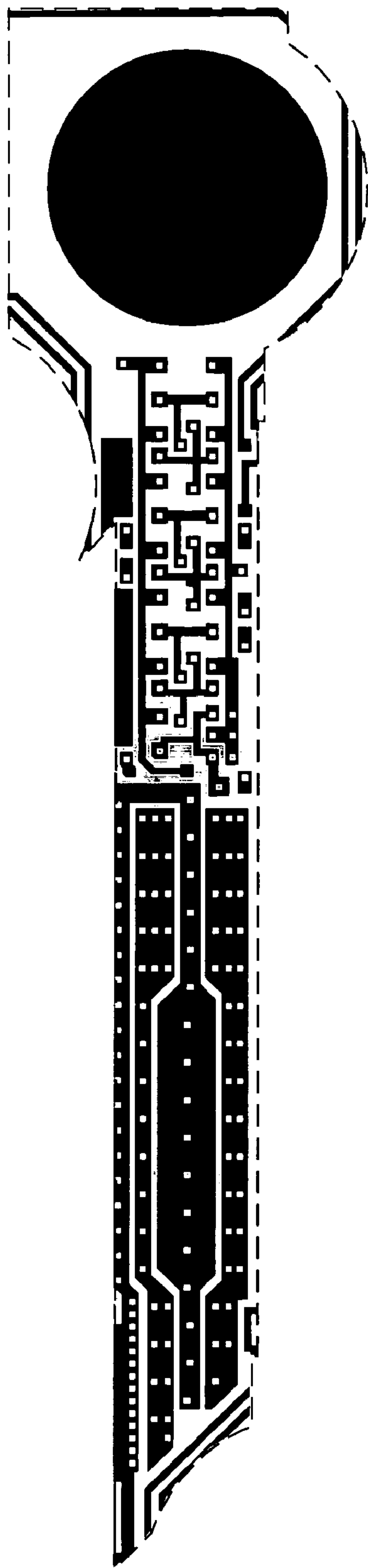
Metal 1 mask
