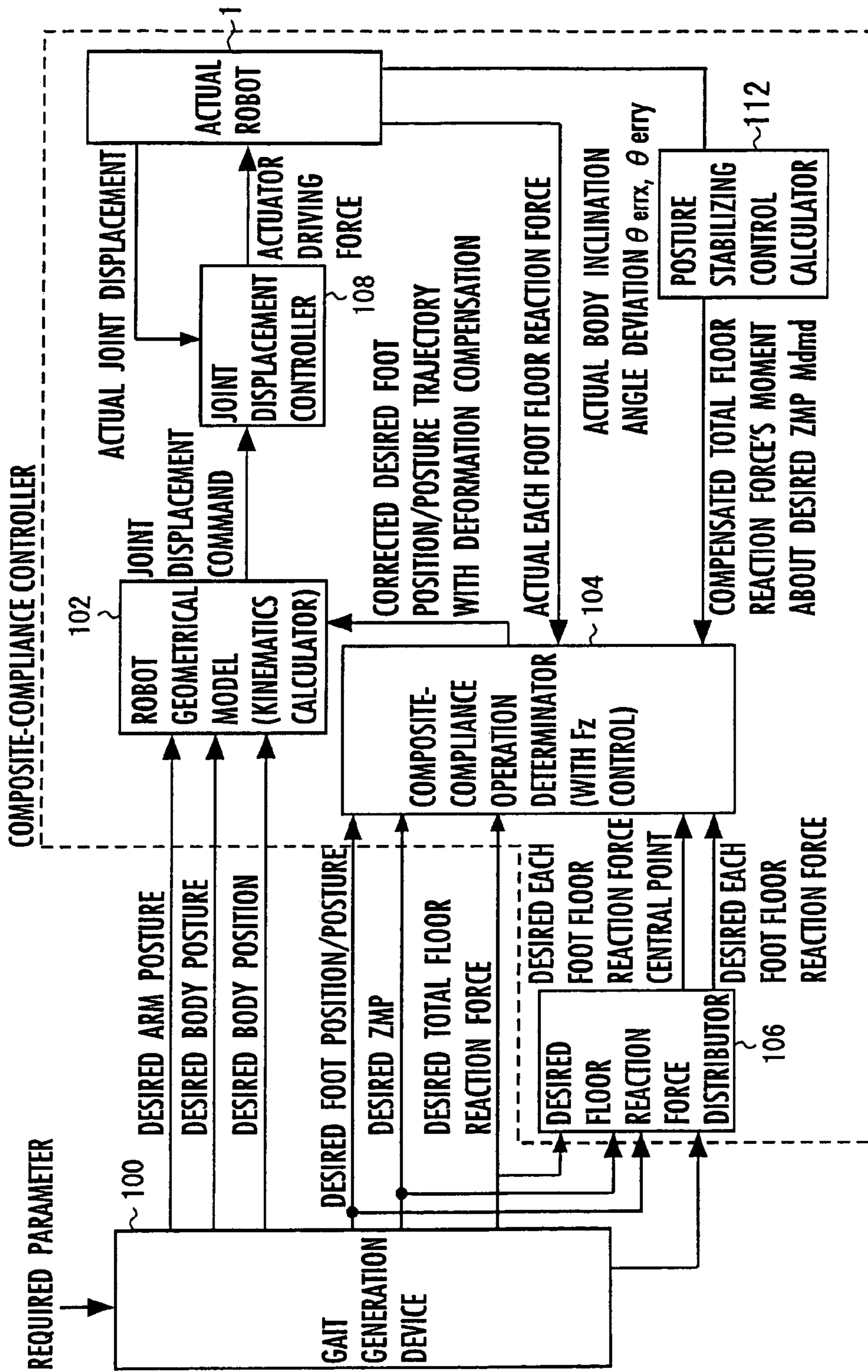
FIG.4 ( FUNCTIONAL BLOCK DIAGRAM OF LEGGED MOBILE ROBOT )
