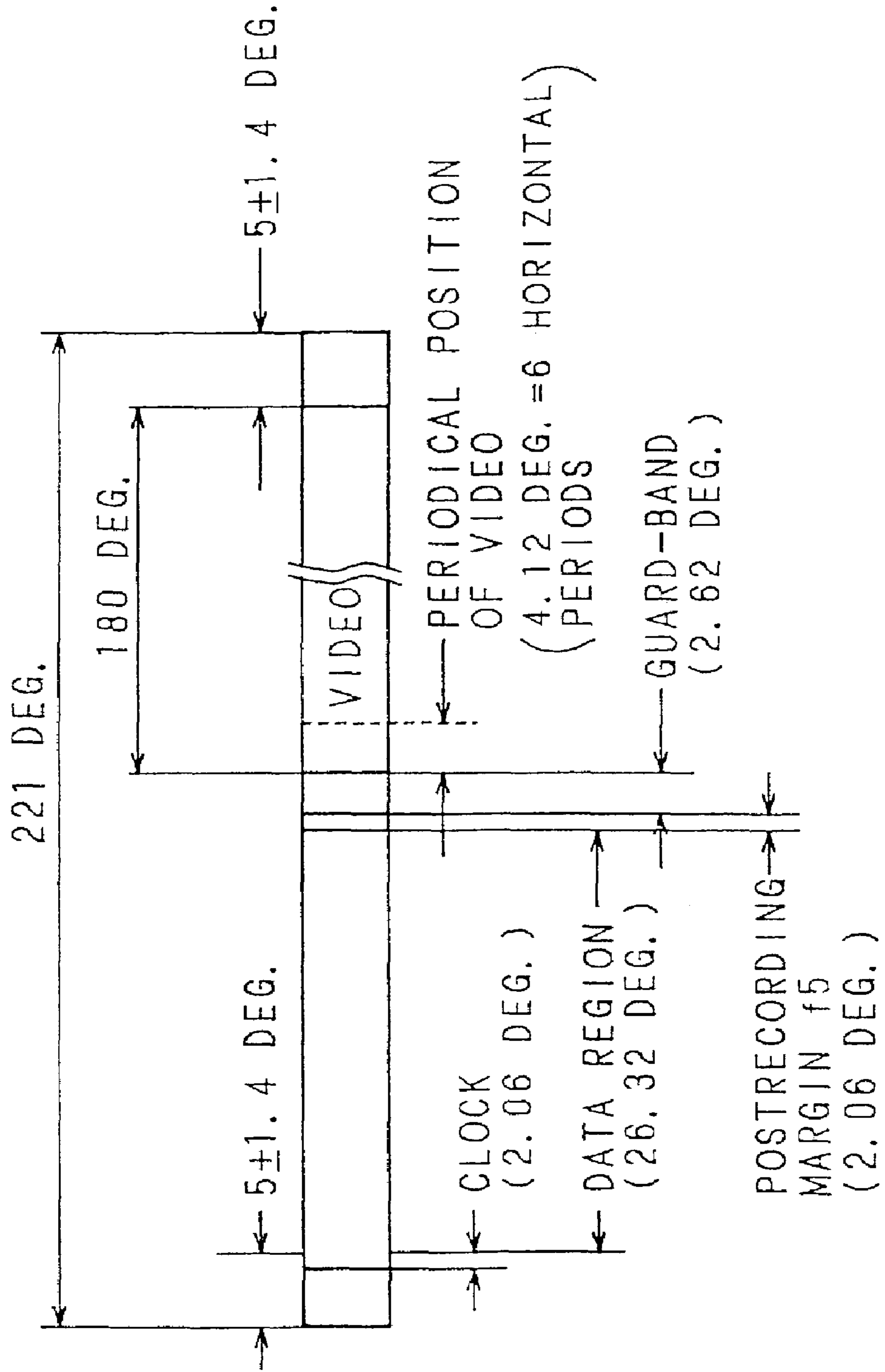
Fig. 10 Prior Art
