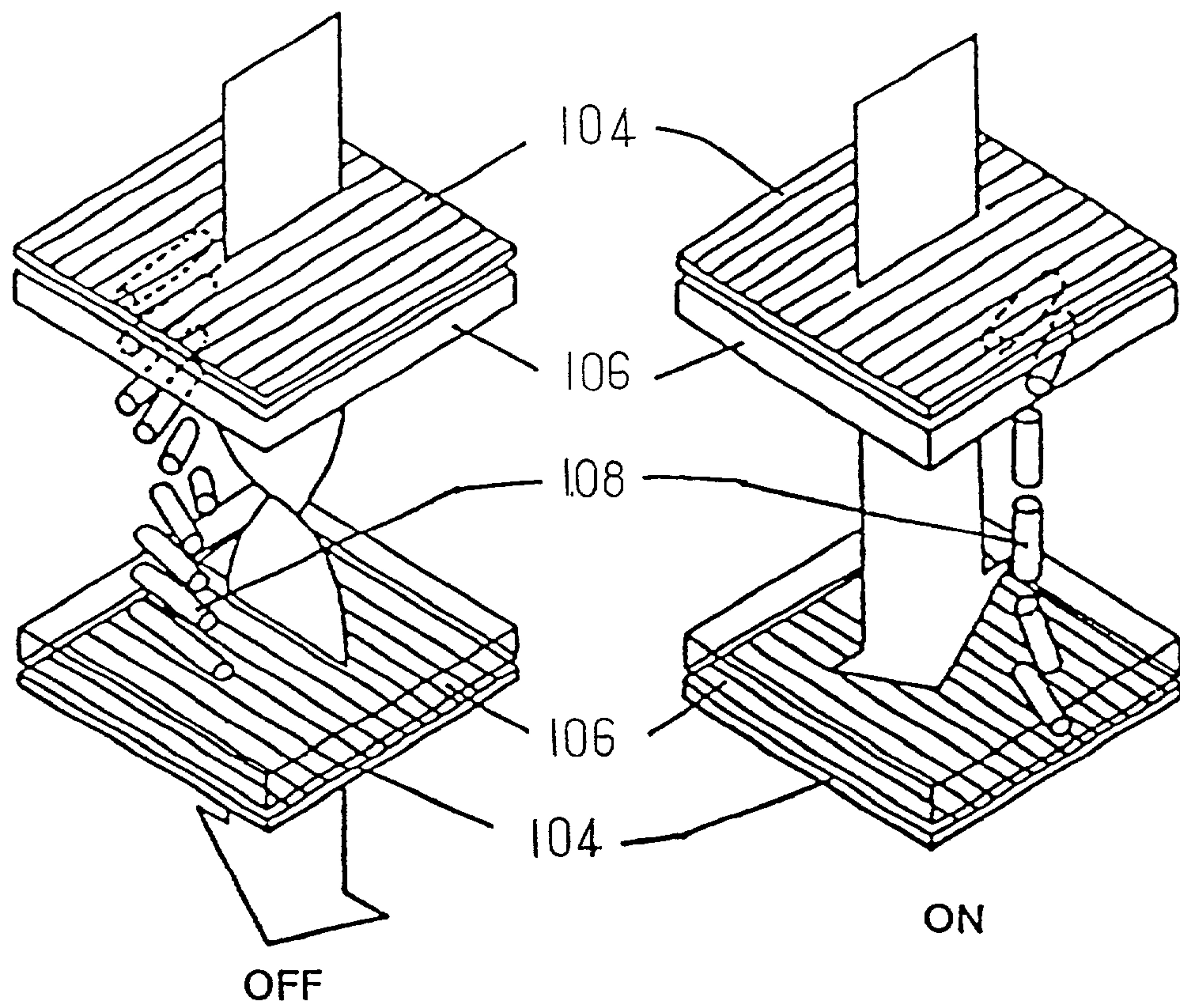
FIG. 3 (PRIOR ART)
