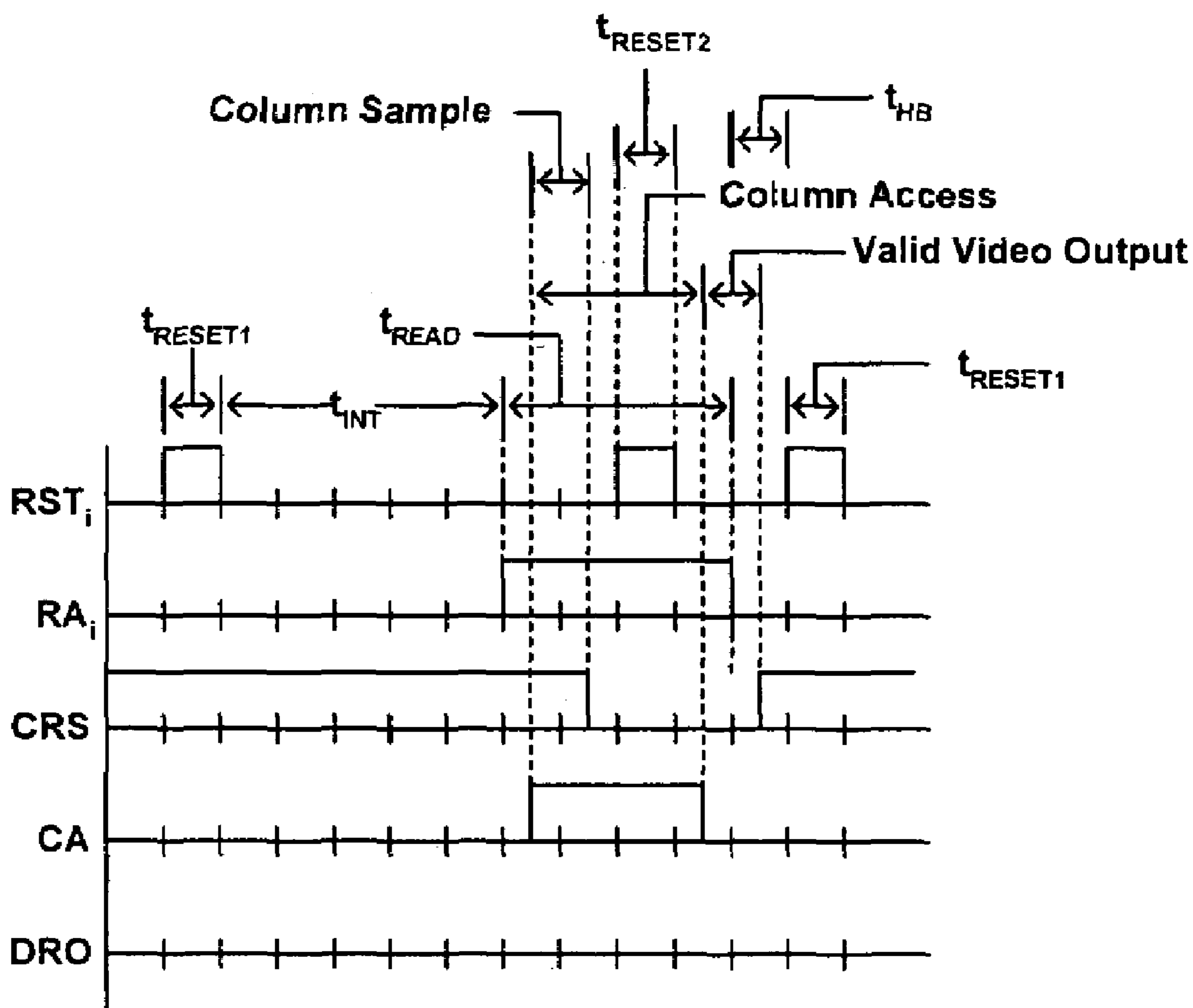
Figure 4 (PRIOR ART)
