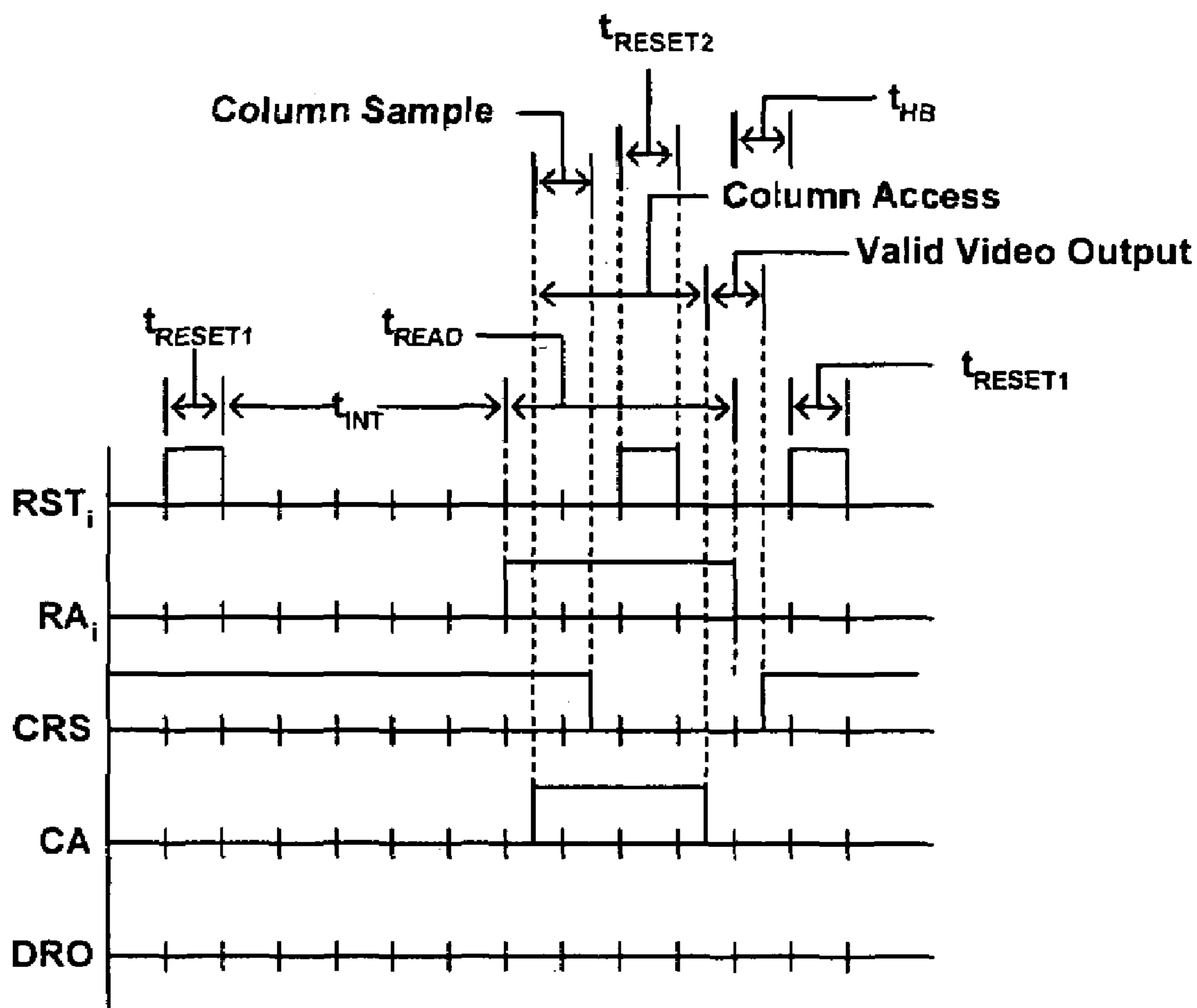
Figure 4 (PRIOR ART)
