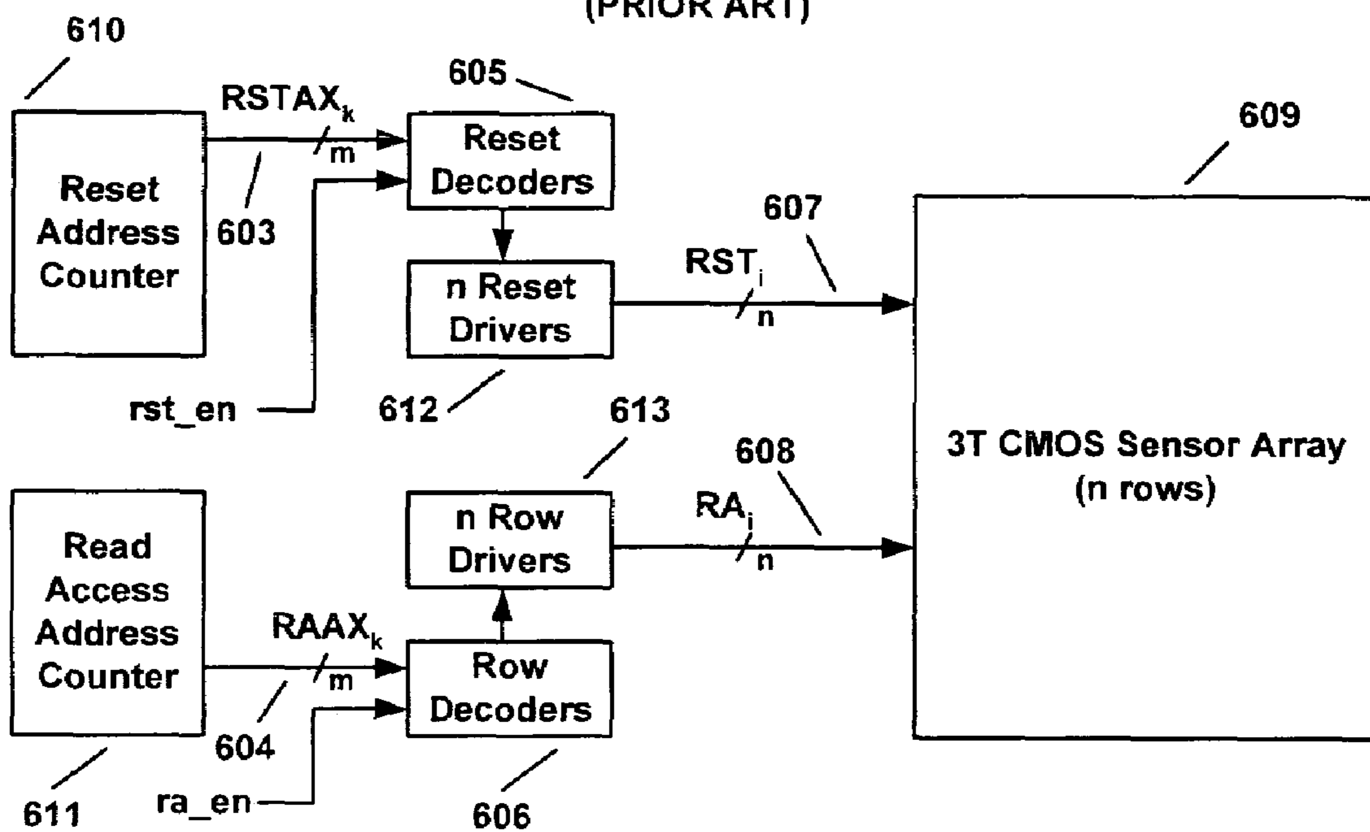
Figure 6 (PRIOR ART)
