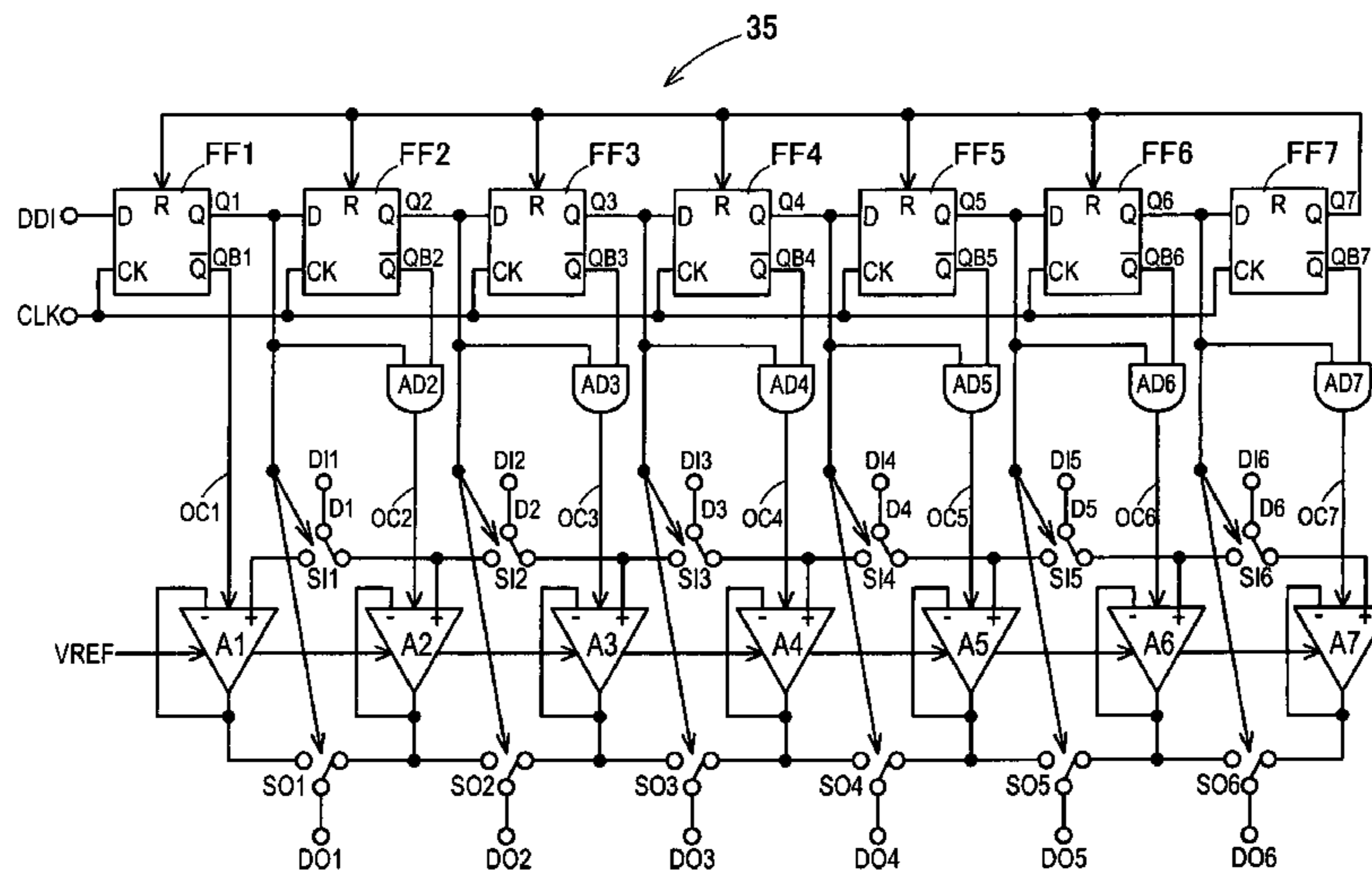
SCHMATIC DIAGRAM OF CIRCUIT BLOCK DIRECTED TO SECOND EMBODIMENT
