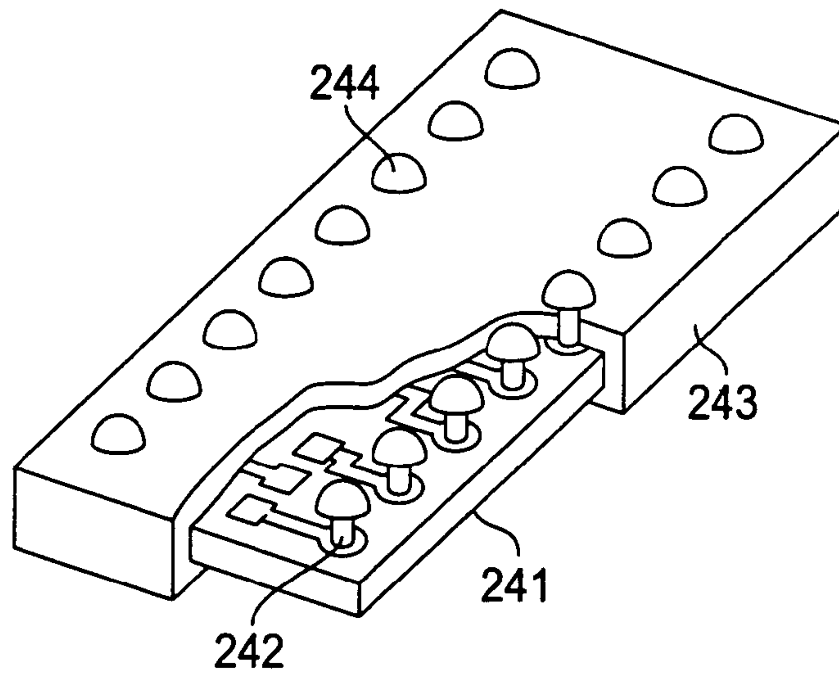
FIG. 24 (PRIOR ART)
