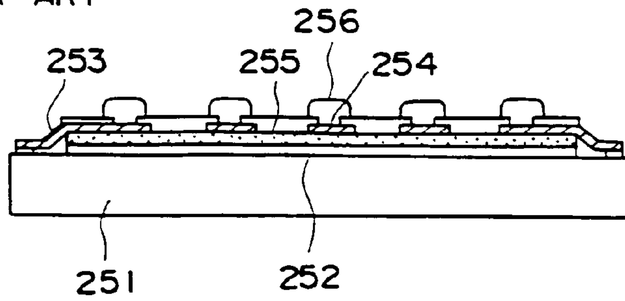
FIG. 25 PRIOR ART
