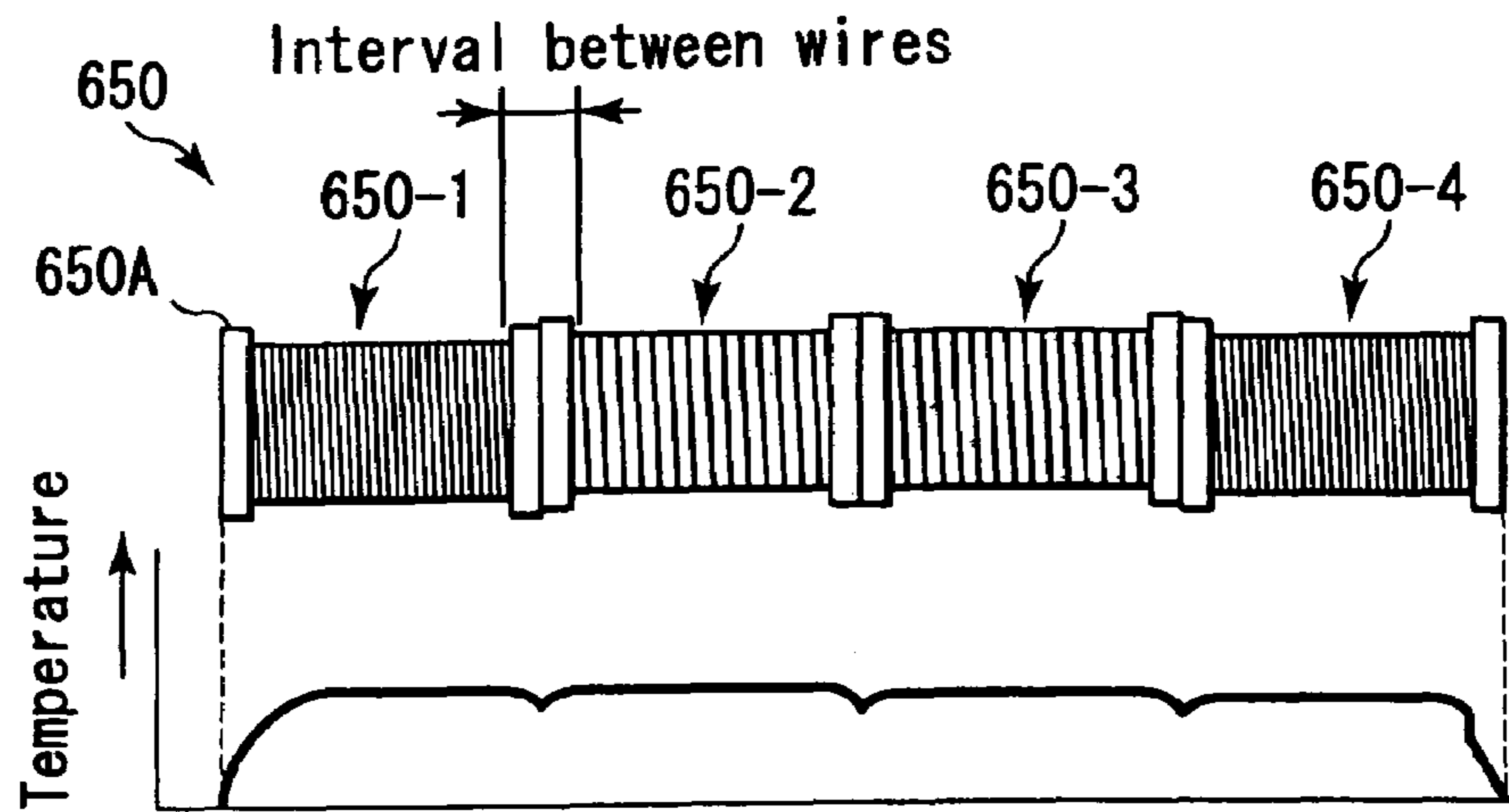
Heat generation distribution
