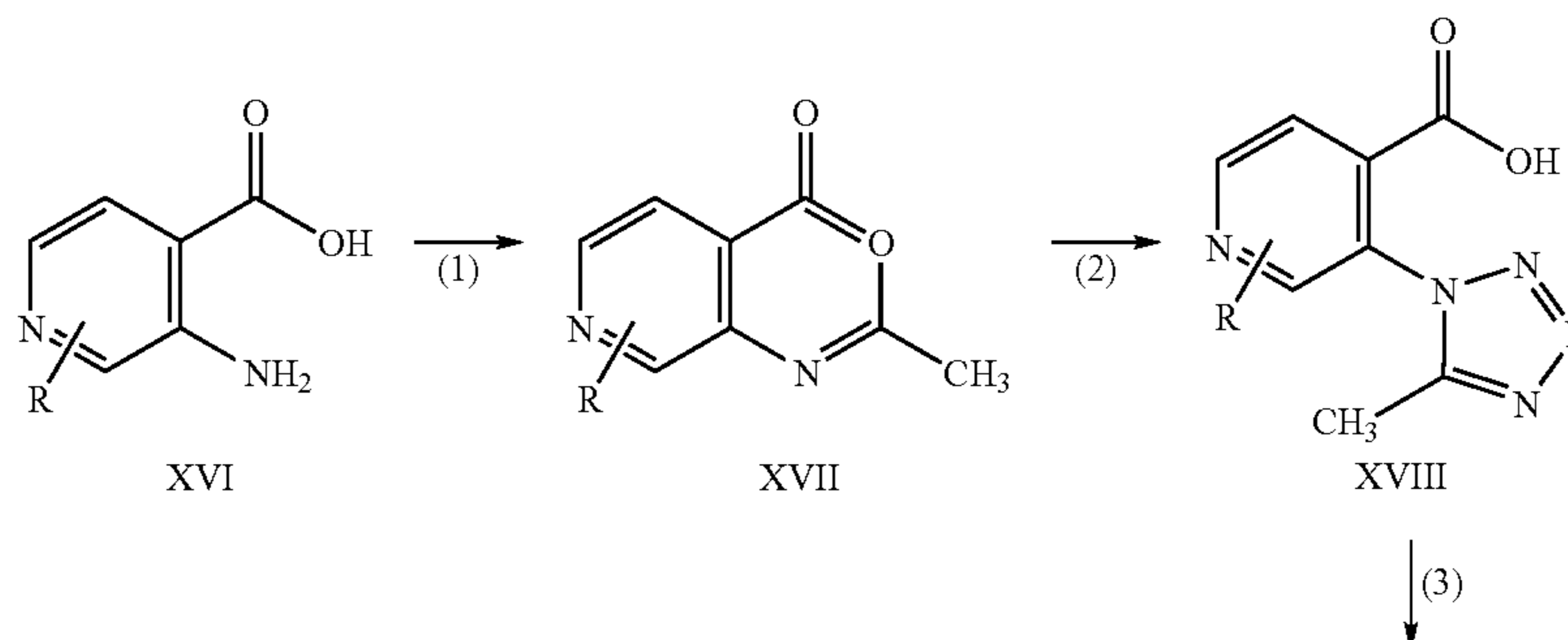
Reaction Scheme II
