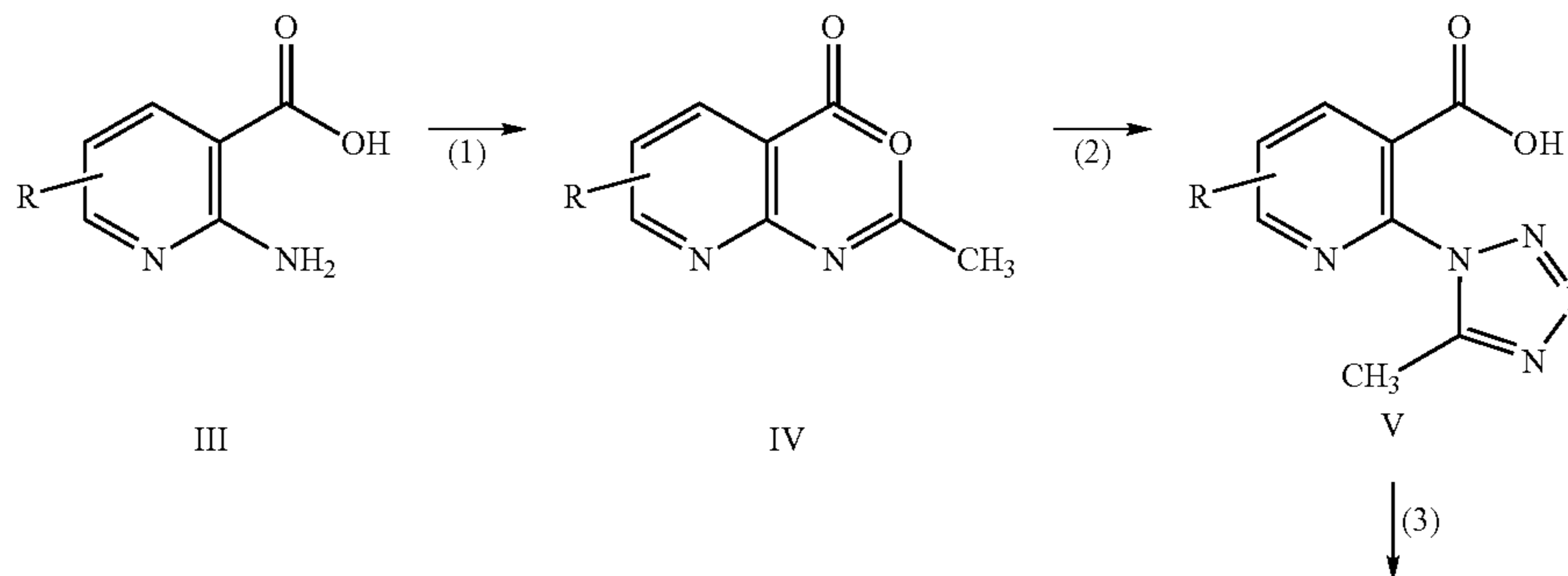
Reaction Scheme I
