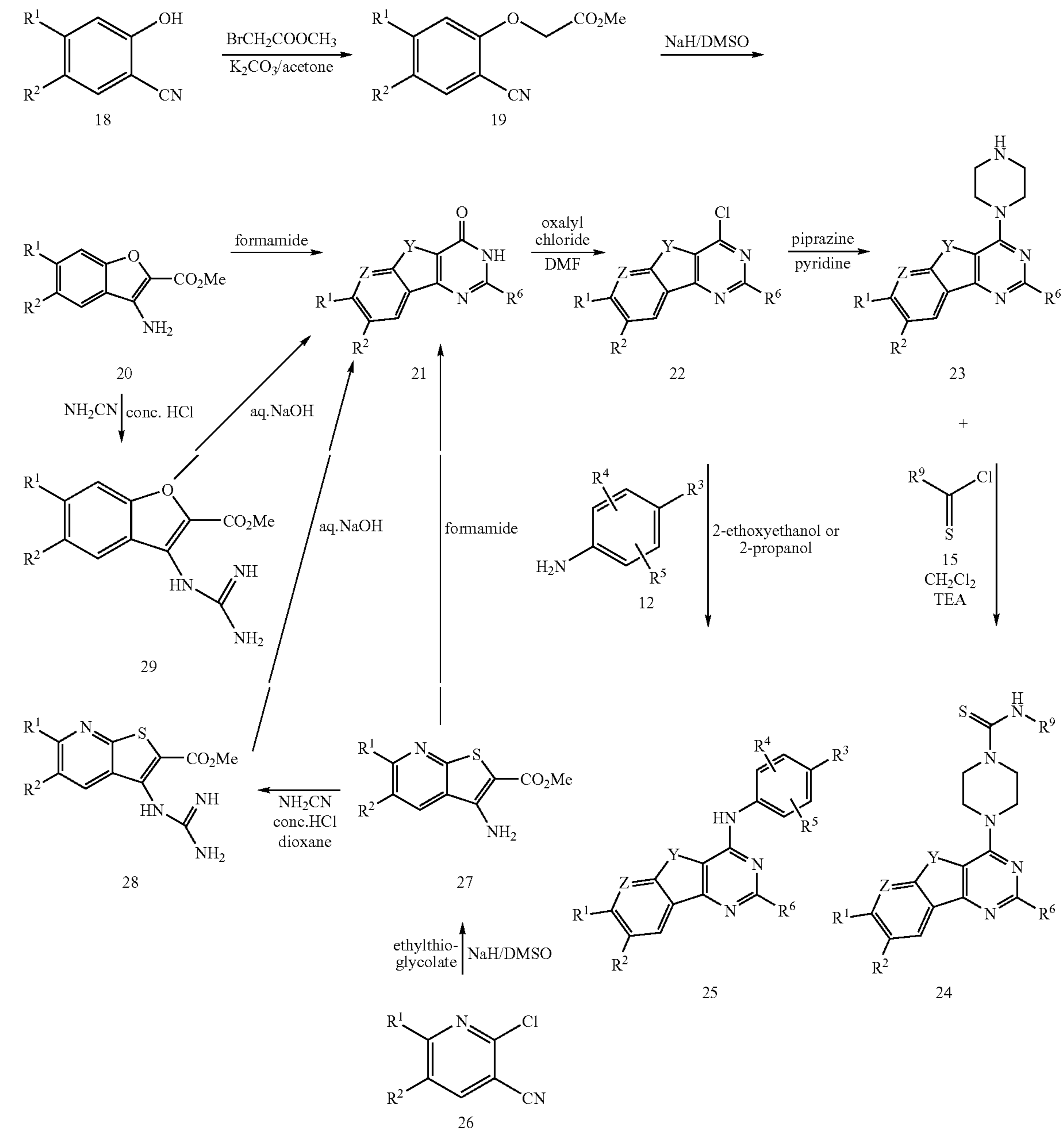
Scheme 14
