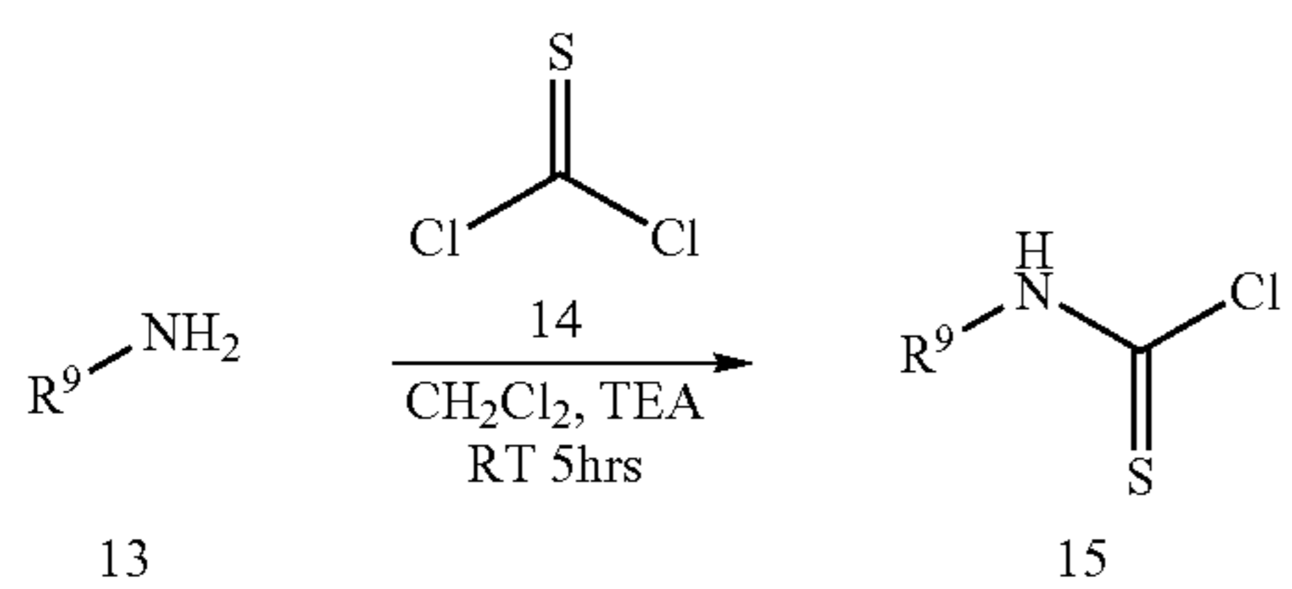
Scheme 12
