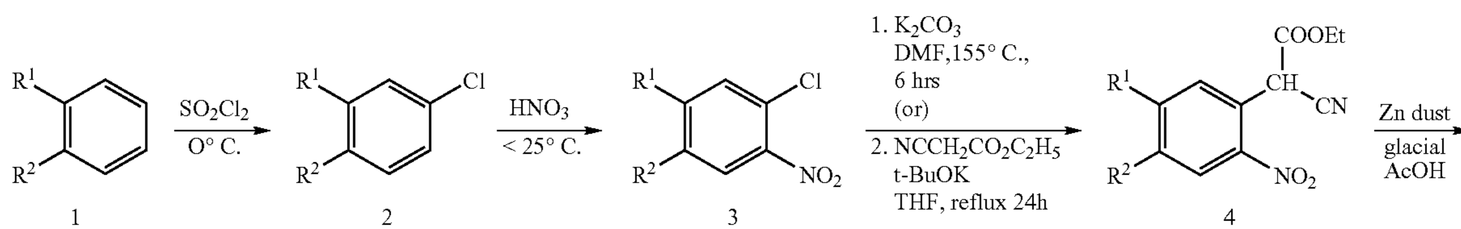
Scheme 11
