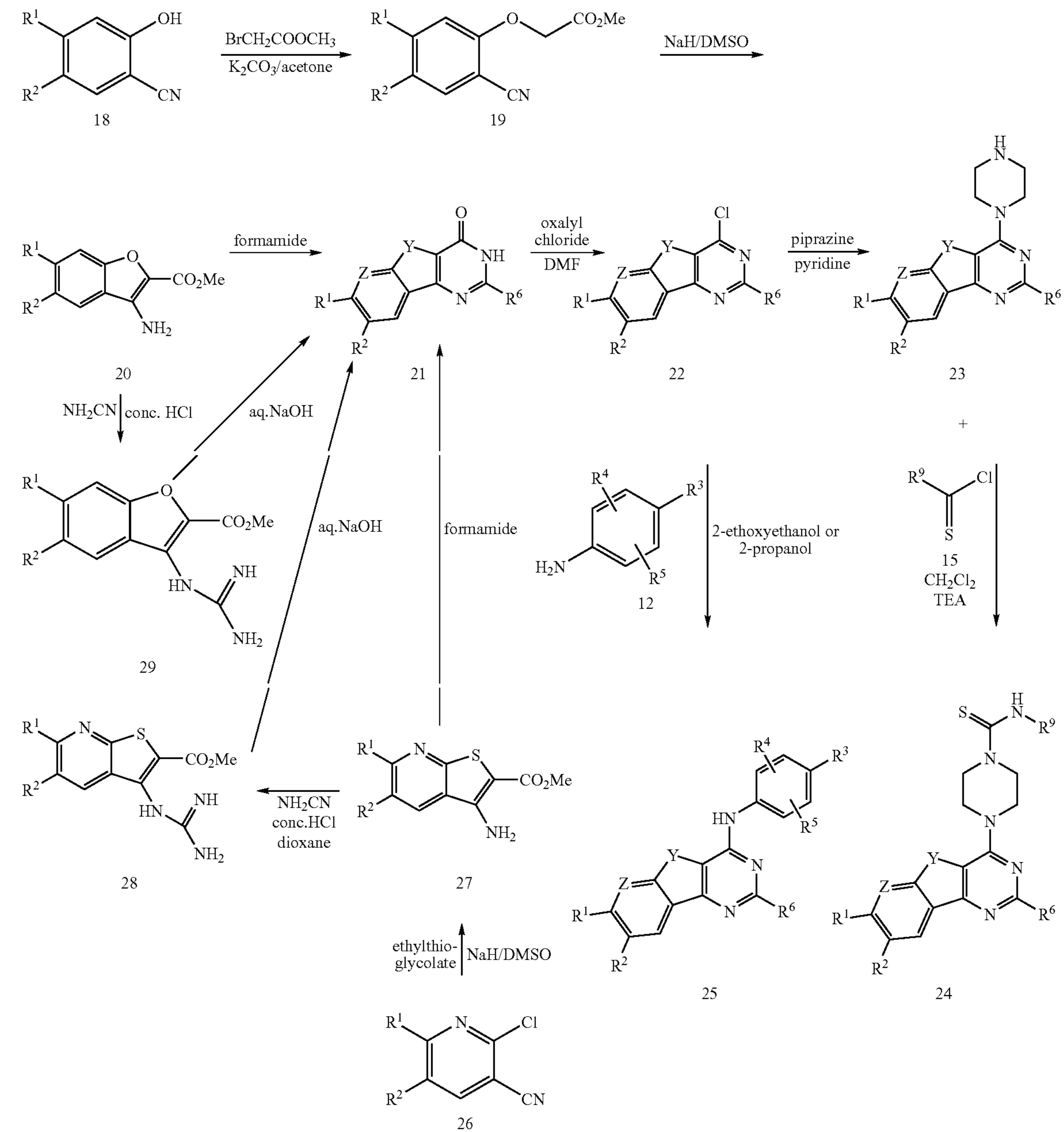
Scheme 14
