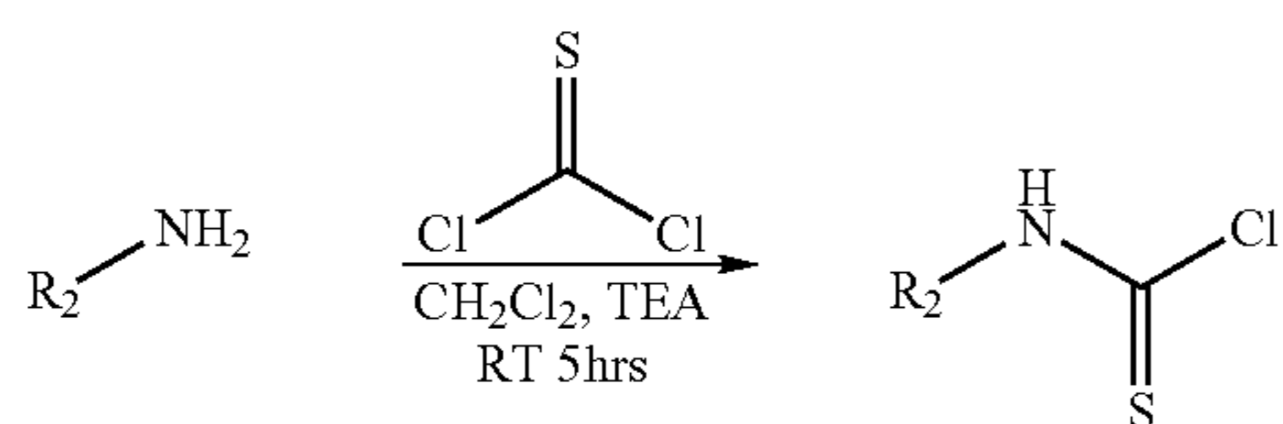
Scheme 2
