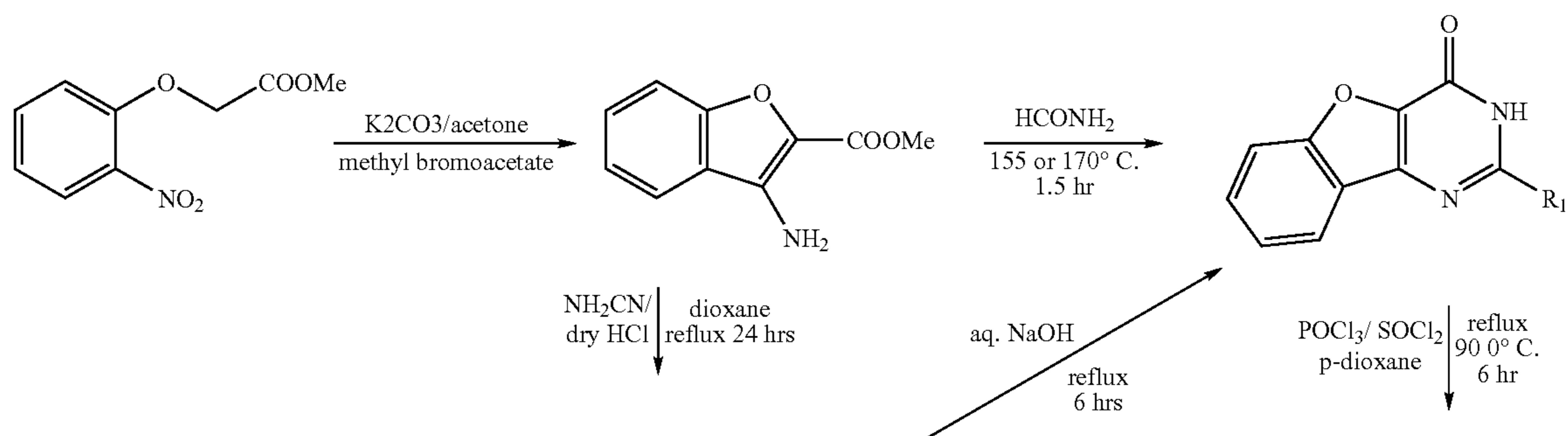
Scheme 1
