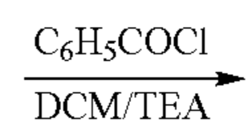
Scheme 13
