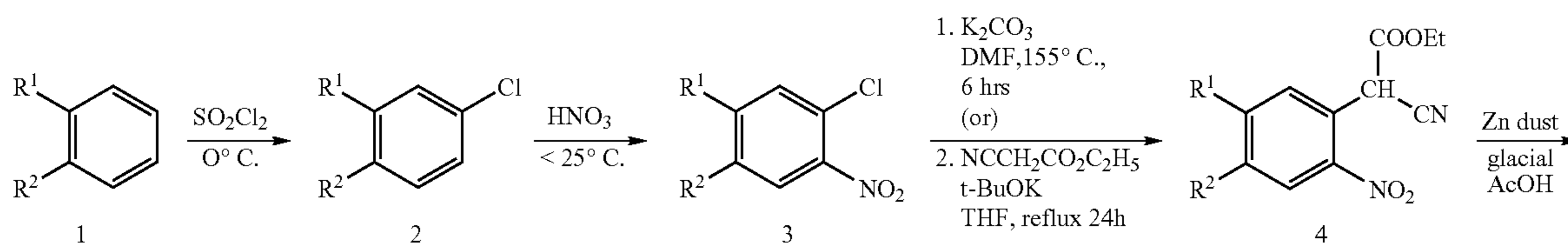
Scheme 11
