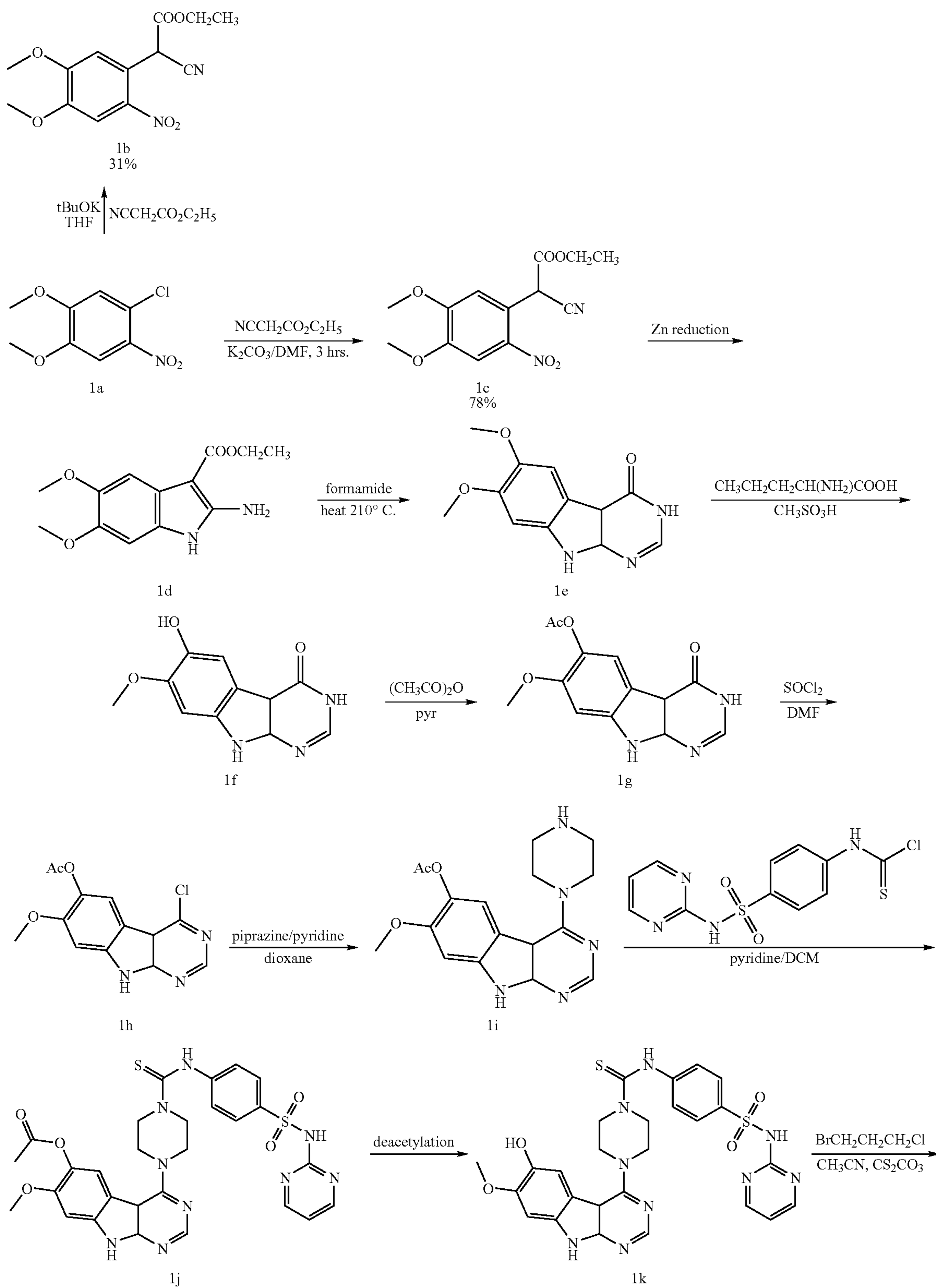
Scheme 7
