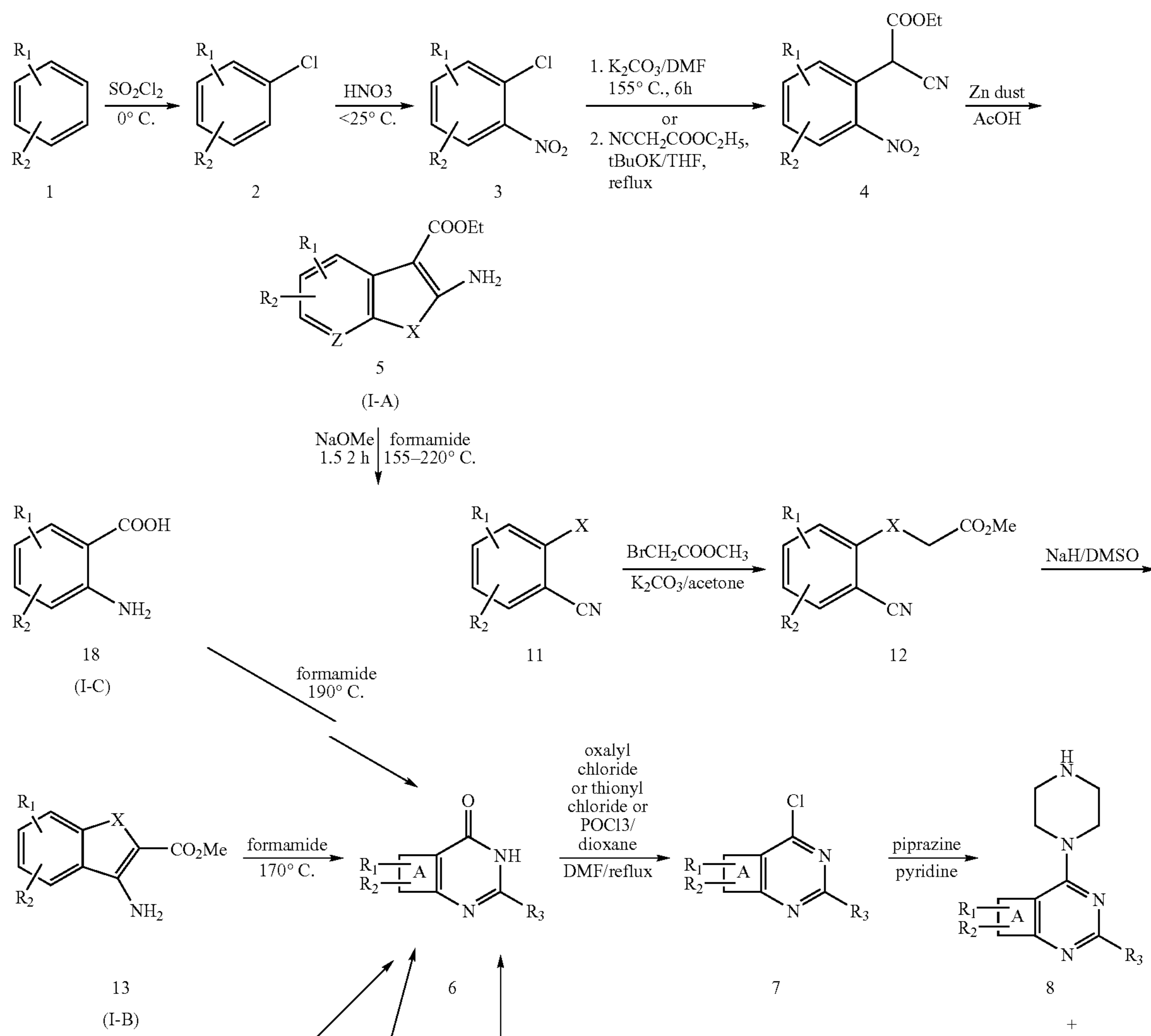
Scheme 1
