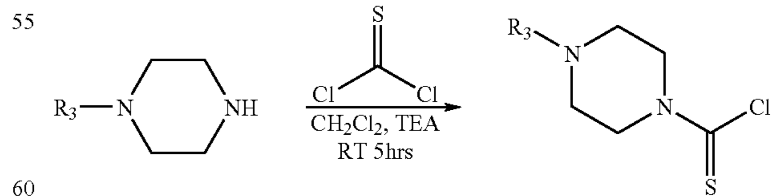
Scheme 3
