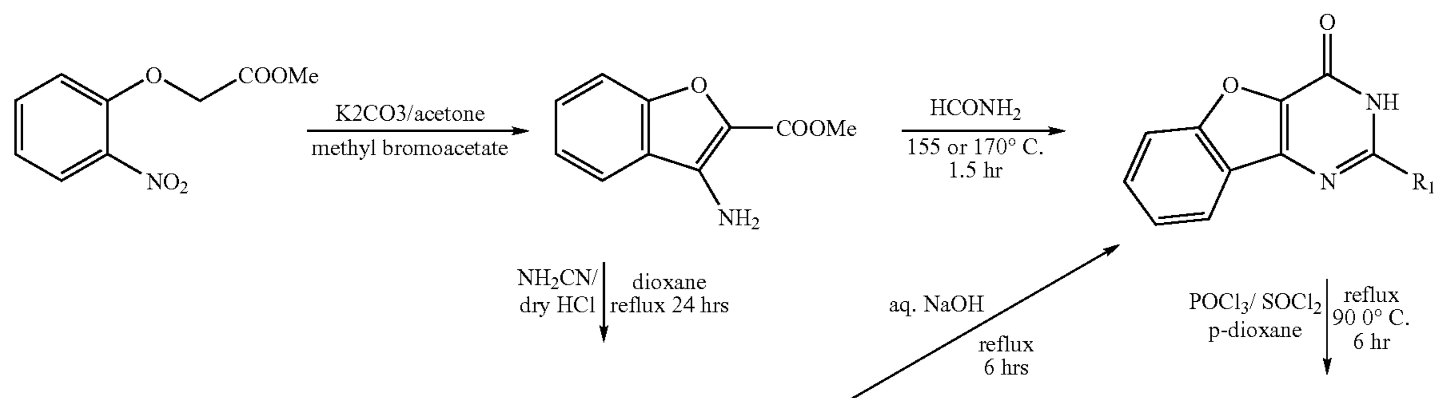
Scheme 1
