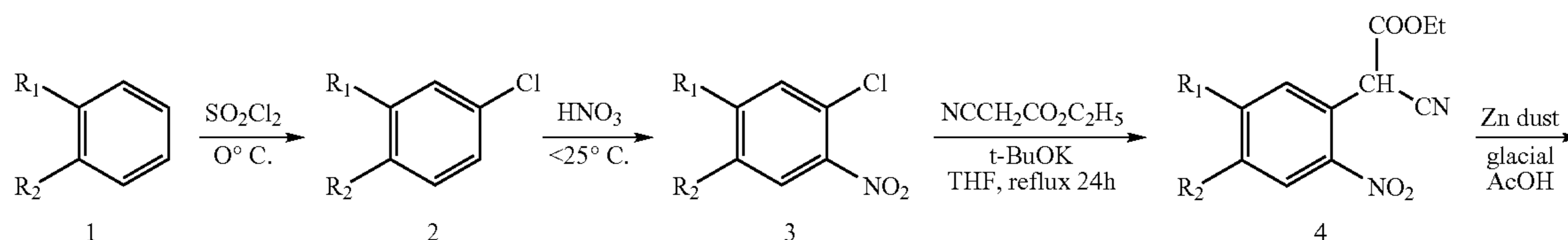
Scheme 3
