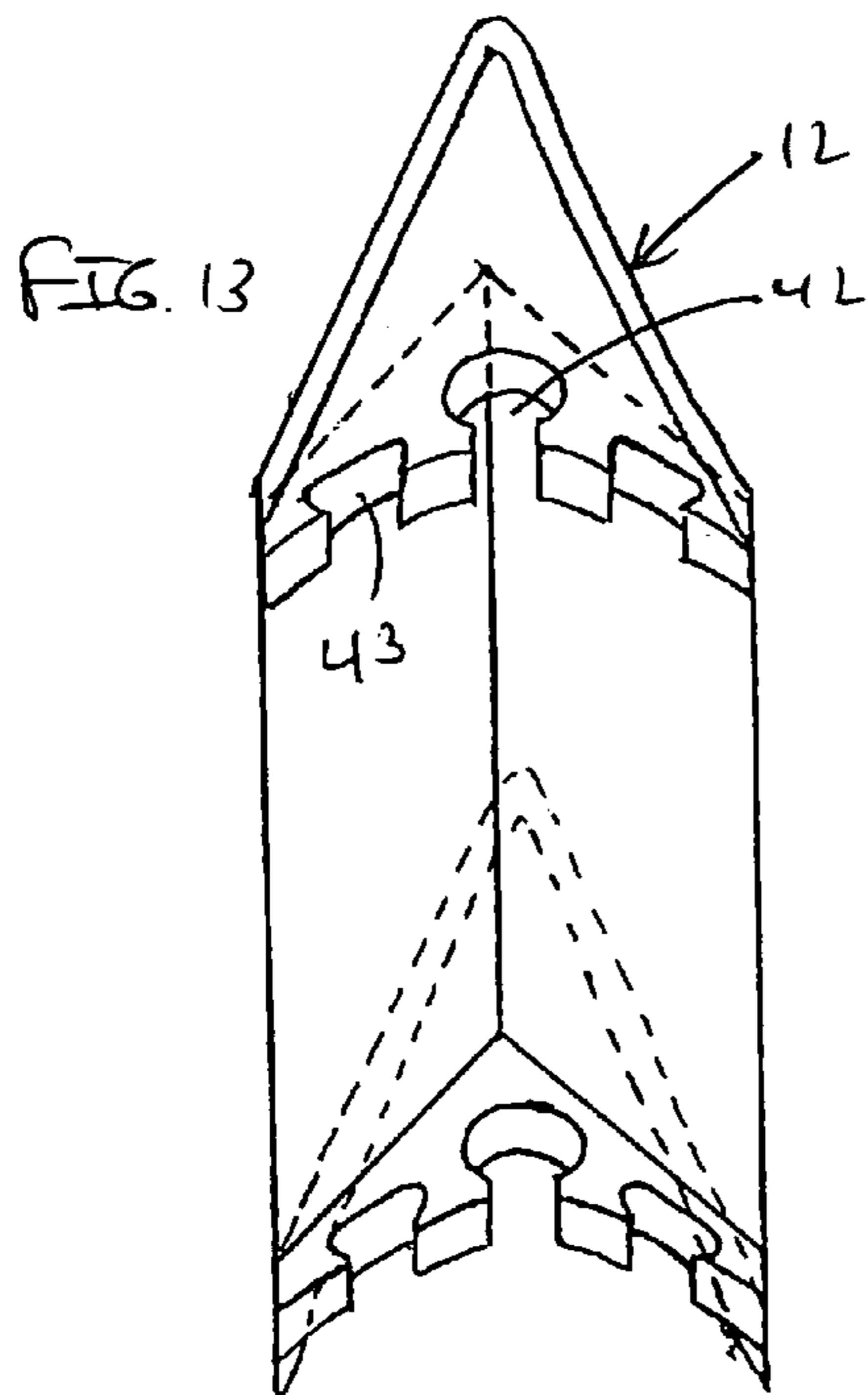
ISOMETRIC FRONT VIEW
