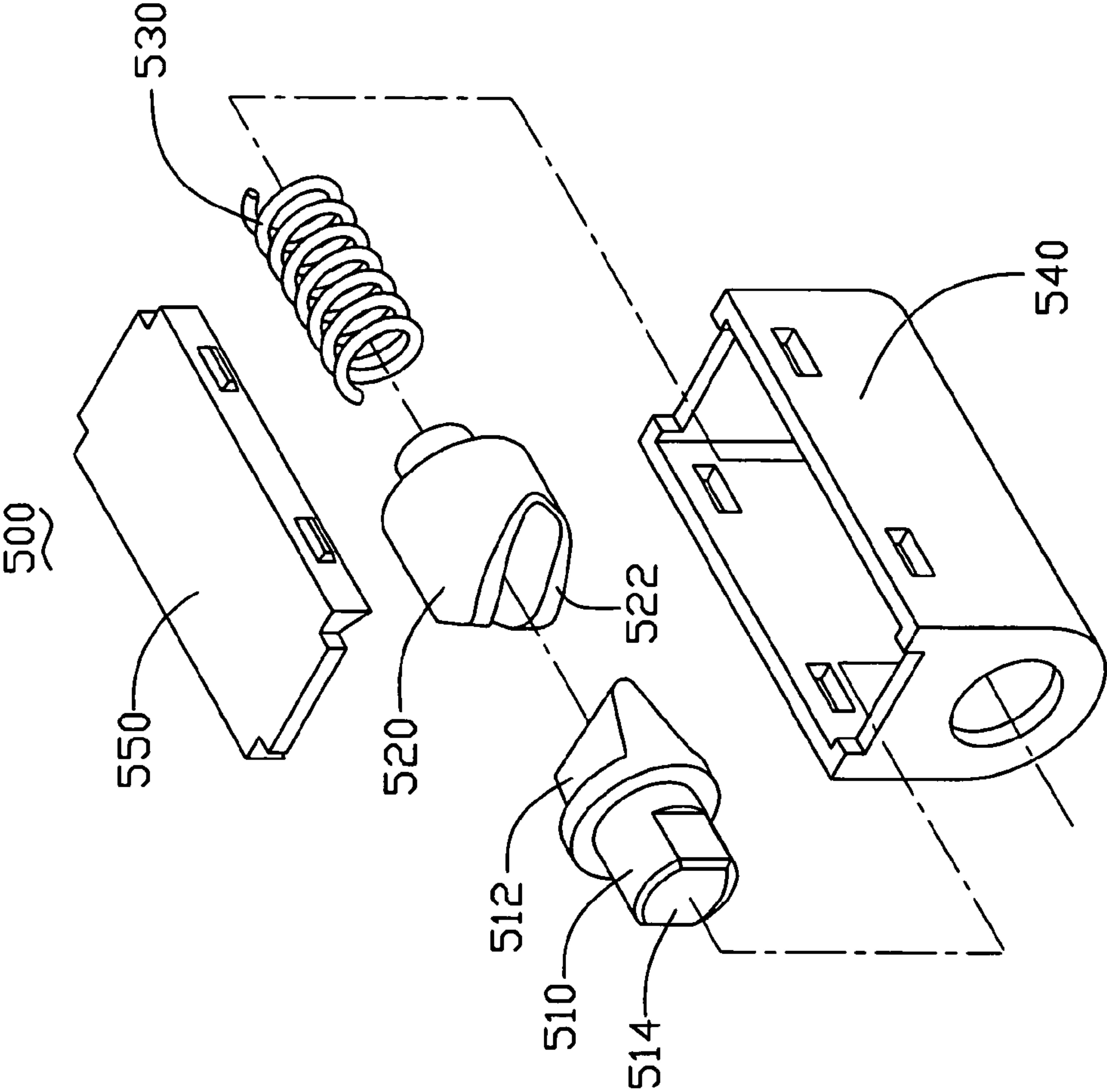
FIG. 5 (RELATED ART)
