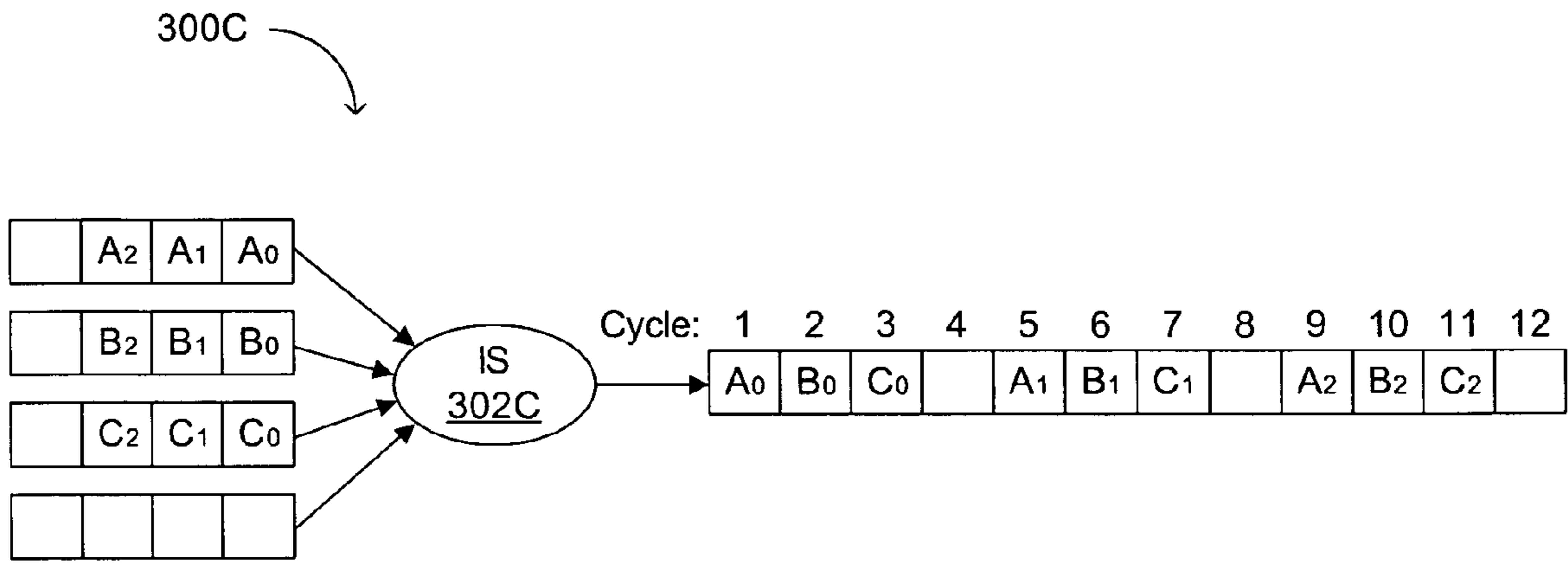
FIG. 3C (conventional)
