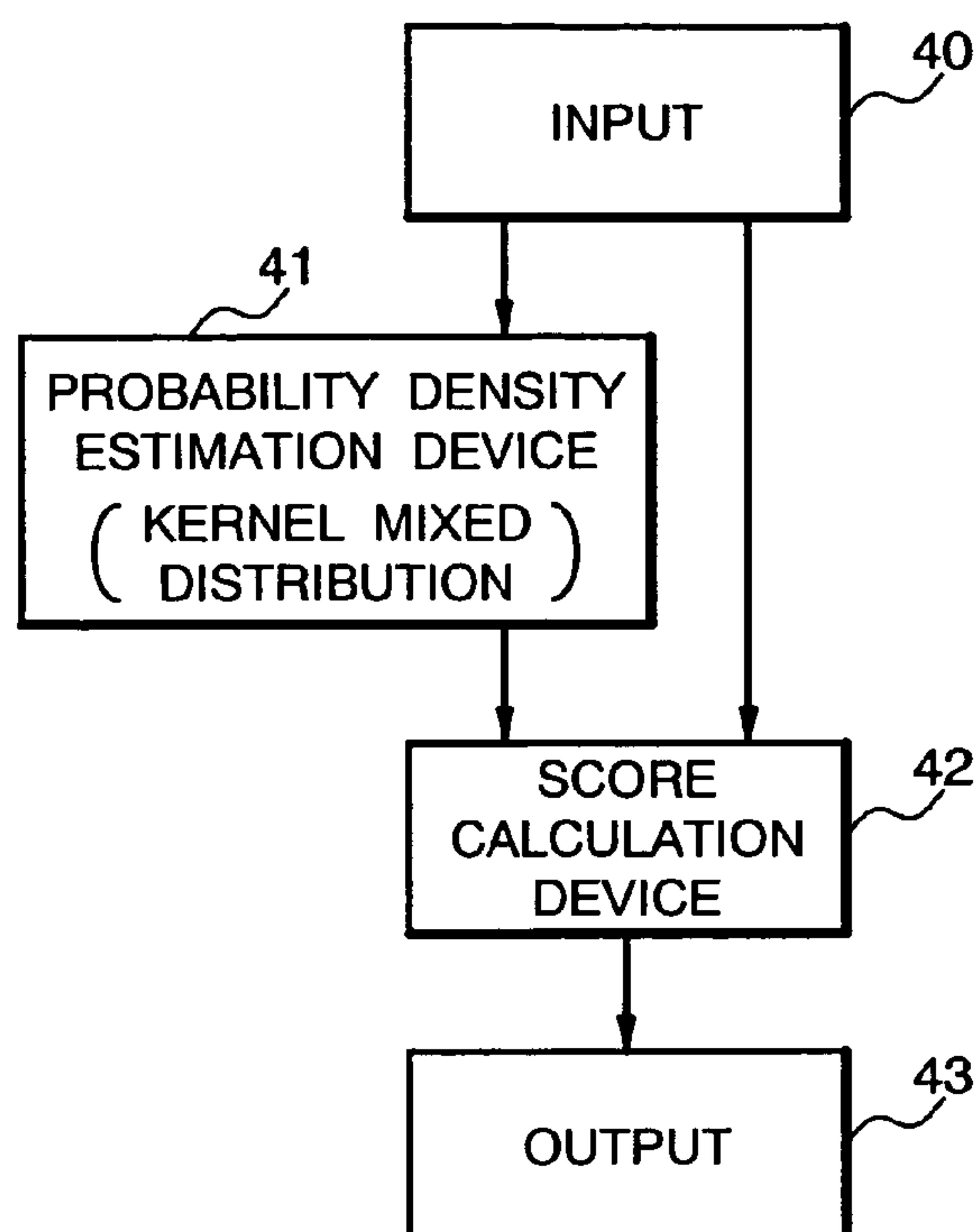
DEGREE OF OUTLIER CALCULATION DEVICE
