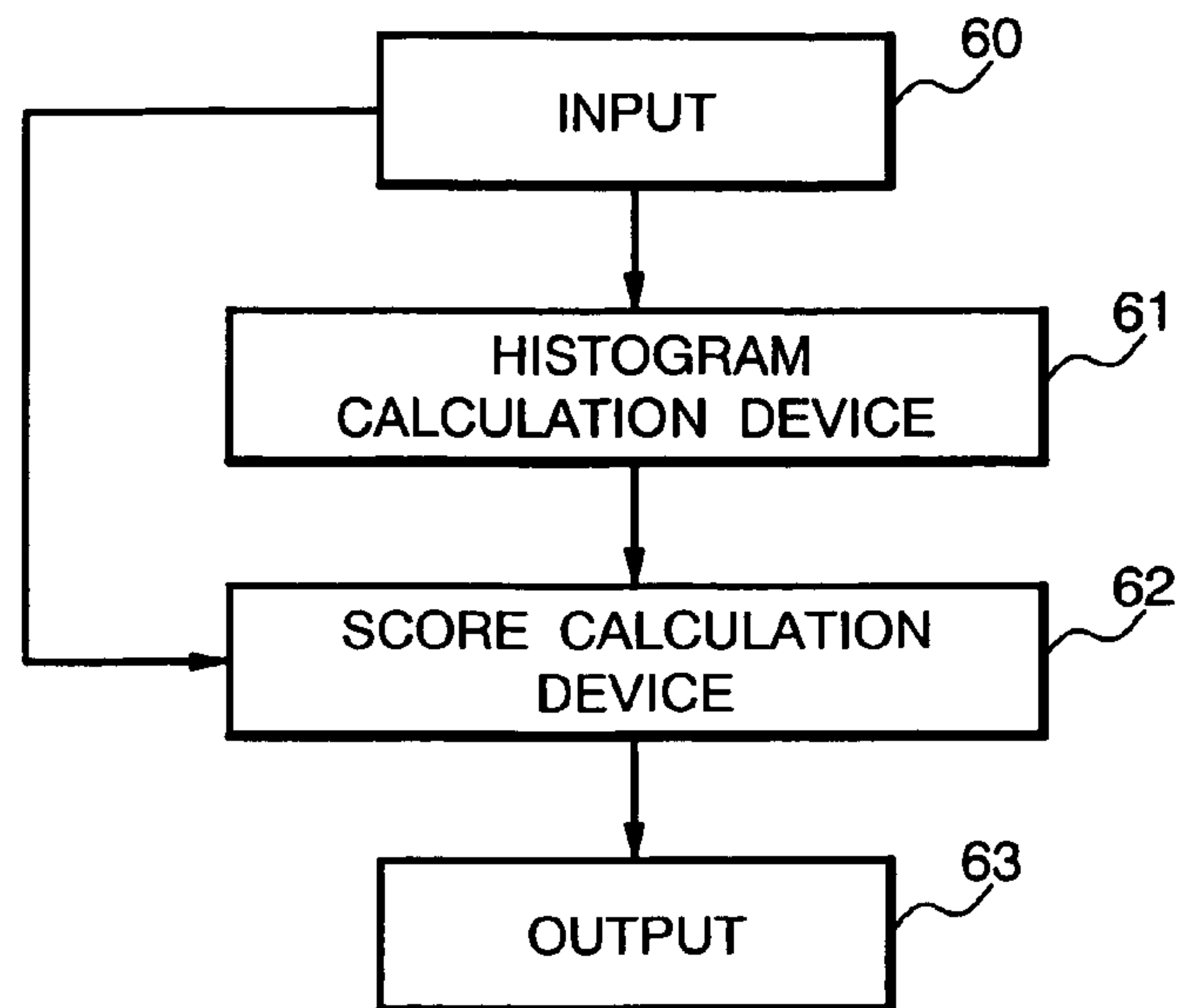
DEGREE OF OUTLIER CALCULATION DEVICE
