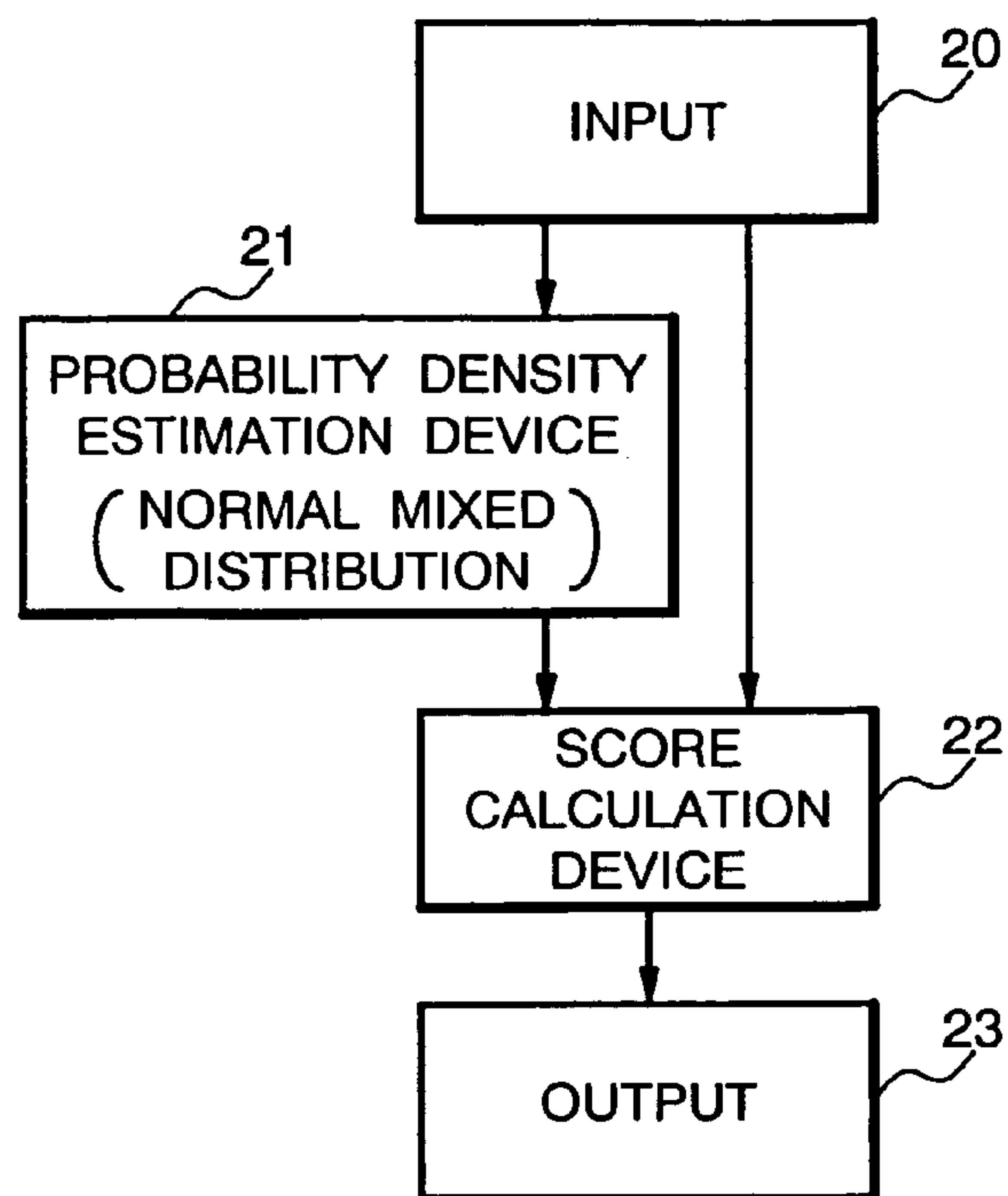
DEGREE OF OUTLIER CALCULATION DEVICE
