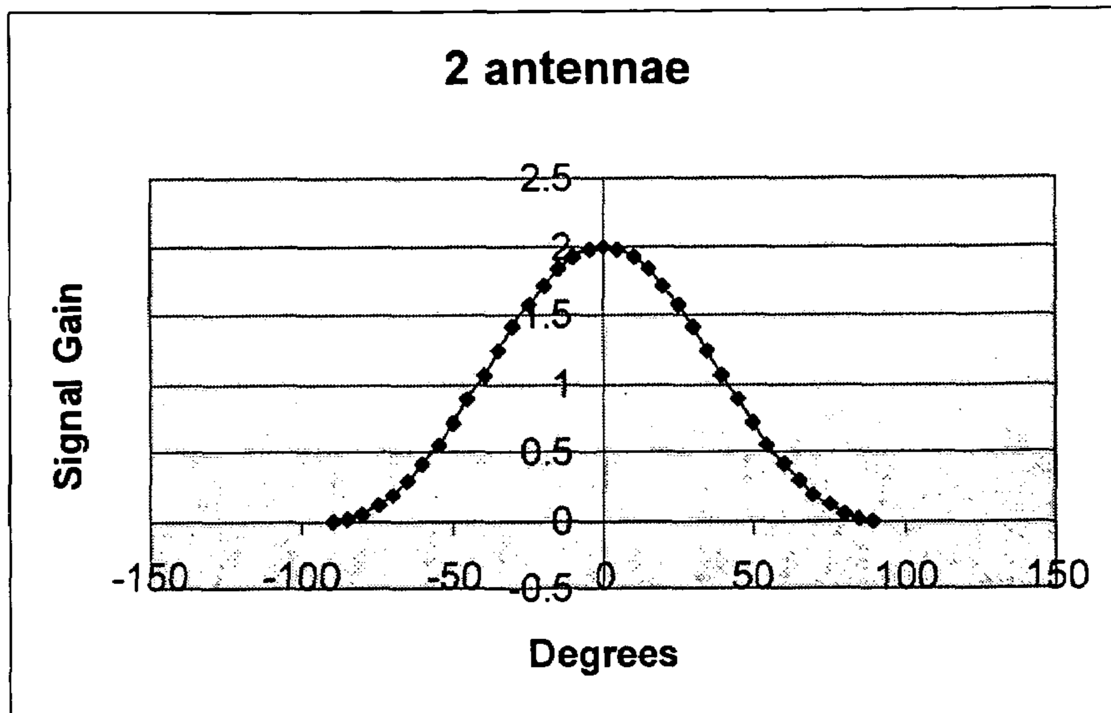
Fig 7a Beam Pattern for Two Elements
