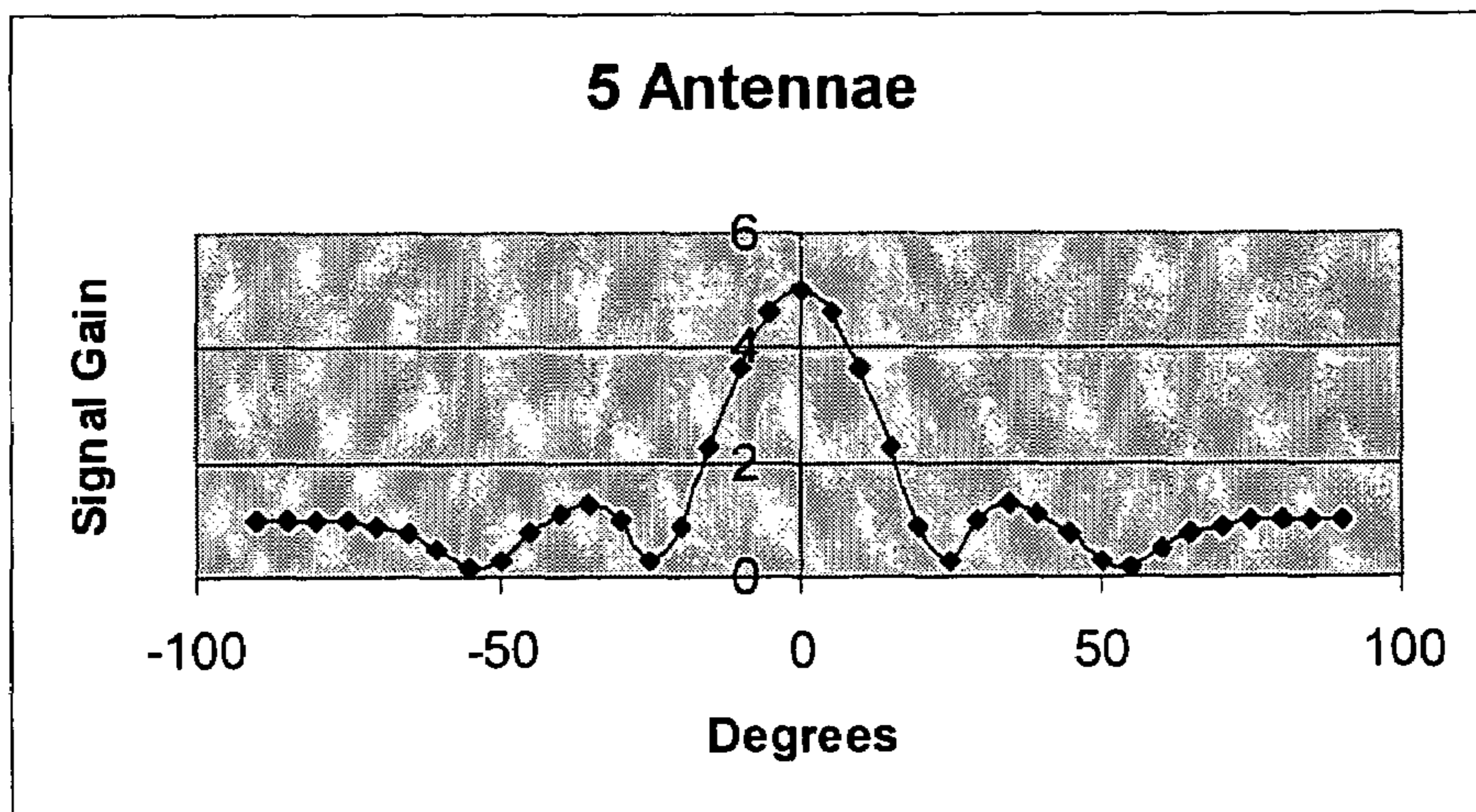
Fig 7b Beam Pattern for Five Elements
