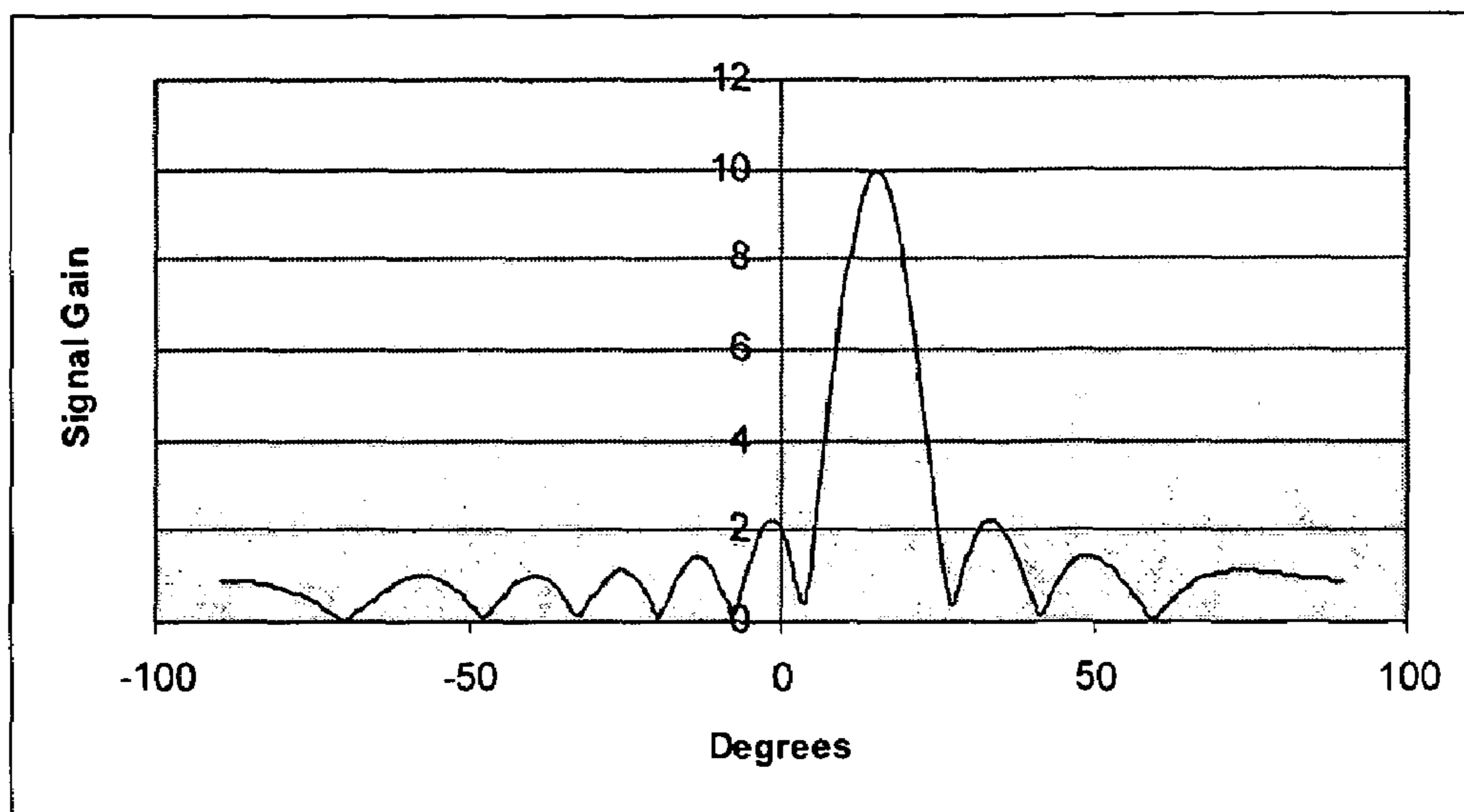
Fig 11a Scanned Beam Pattern for ten antennae elements
