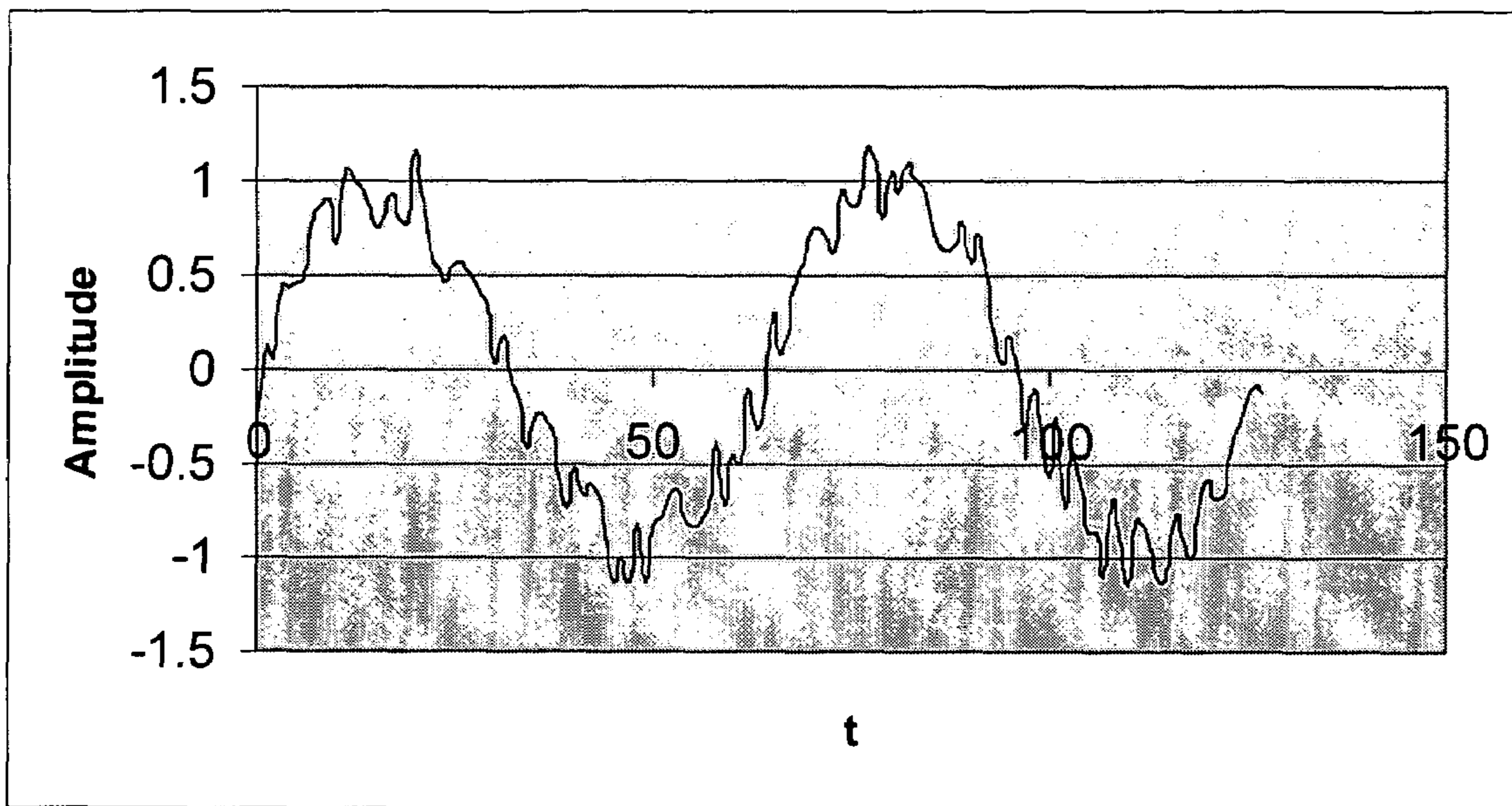
Fig 1 Effect of noise on a received waveform
