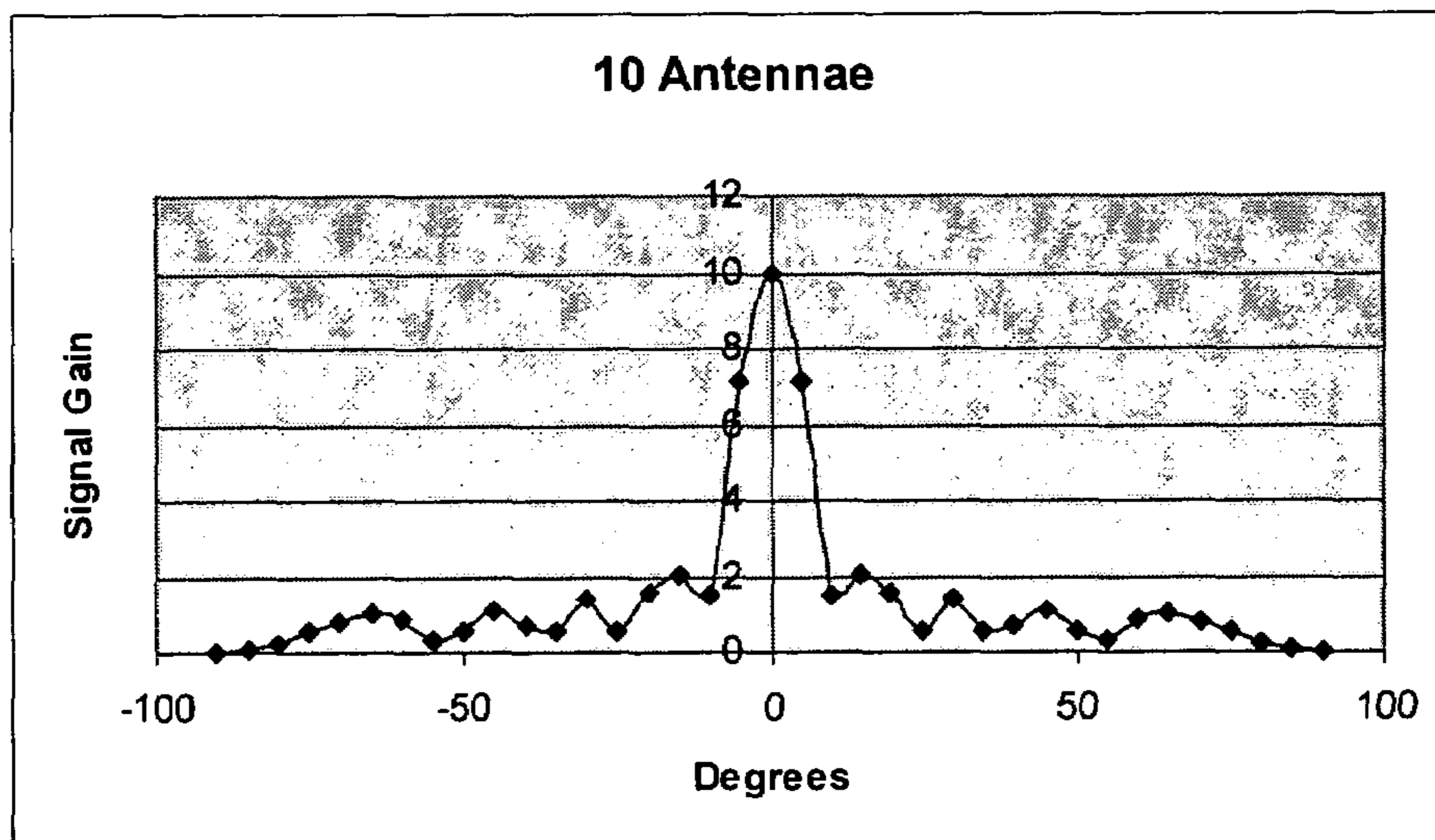
Fig 7c Beam Pattern for Five Elements
