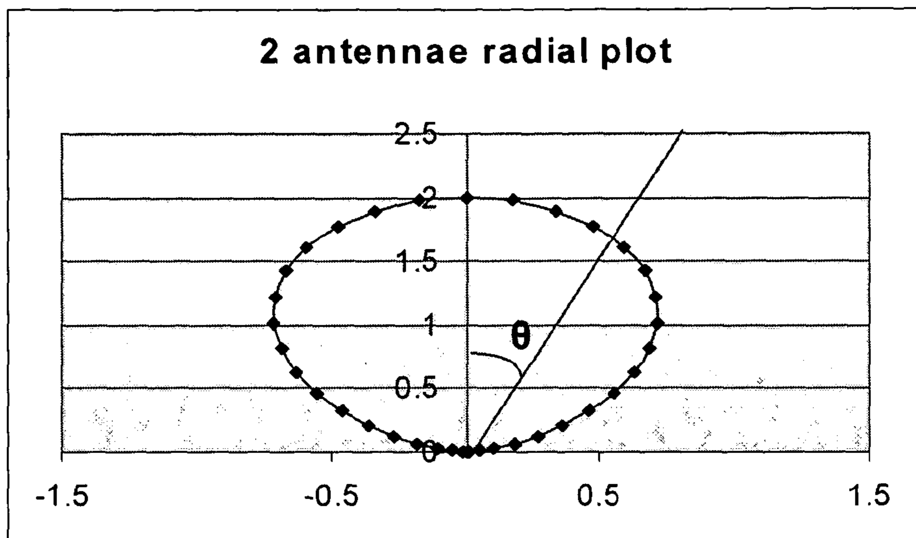
Fig 8a Radial Plot of beam pattern of antennae array with two elements
