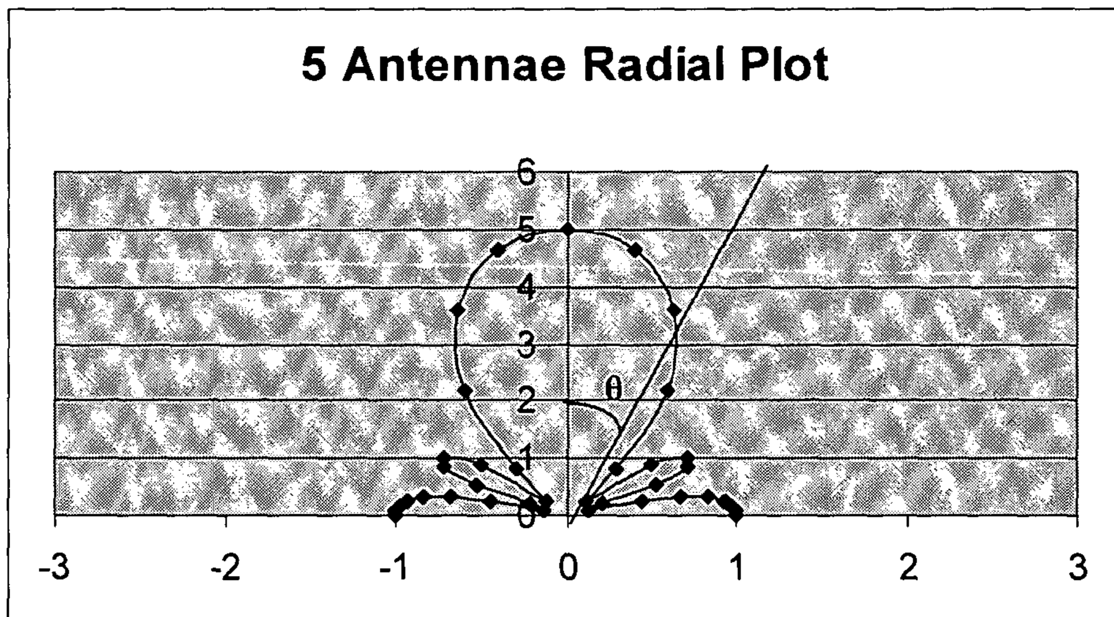
Fig 8b Radial Plot of beam pattern of antennae array with five elements
