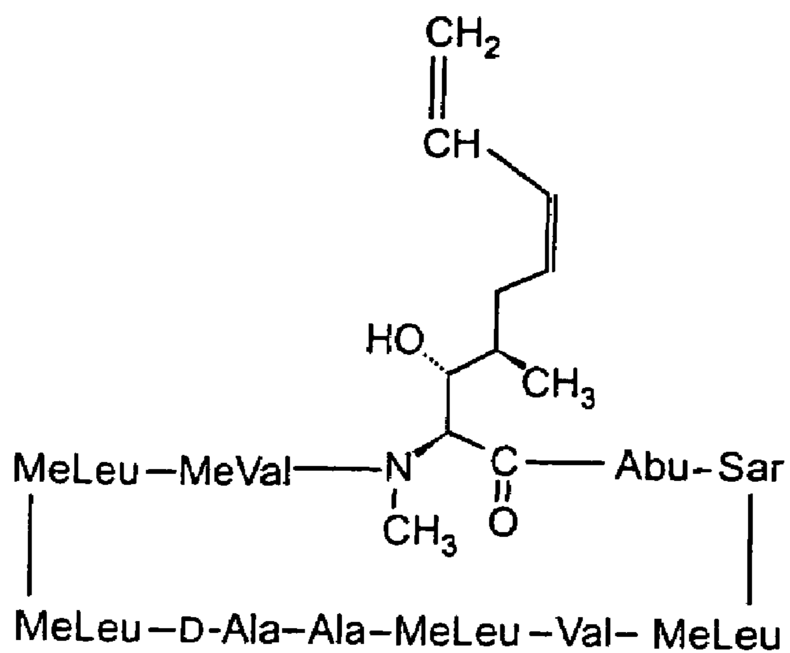
Z-isomer of ISA tx 247
