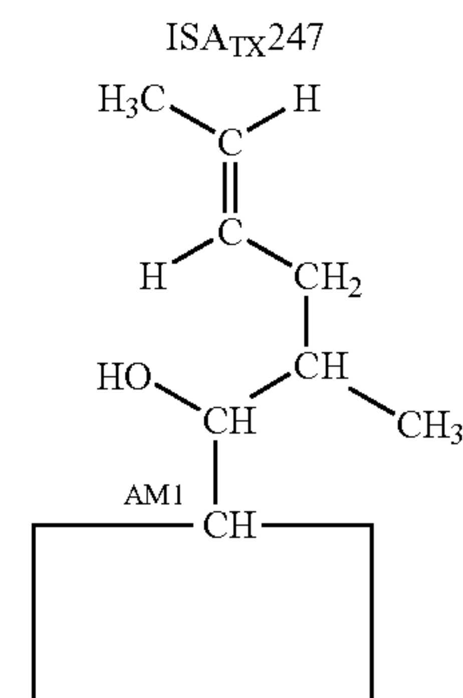
CYCLOSPORIN
