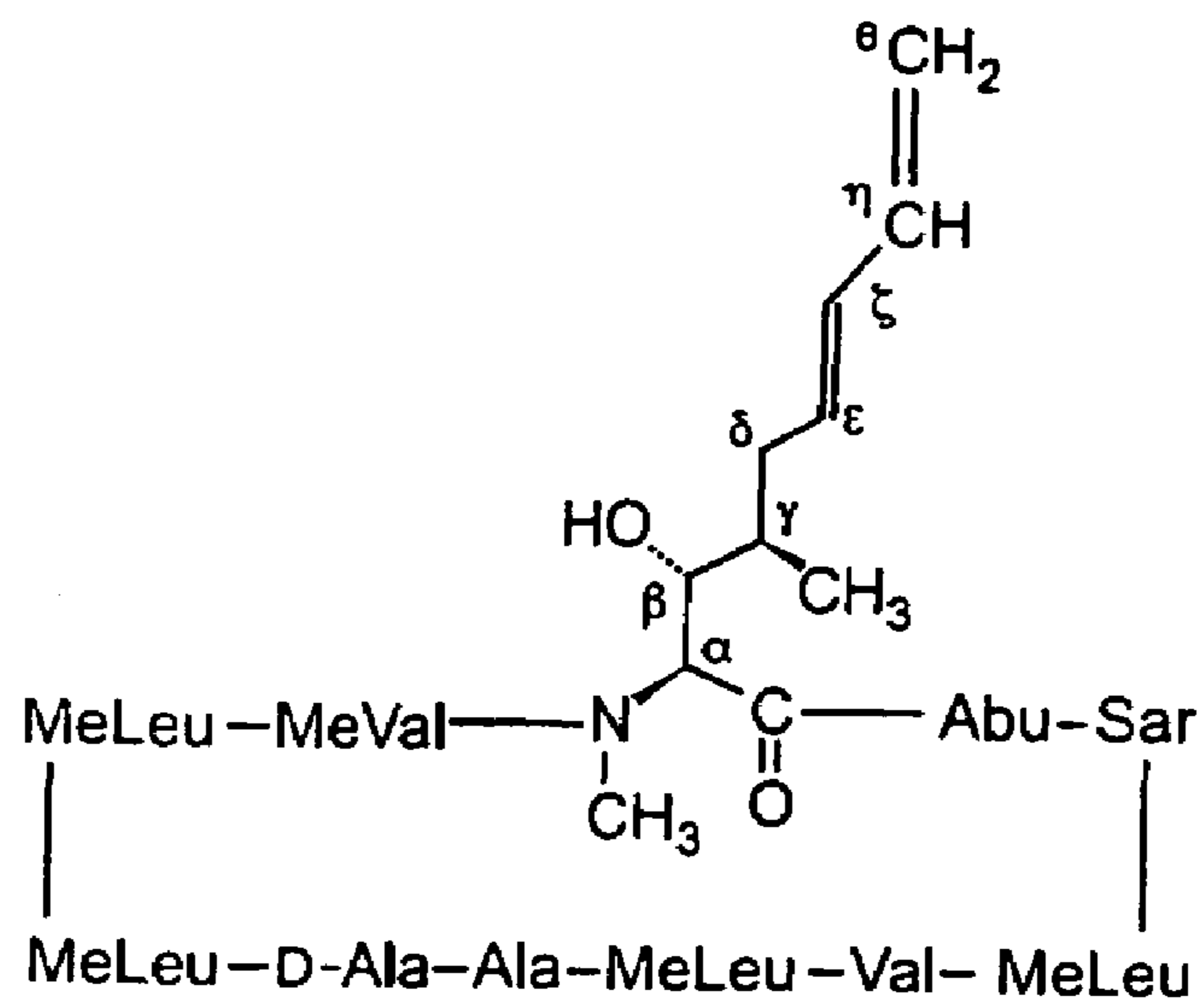
E-isomer of ISA tx 247
