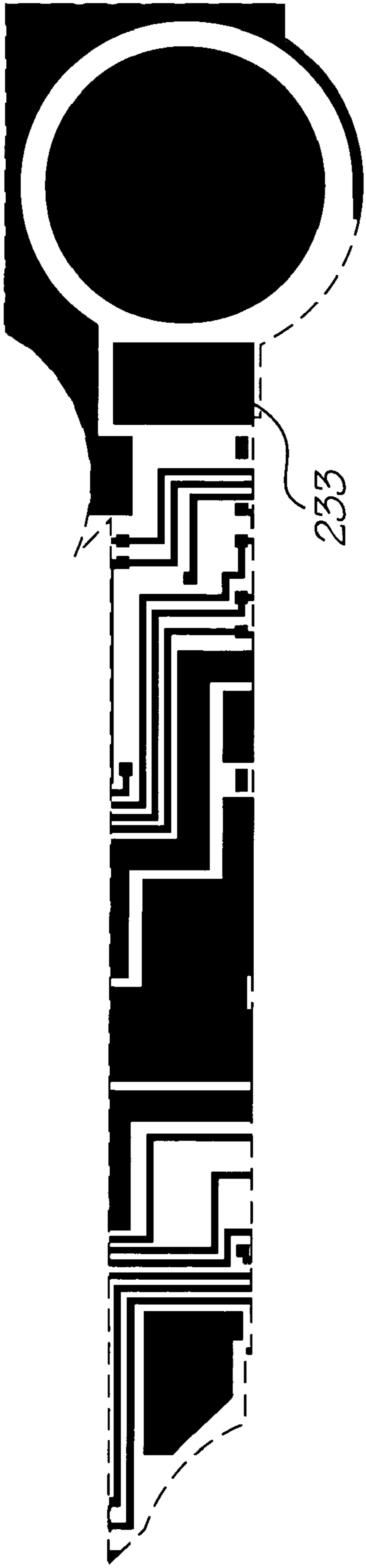
Metal 2 mask
