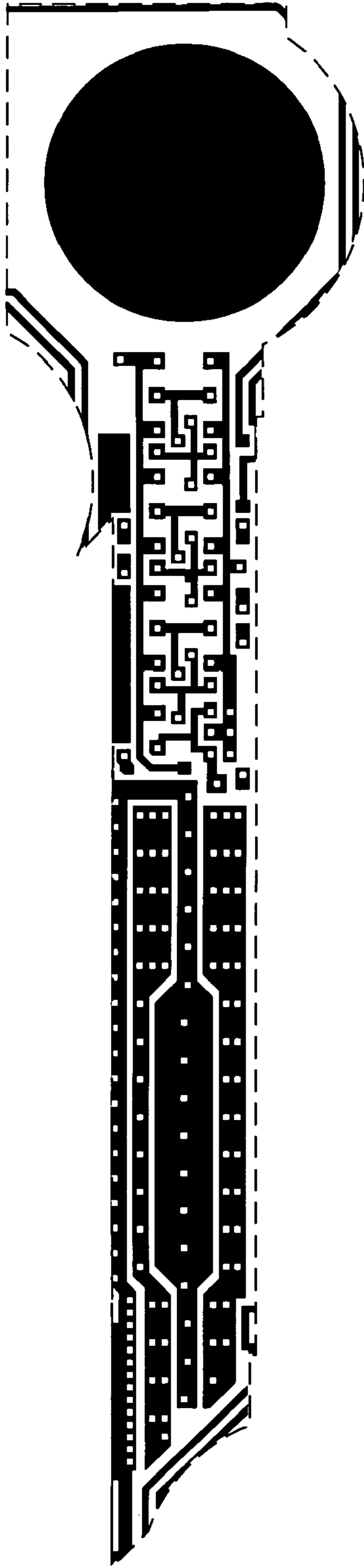
Metal 1 mask
