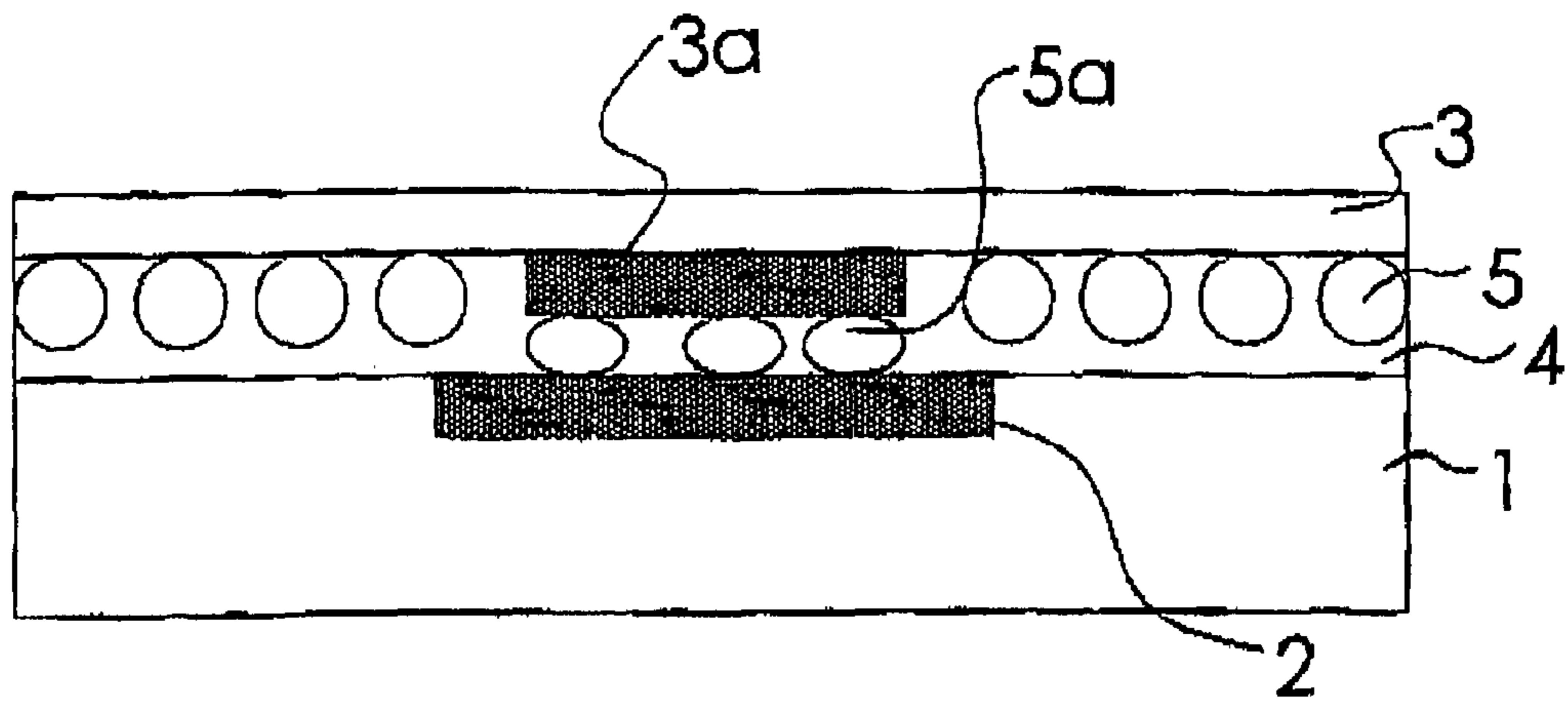
Fig. 1 (prior art)
