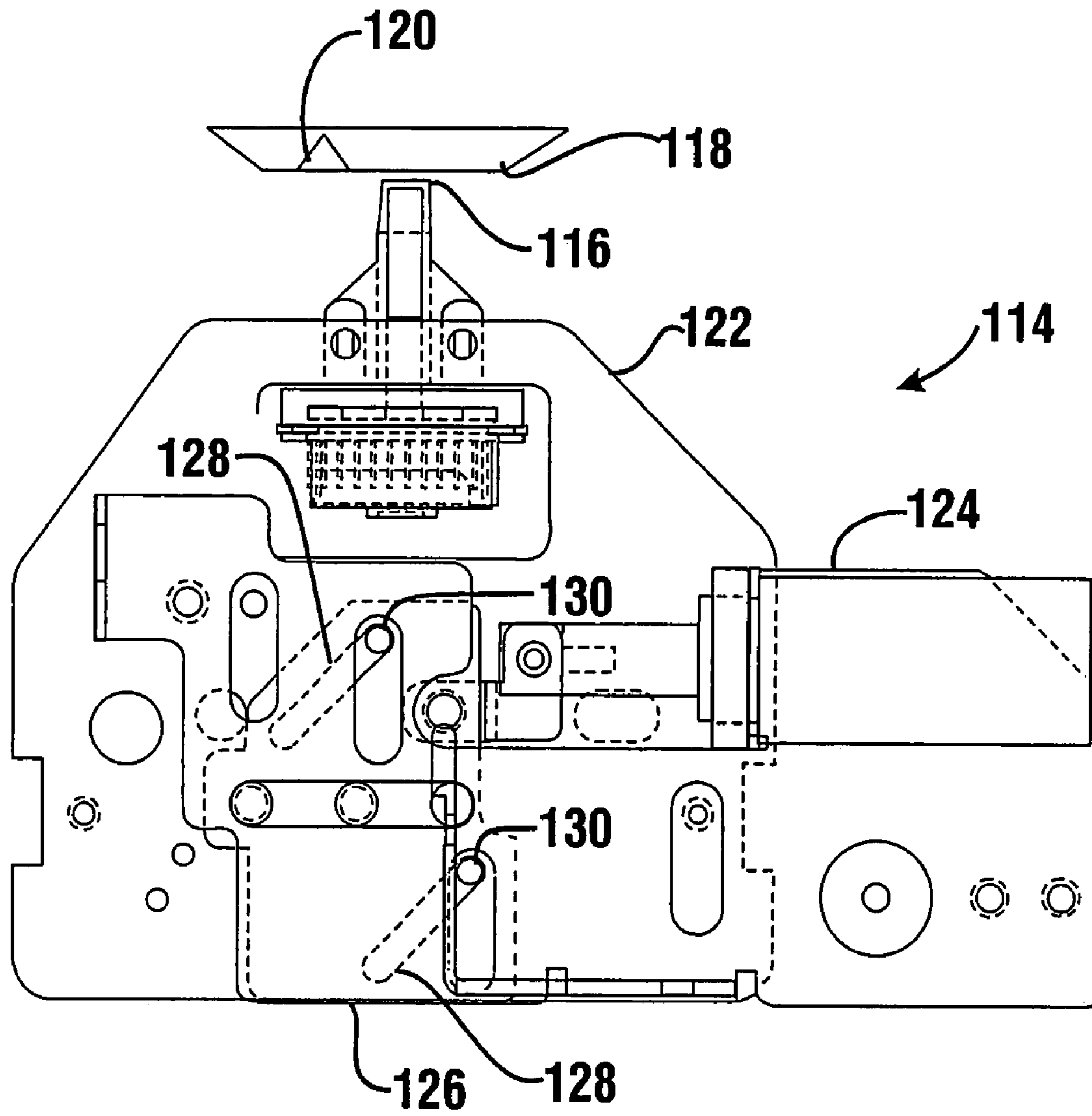
Printing Position
