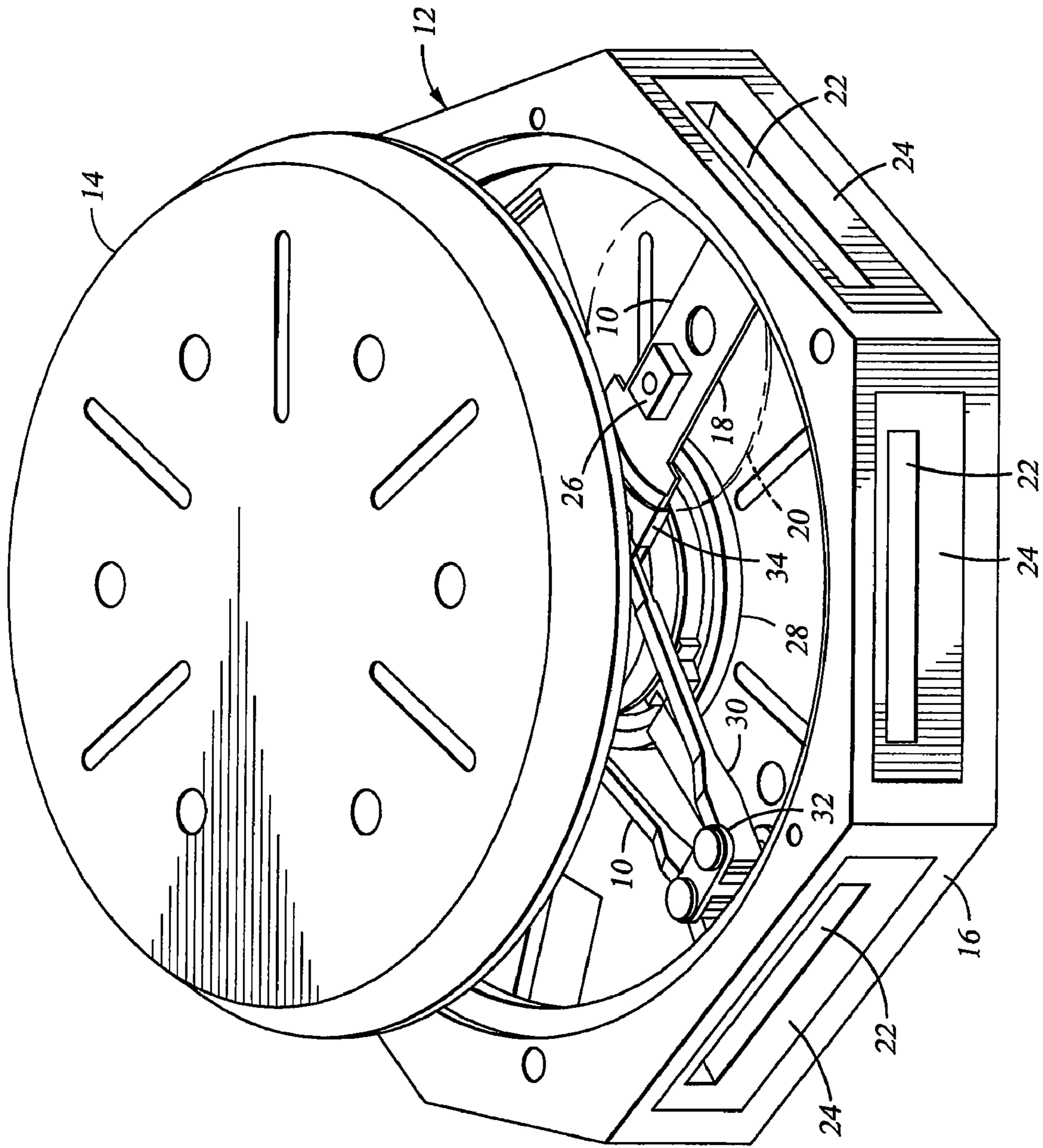
Fig. 1 (PRIOR ART)
