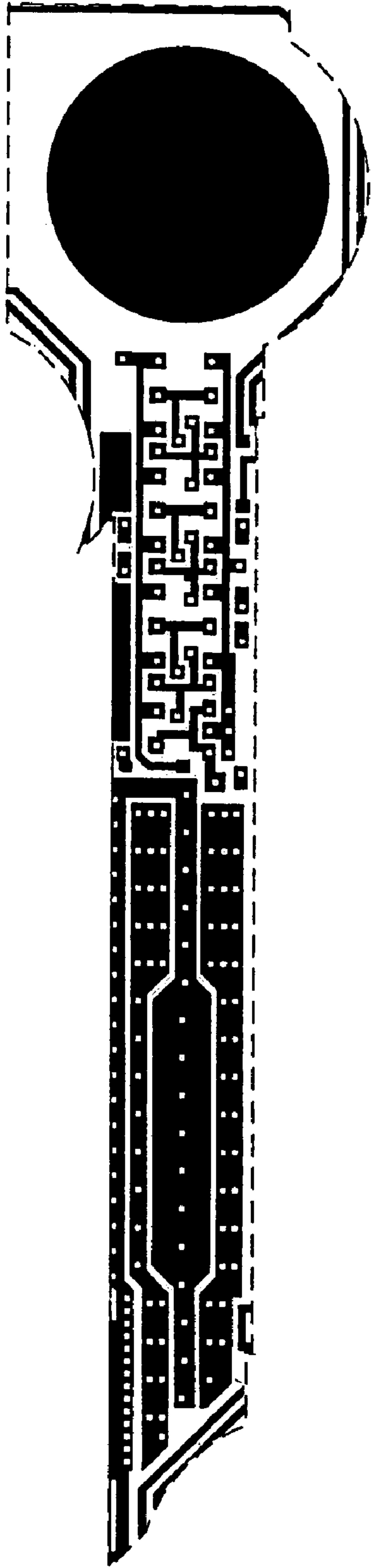
Metal 1 mask
