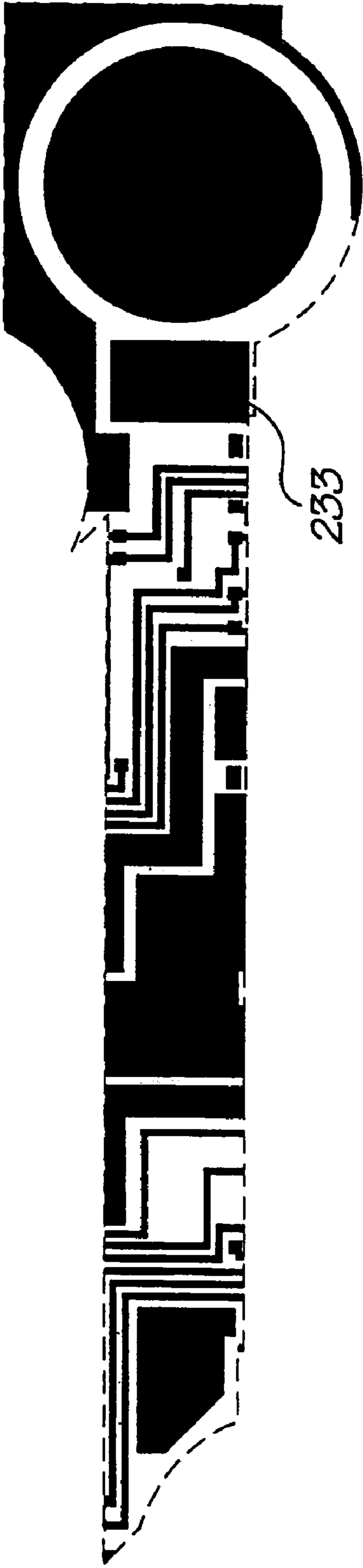
Metal 2 mask
